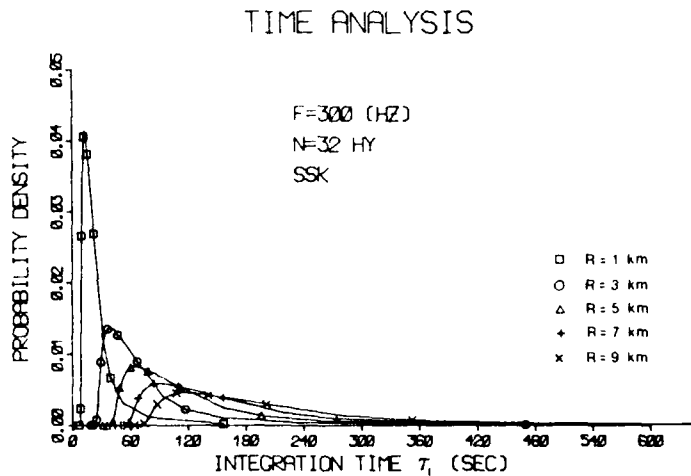
Fig. 6. Time domain analysis: probability density function of integration time ( \tau_i ) for a conventional submarine target.
