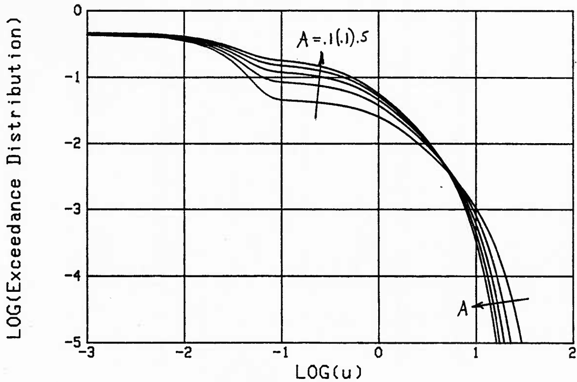
Figure 4.12 Exceedance Distribution Function for \alpha_0 = .25 , \Gamma = 1E-3
