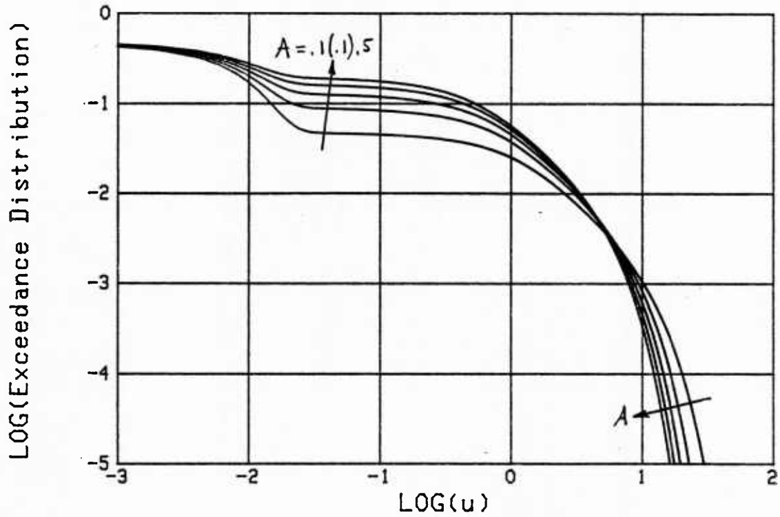
Figure 4.11 Exceedance Distribution Function for \alpha_0 = .25 , \Gamma = 1E-4
