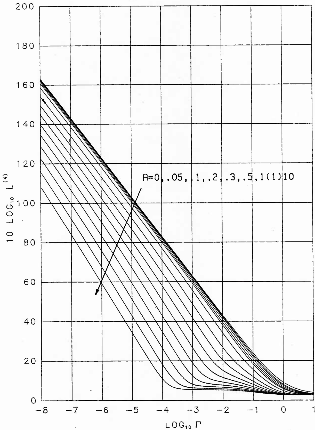
FIGURE 5.2 L^{(4)} IN DB FOR \alpha_0 = .25
