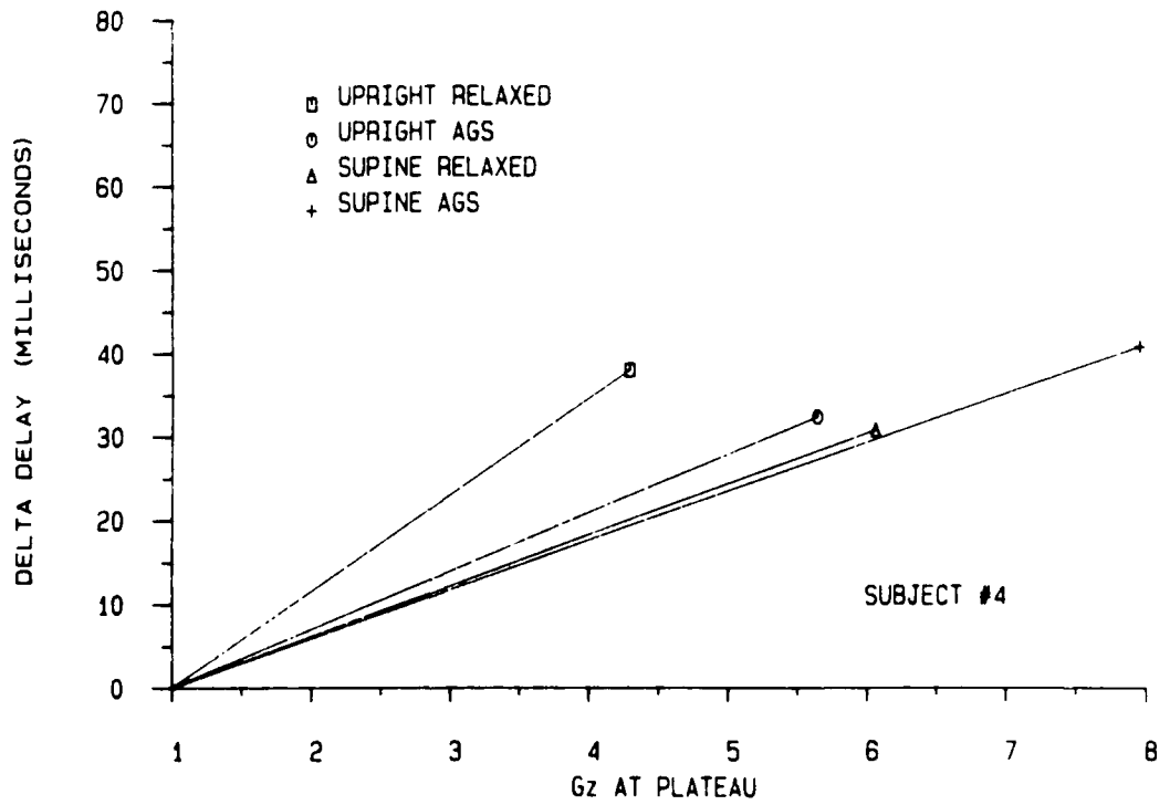
FIGURE 5 - Delta Delay as a Function of Gz with Light-Bar End Points
