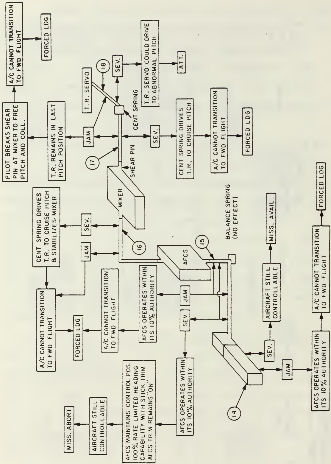
Figure 3.5 Example Disablement Diagram
