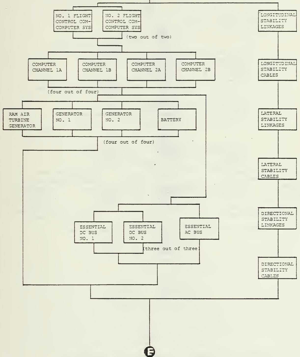
Figure 7.9 (cont.) A-20 Kill Tree Diagram
