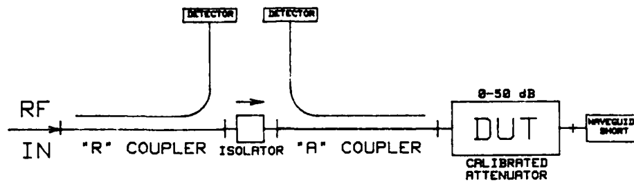
Figure 10. Calibrated Return Loss Setup.
