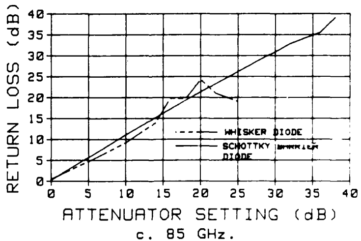
Figure 18. Dynamic Range for Return Loss.
