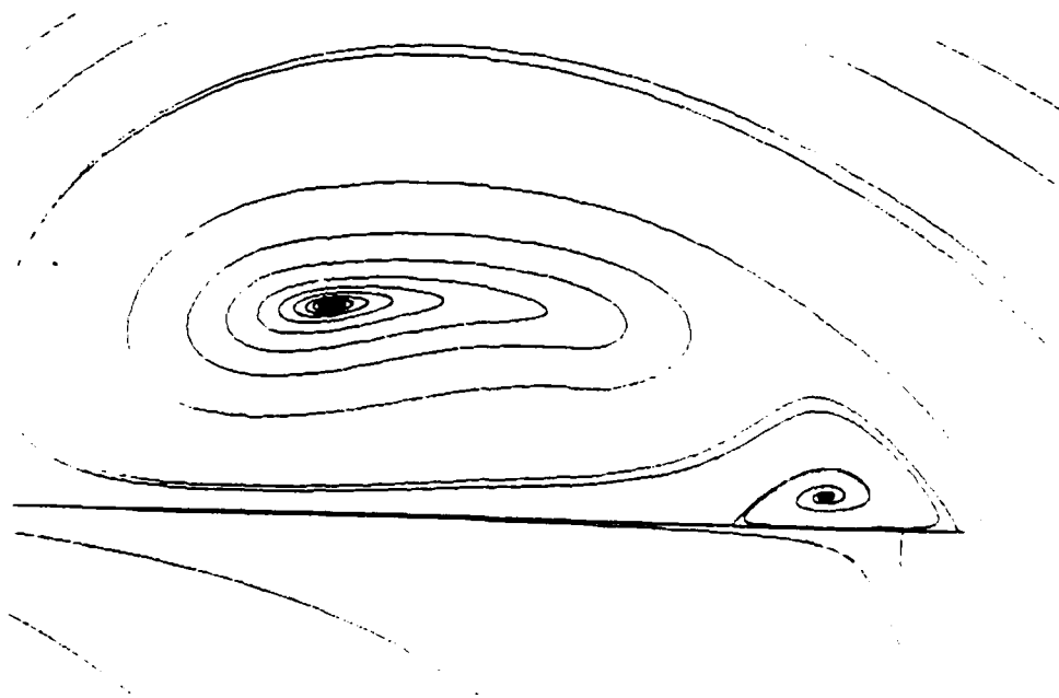
Fig. 12 (a) Flat Plate Delta, 75^\circ Sweep, M_\infty = 1.95 , \alpha = 10^\circ , Surface Pressure Comparison
