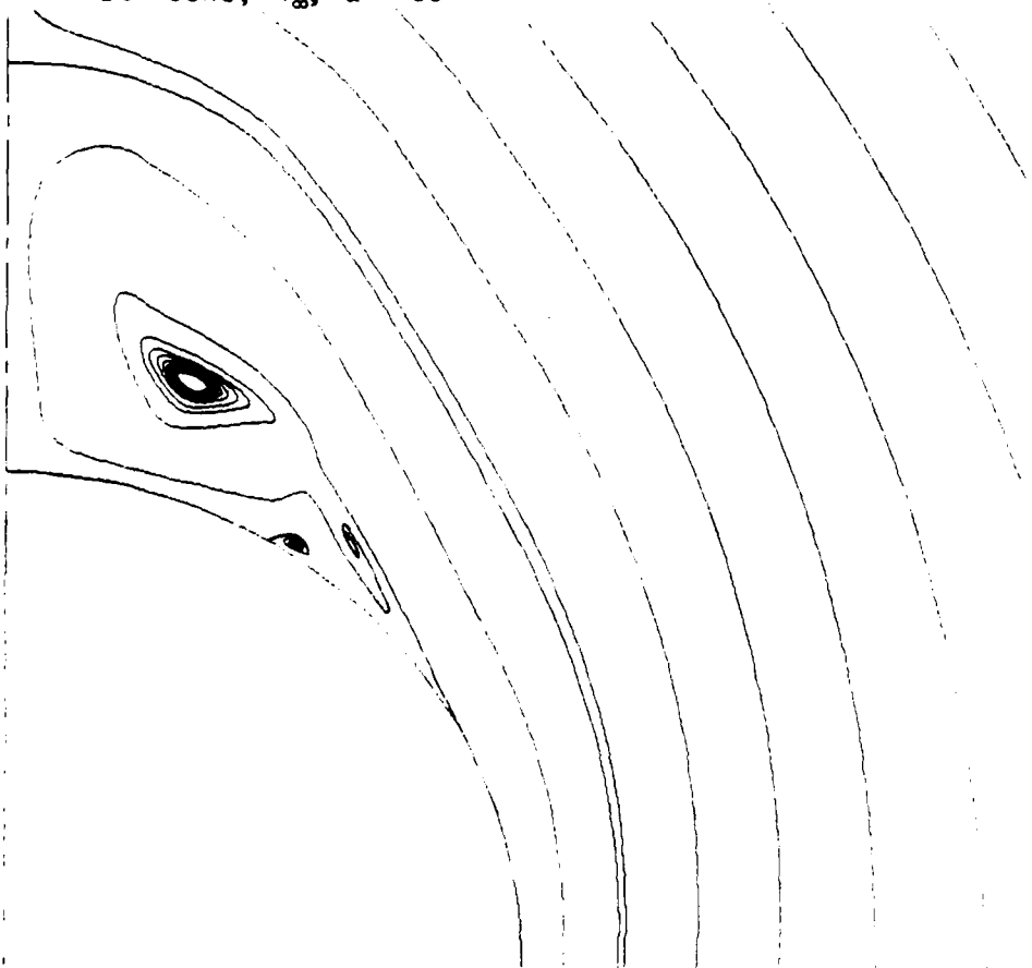
Fig. 11 (b) Crossflow Streamline
