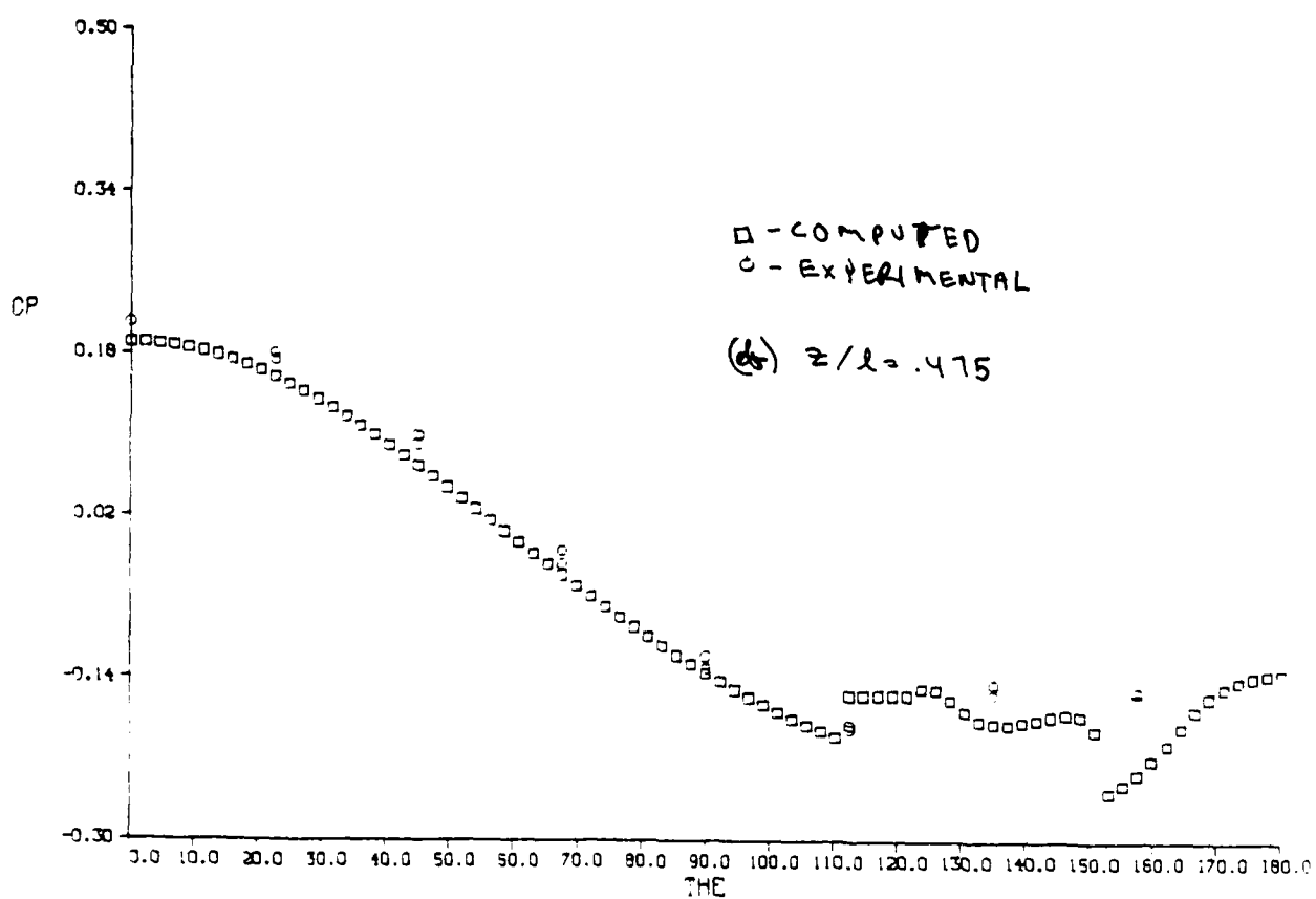
Fig. 10 3-D Cone/Cylinder, Half Angle \delta = 10^\circ , M_\infty = 2.3 , \alpha = 20^\circ , Surface Pressure Distribution
