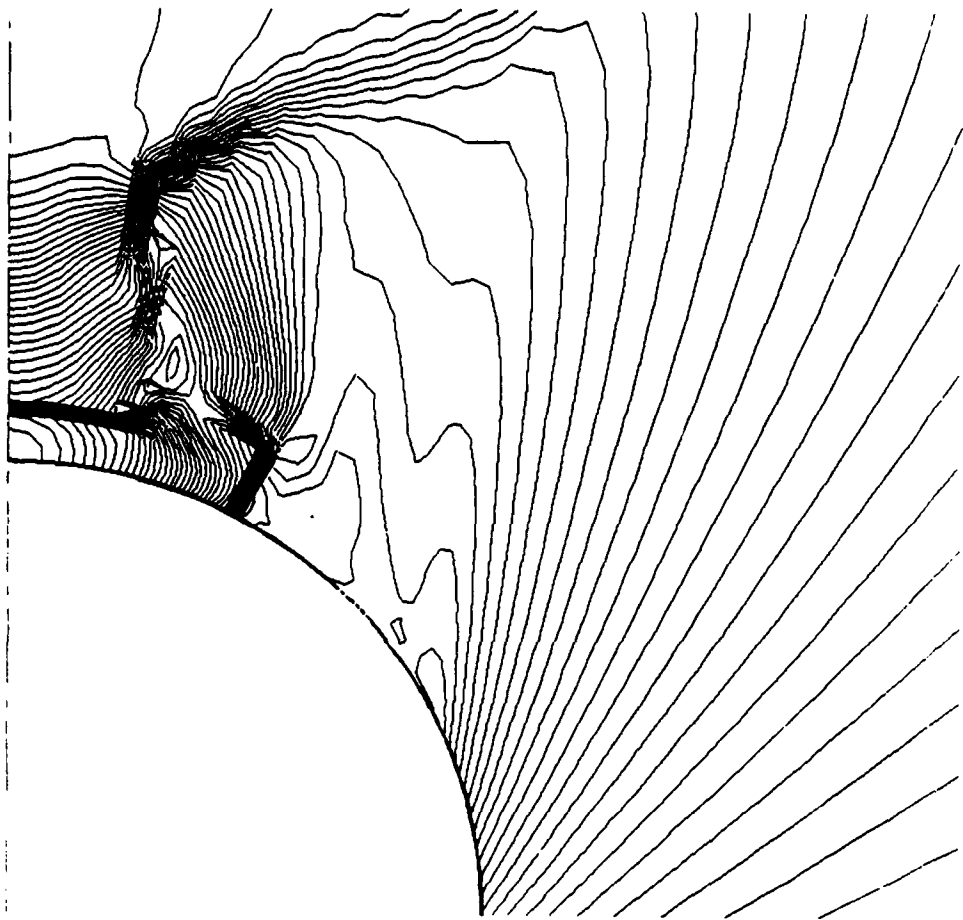
Fig. 11 (a) Isobars, Pin Wheel Shock Pattern 10° Cone, M_\infty , \alpha = 36^\circ
