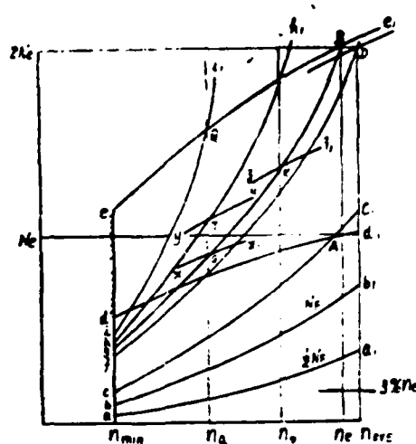
Fig. 3. Operational characteristics of double-engine coupled axles and propeller-fan joint motion.
