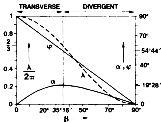
Fig. 3c - The Waterline-Tangent Angle \varphi , the Angle From the Ship Track \alpha and the Wavelength \lambda as Functions of the Wave-Propagation Angle \beta .
