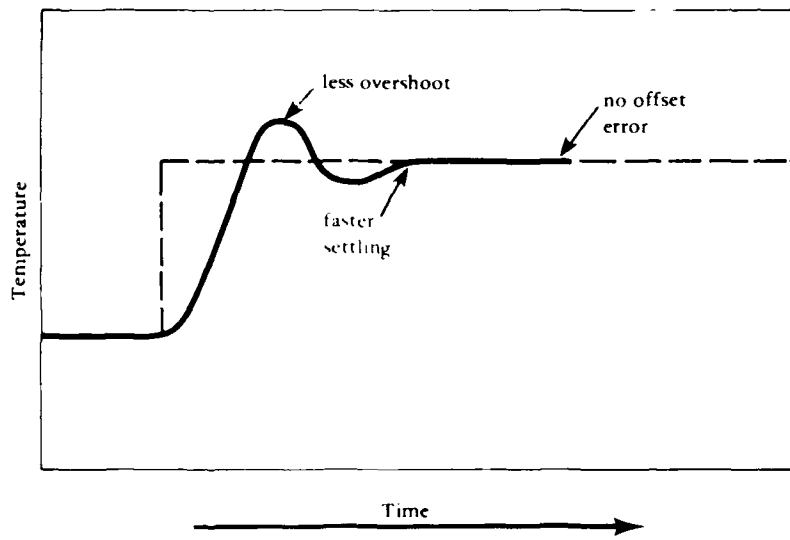
Figure 10. Proportional/integral/derivative control.
