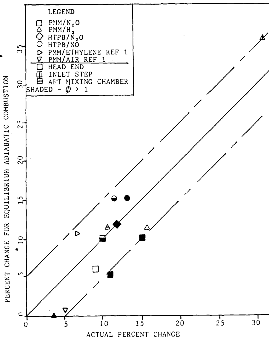
Figure 10. Percent Change in Chamber Pressure; Actual vs Equilibrium Adiabatic Combustion.
