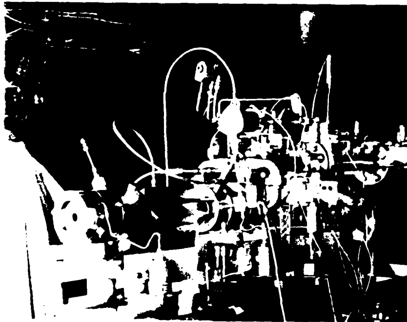
Figure 6. Experimental Thrust Stand and SFRJ.
