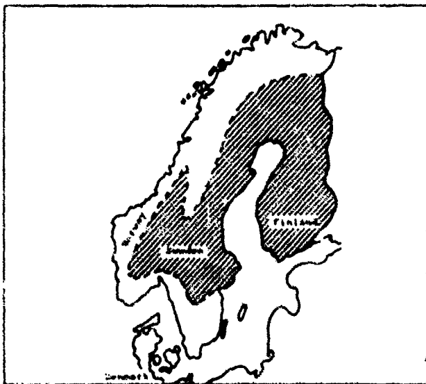
Figure 3-7. Eastern Scandinavian Region (Ref. 19)
