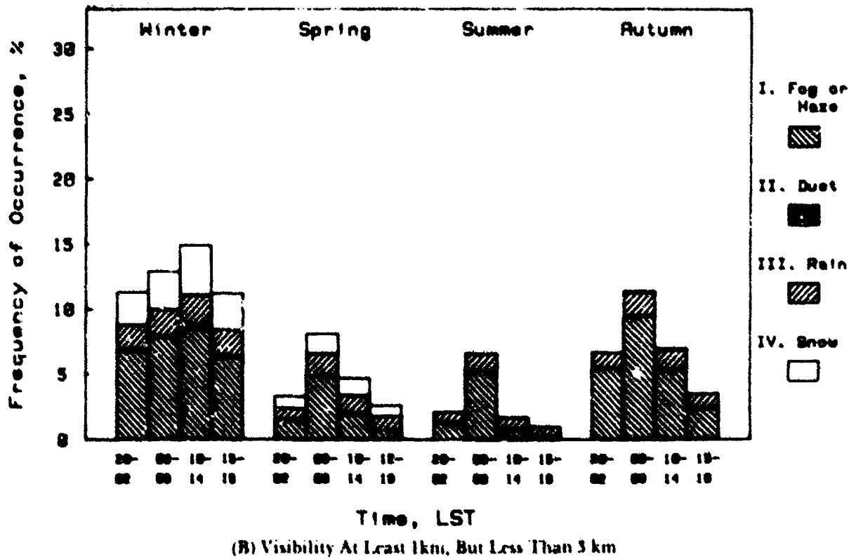
Figure 3-8. European Highlands, Frequency of Natural Obscuration
