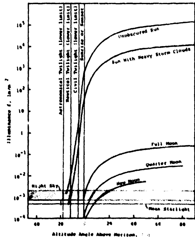
Figure 3-1. Light Level Under Various Atmospheric Conditions
