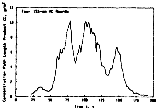
Figure 4-3. Integrated HC Smoke Concentration vs Time (Ref. 7)
