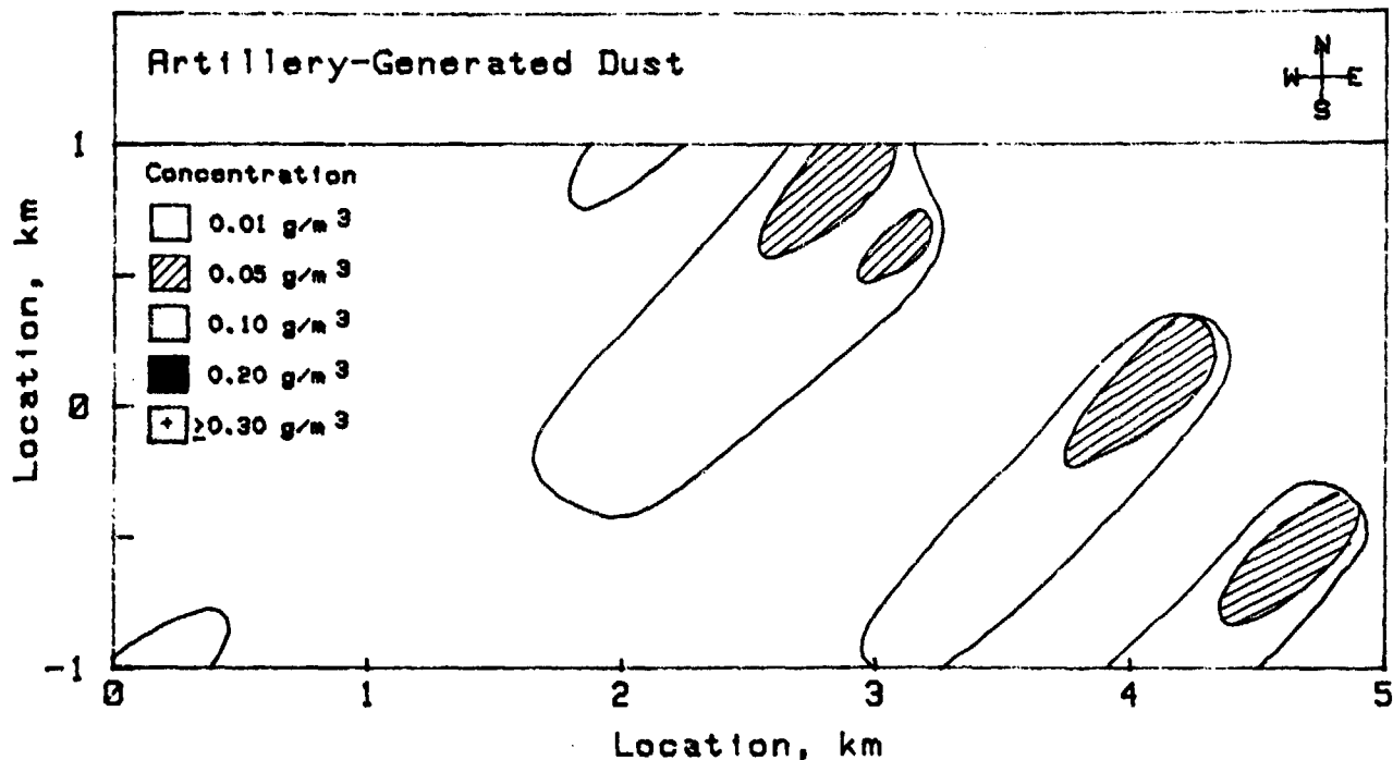
Figure 4-13. Concentration of HE-Generated Dust at 2-m Altitude After Twenty-Fifth Volley (Ref. 15)
