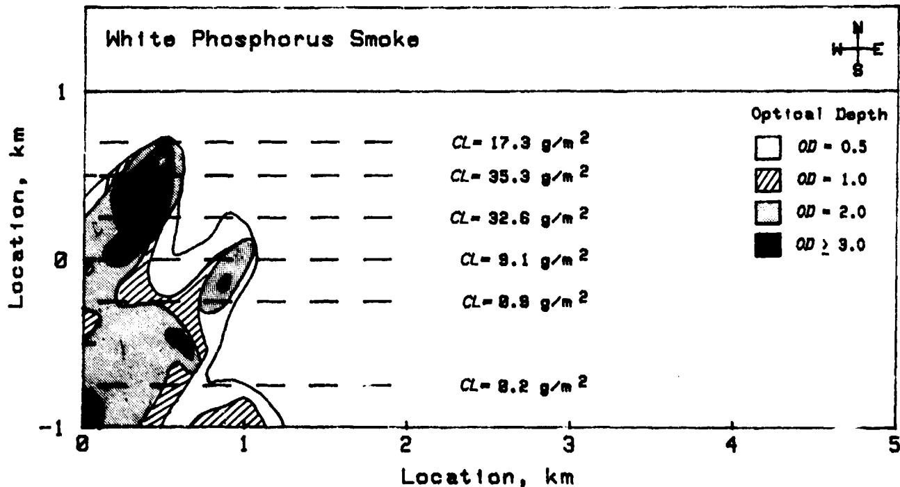
Figure 4-17. Downward-Looking Optical Depth of Phosphorus Smoke at Time H+4 Min (Ref. 15)
