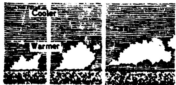
(C) Lapse Conditions
