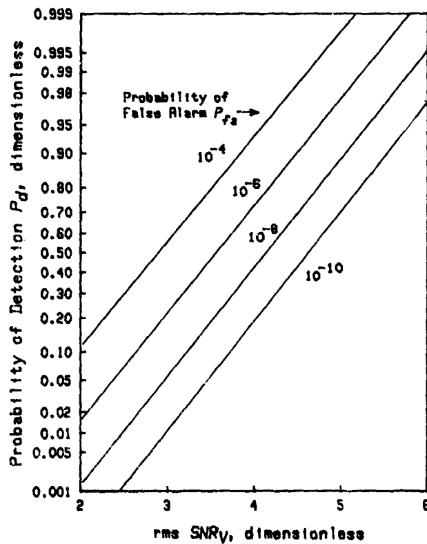
Figure 5-7. Probability of Detection vs rms Voltage SNR (Ref. 4)
