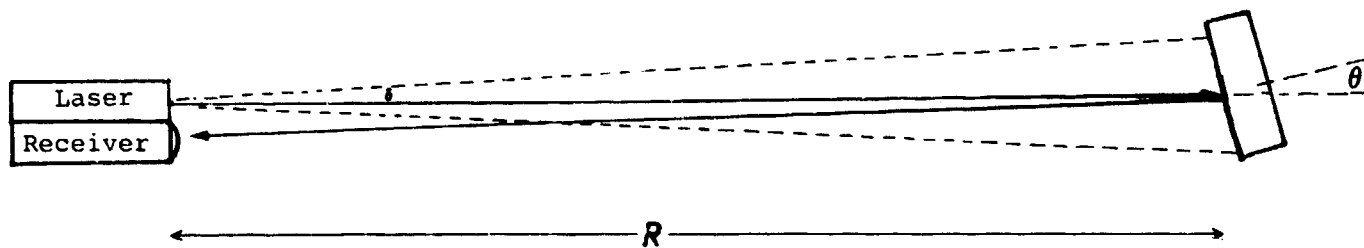
Figure 5-11. Laser Range Finder Geometry
