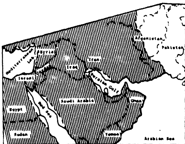
Figure 3-6. Mideast Desert Region (Ref. 3)
