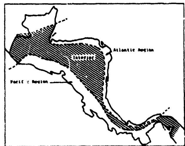
Figure 3-5. Central American Region (Ref. 19)
