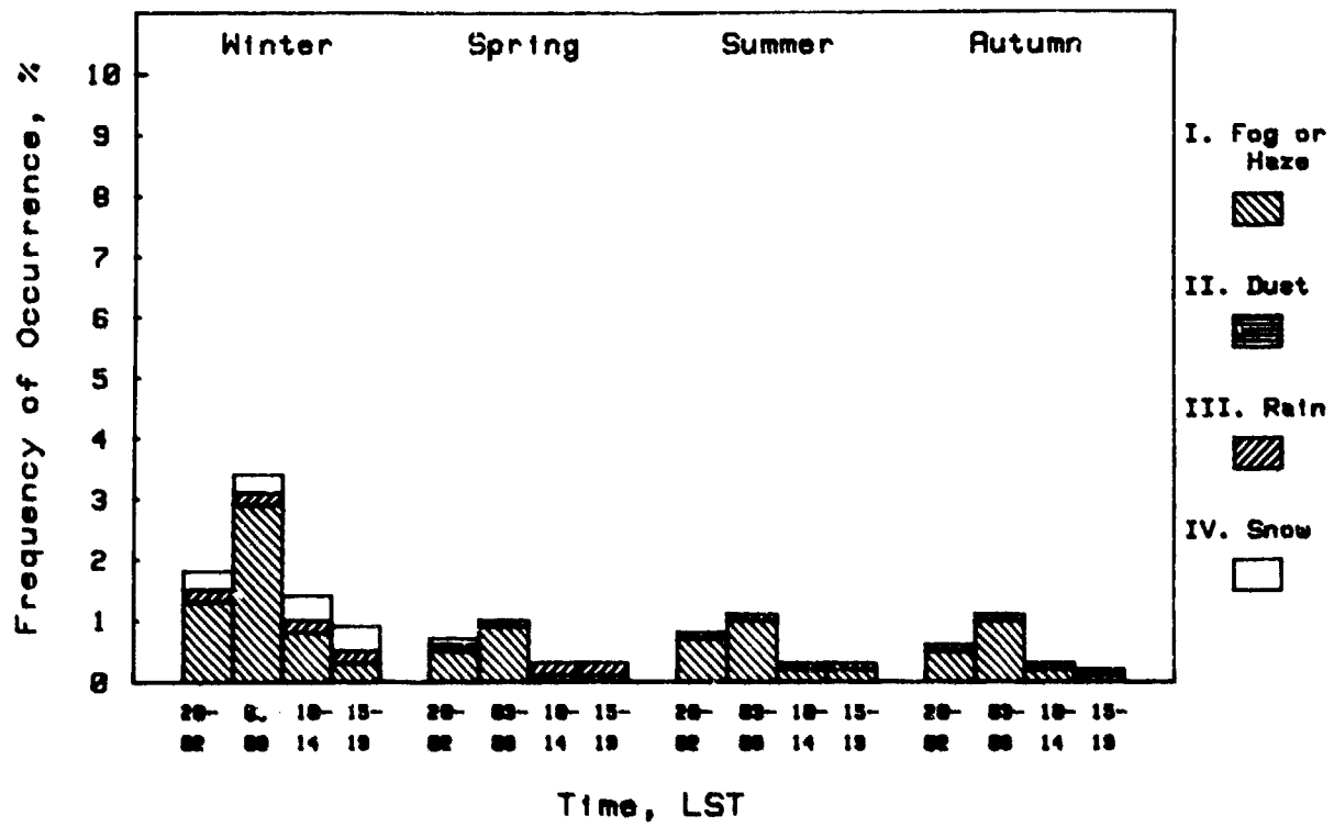
(A) Visibility Less Than 1 km
