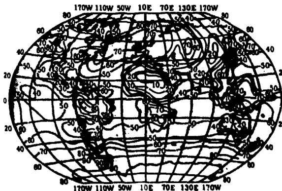
Figure 3-3. Mean Cloudiness in Percentage of Sky Cover, January (Ref. 17)
