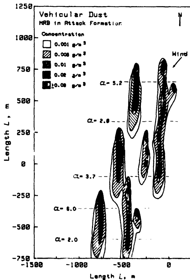
Figure 4-24. Concentration of Dust at a 2-m Altitude from Motorized Rifle Battalion in Attack Formation
