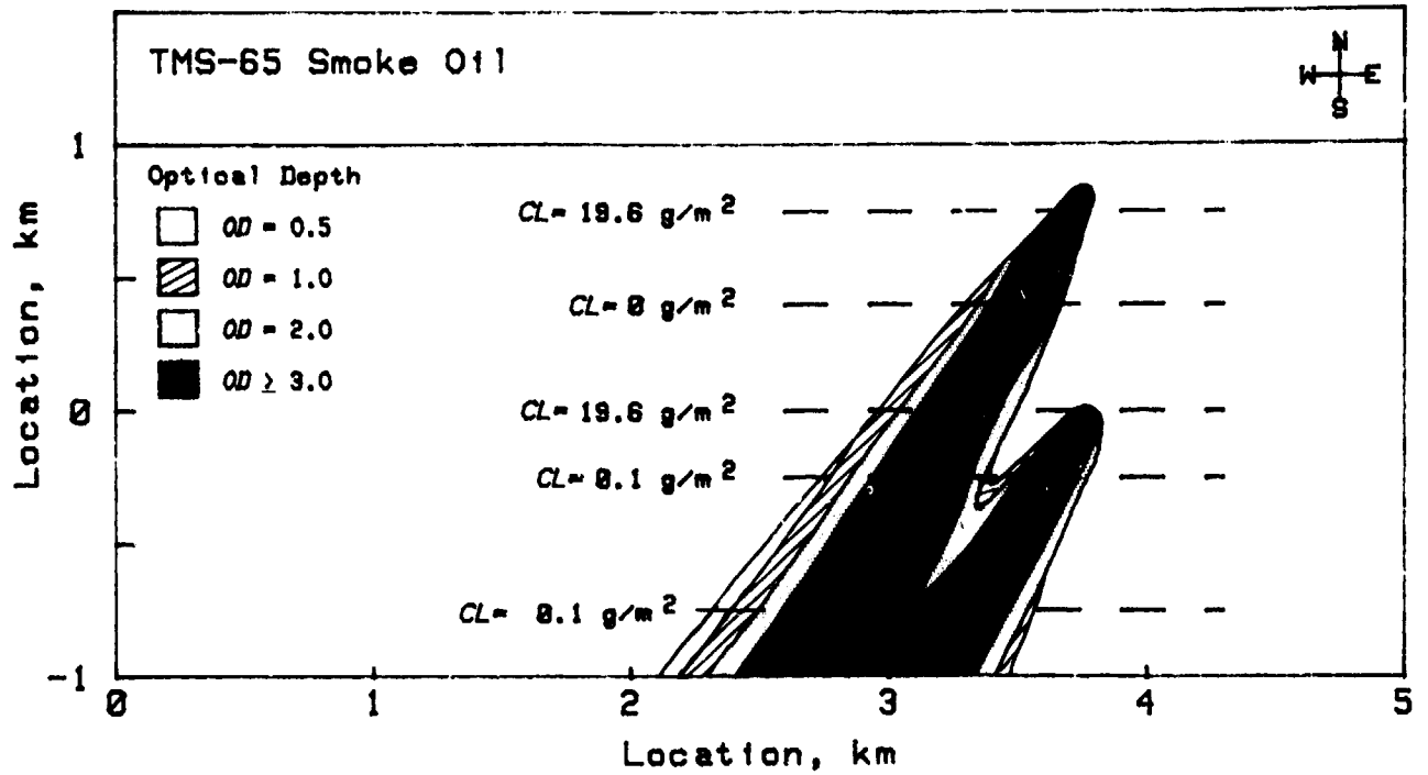
Figure 4-15. Downward-Looking Optical Depth of TMS Smoke at Time H-9 Min (Ref. 15)
