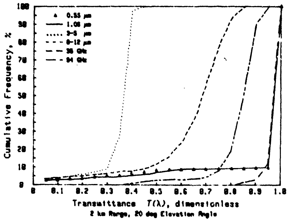
(B) Efsahan, Iran, 1500 Hours
