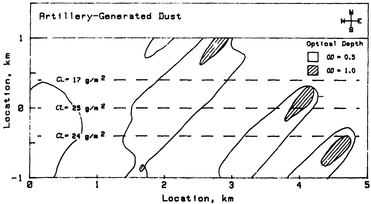
Figure 4-12. Downward-Looking Optical Depth of HE-Generated Dust After Twenty-Fifth Volley (Ref. 15)
