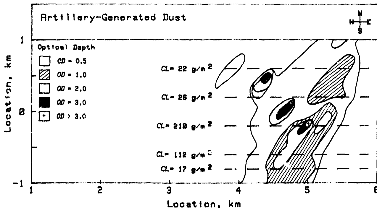
Figure 4-10. Downward-Looking Optical Depth of HE-Generated Dust After Fifth Volley (Ref. 15)
