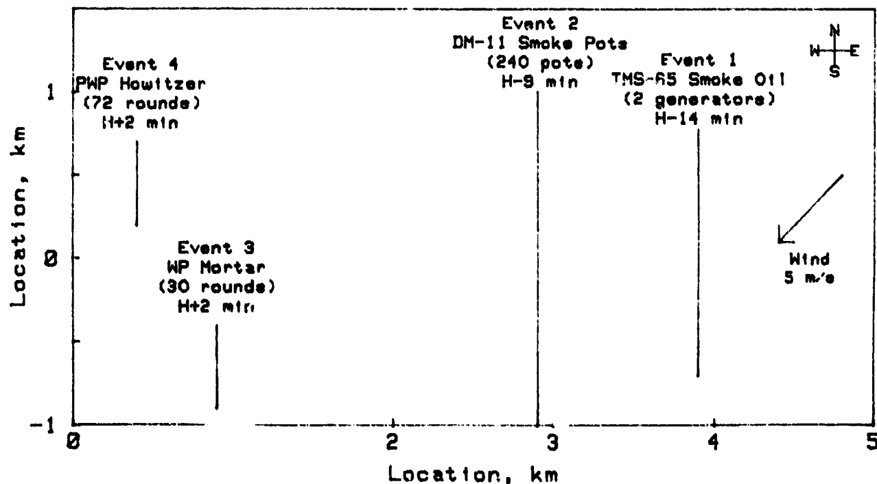
Figure 4-14. Smoke Example Overview
