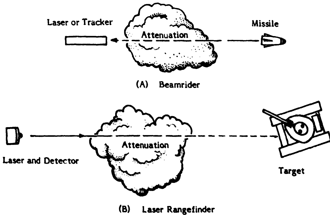
Figure 2-4. Direct View Geometries (Ref. 5)
