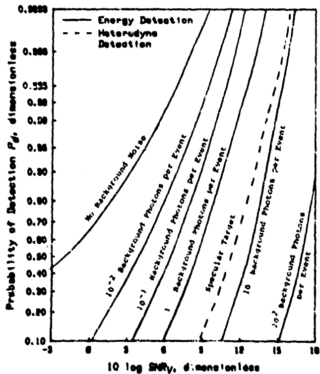
Figure 5-8. Probabilities of Detection for Active Systems With a Specular or Well-Resolved Rough Target (Ref. 4)
