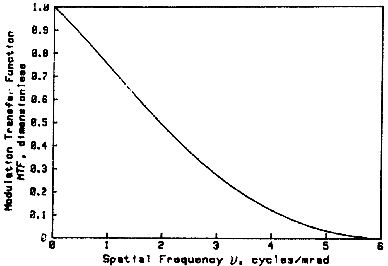
Figure 5-1. Modulation Transfer Function vs Spatial Frequency
