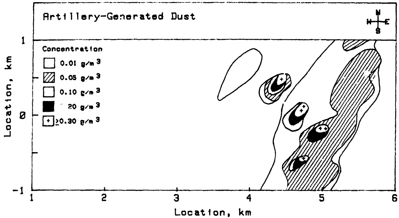
Figure 4-11. Concentration of HE-Generated Dust at 2-m Altitude After Fifth Volley (Ref. 15)
