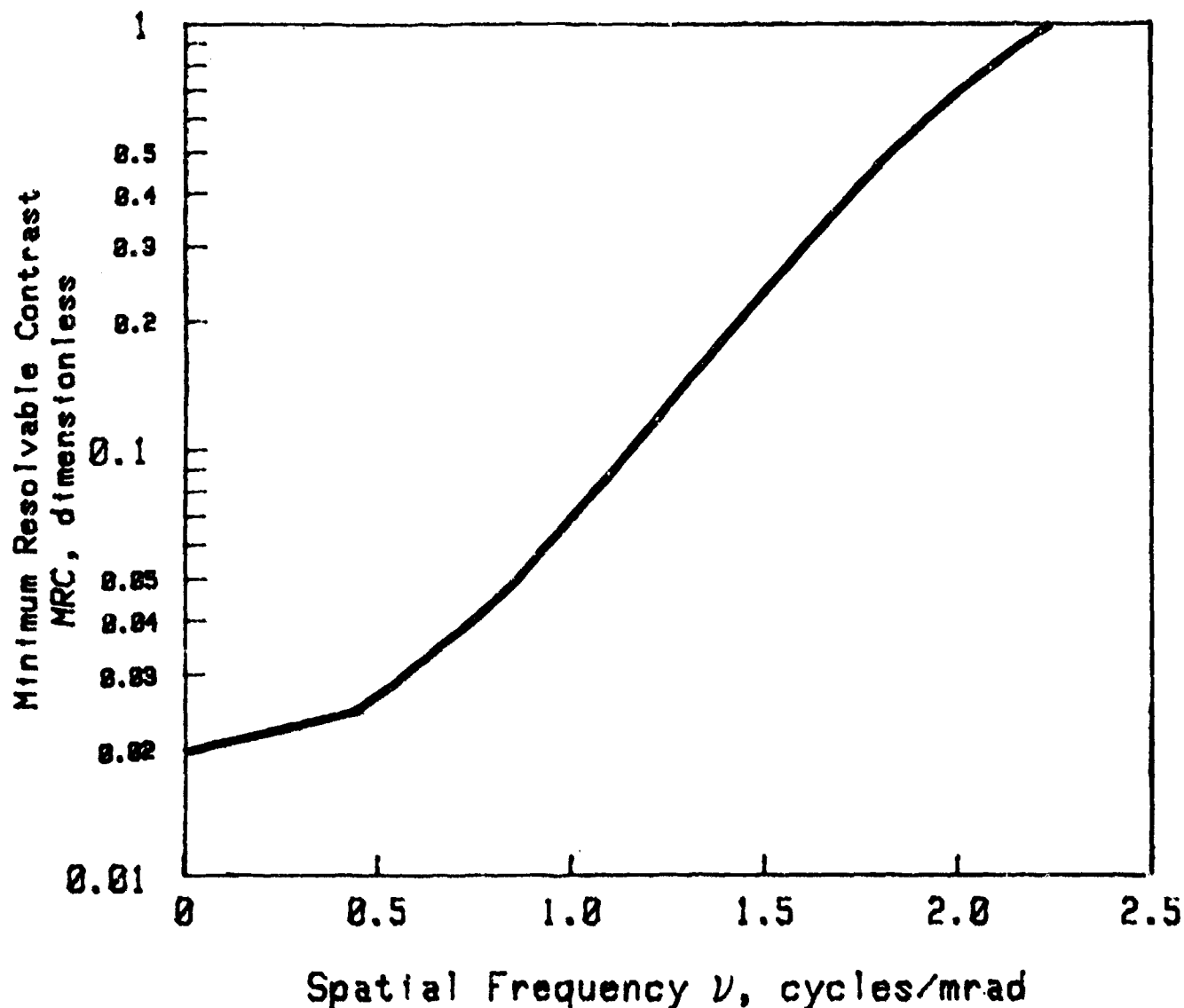
Figure 5-3. Eye MRC Curve, Daylight (Ref. 1)
