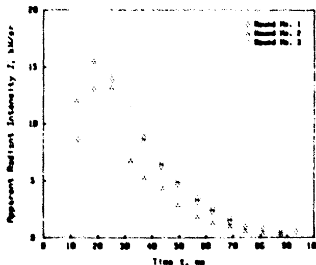
Figure 4-8. Apparent Radiant Intensity of an M-68 105-mm Gun in the 4.35 to 4.70 μm Spectral Band (Ref. 16)
