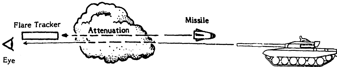
(E) Command Line of Sight Guidance
