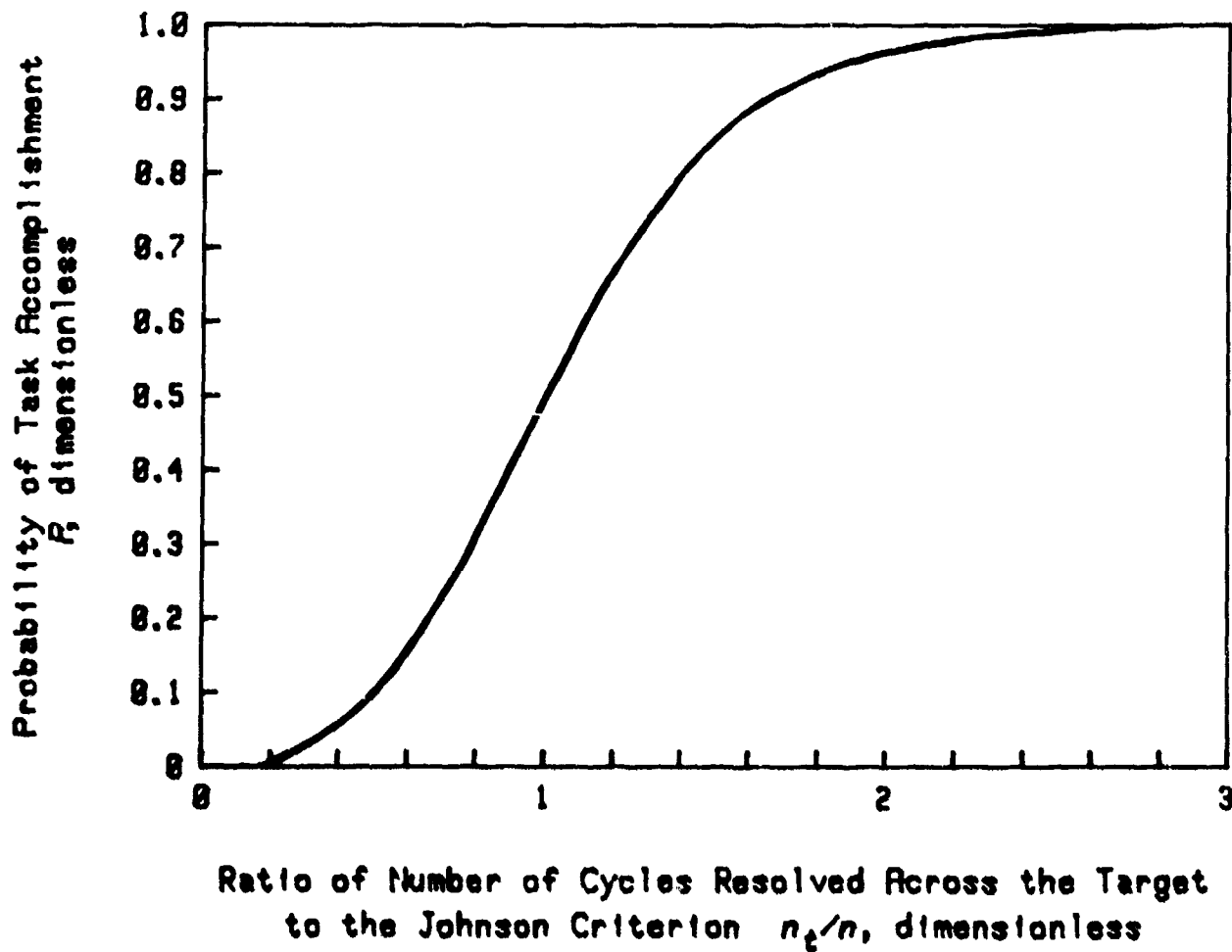
Figure 5-5. Probability vs Resolution Requirement (Ref. 2)
