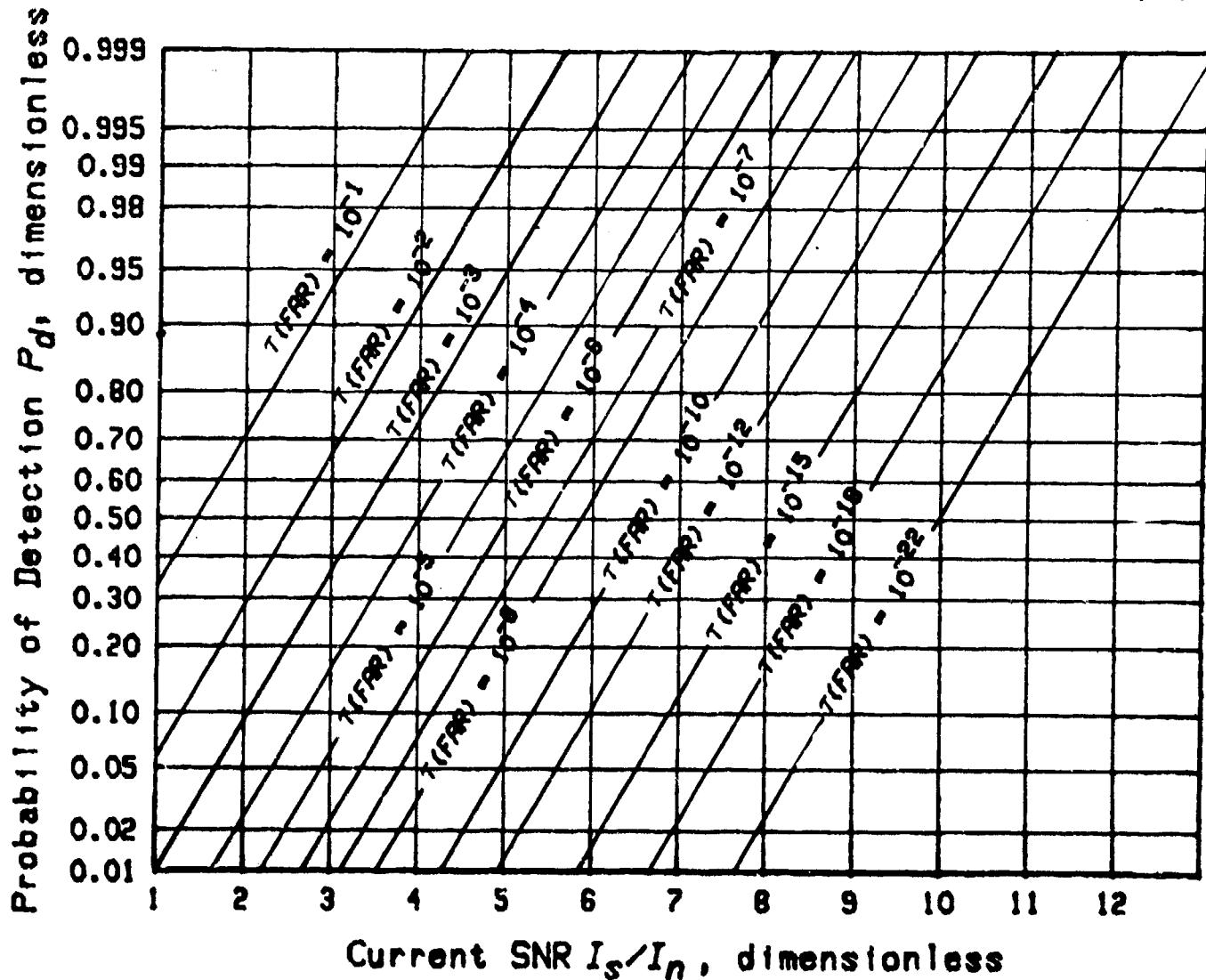
Figure 5-10. Probability of Detection vs Signal-to-Noise Ratio as a Function of False Alarm Rate (Ref. 3)
