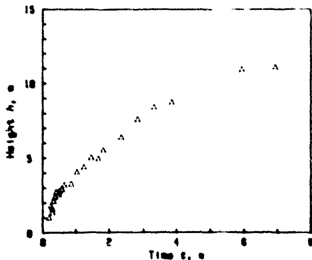
Figure 4-7. HE-Generated Dust Cloud Centroid Height vs Time (Ref. 14)
