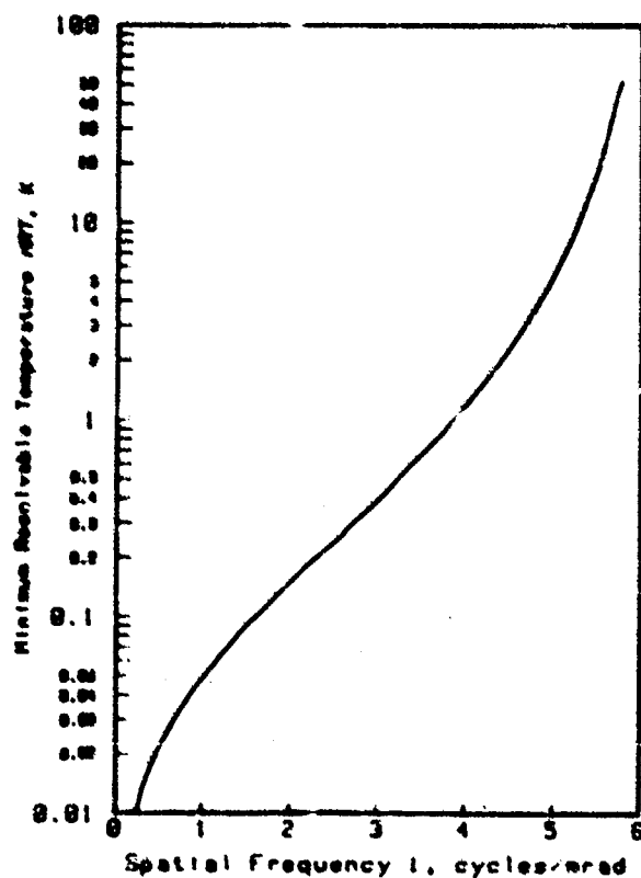
Figure 5-2. Thermal Imager MRT Curve
