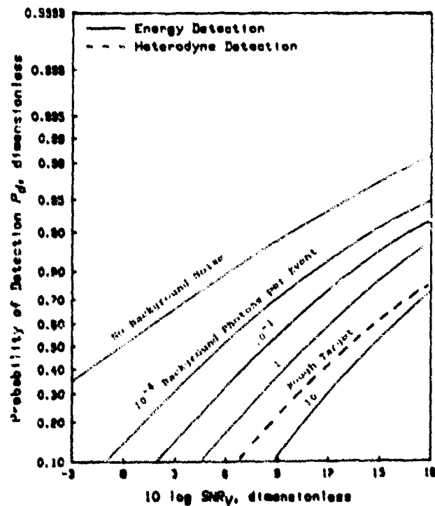
Figure 5-9. Probabilities of Detection for Active Systems With Rough Targets (Ref. 4)
