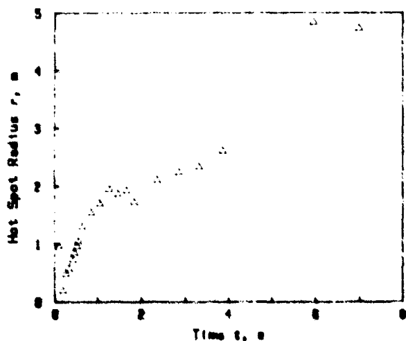
Figure 4-6. HE-Generated Dust Cloud Hot Spot Radius vs Time (Ref. 14)
