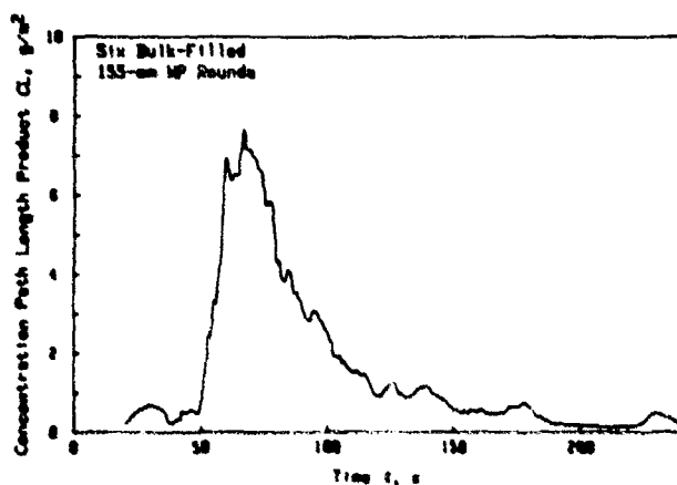
Figure 4-2. Integrated WP Smoke Concentration vs Time (Ref. 7)
