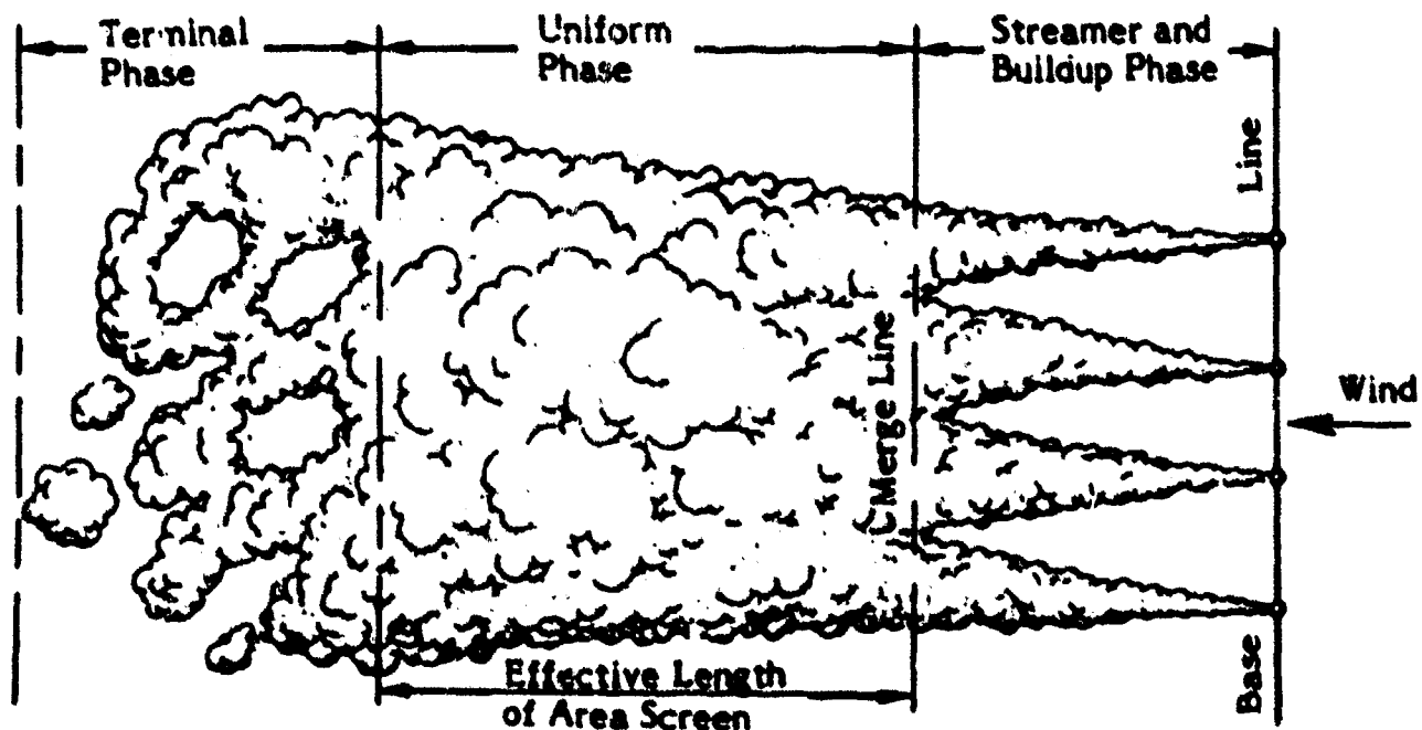
Figure 2-7. Smoke Screen—Effective Length and Smoke Phases (Ref. 5)
