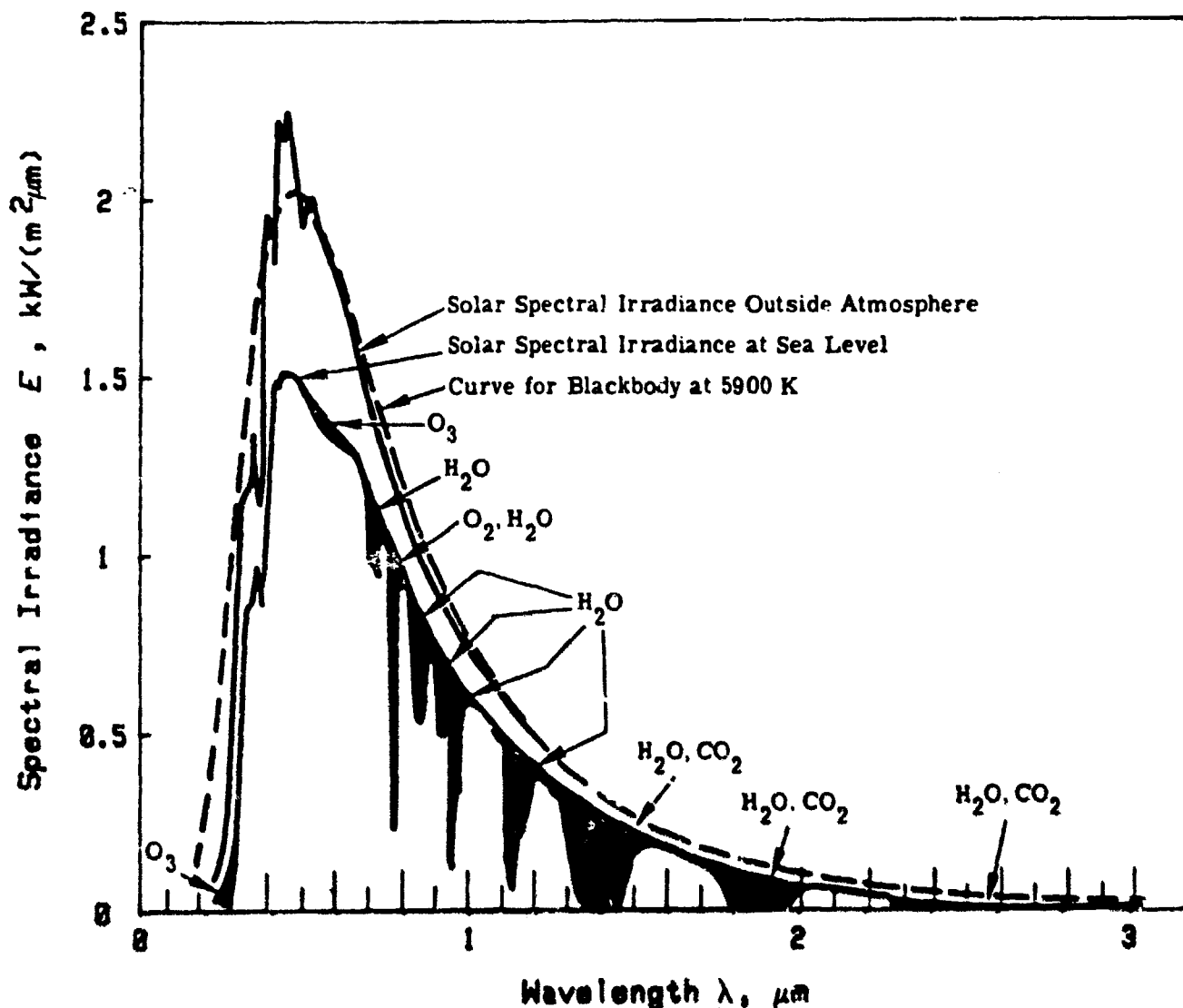
Figure 2-6. Solar Spectrum as Seen Through The Earth's Atmosphere (Ref. 9)
