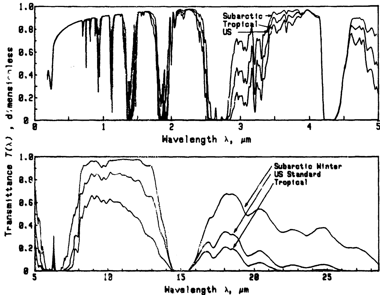
Figure 2-1. Atmospheric Transmittance T(\lambda) vs Wavelength \lambda (Ref. 1)
