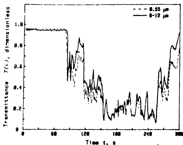
Figure 4-9. Transmittance Through Snow Lofted by Helicopter Downwash (Ref. 20)
