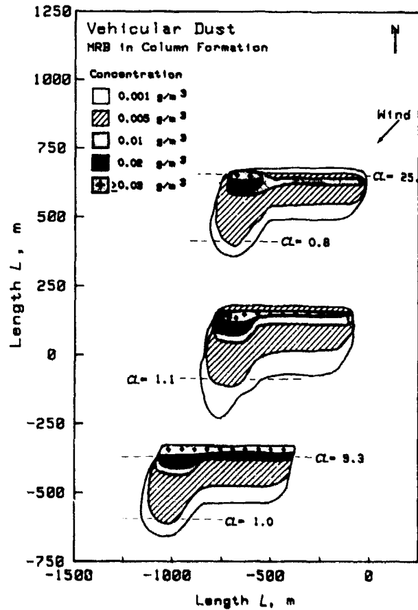
Figure 4-23. Concentration of Dust at a 2-m Altitude from Motorized Rifle Battalion in Column Formation
