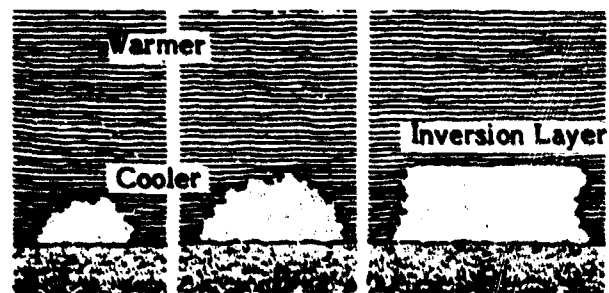
(A) Stable Conditions
