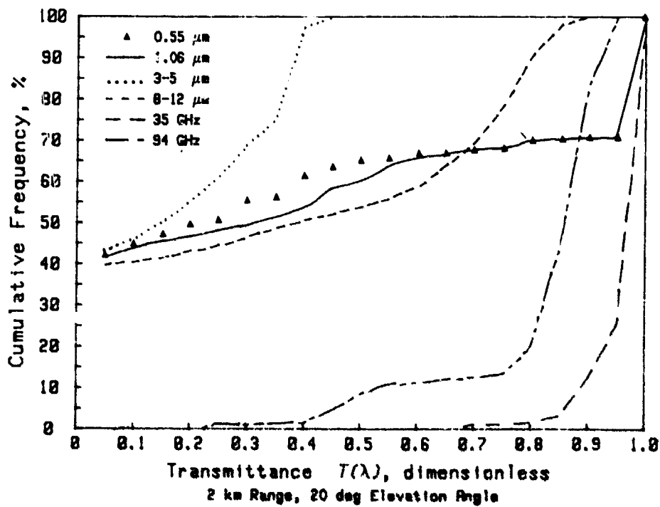
(A) Morning Nautical Twilight
