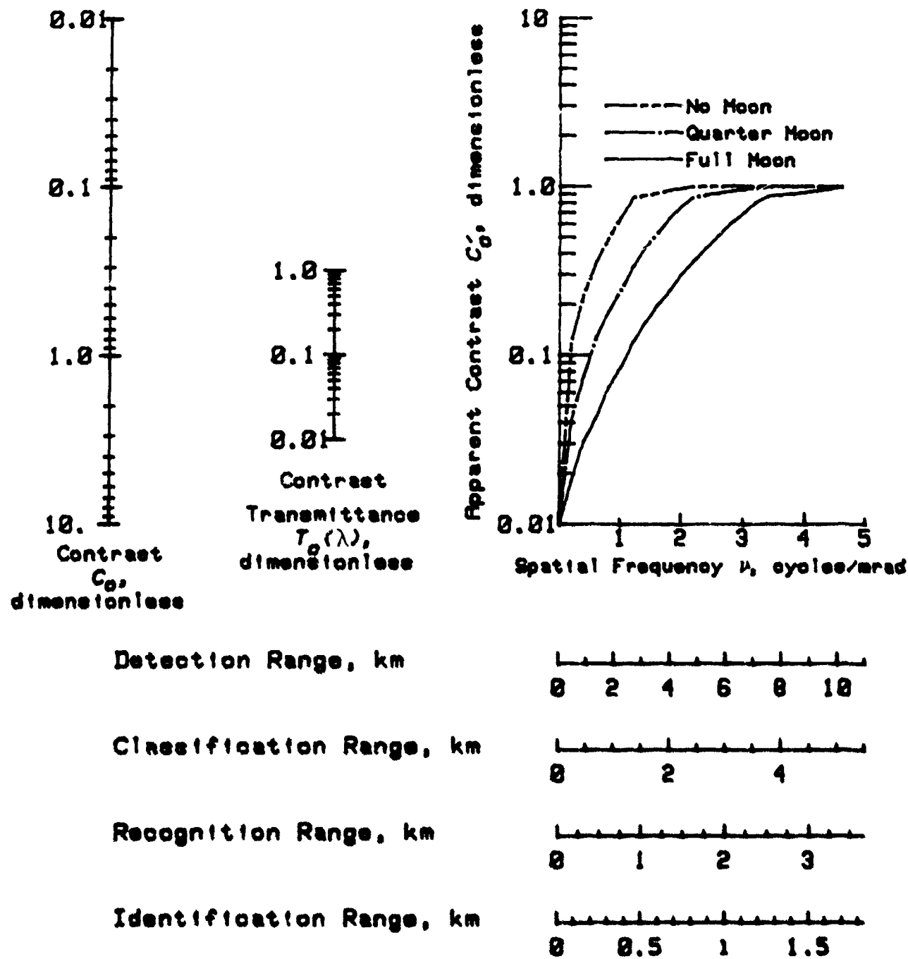
Figure 5-4. Crew Served Weapon Sight Performance Nomogram (Ref. 1)
