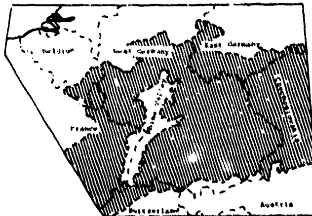
Figure 3-4. European Highlands Region (Ref. 3)
