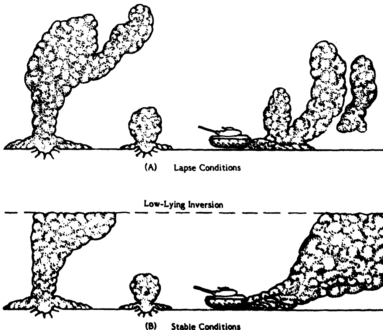
Figure 2-10. Atmospheric Stability Effect on HE-Generated Dust Cloud Development (Ref. 5)
