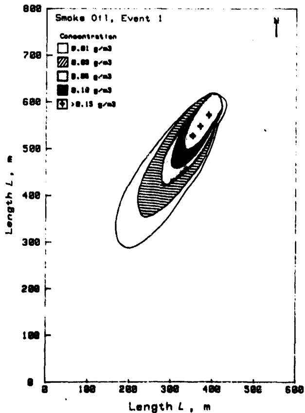
Figure 4-18. Concentration of TMS Oil Smoke at a 2-m Altitude at Time H-9 min (Ref. 15)
