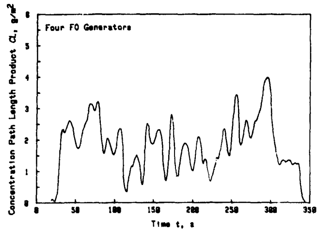
Figure 4-4. Integrated Fog Oil Concentration vs Time (Ref. 7)
