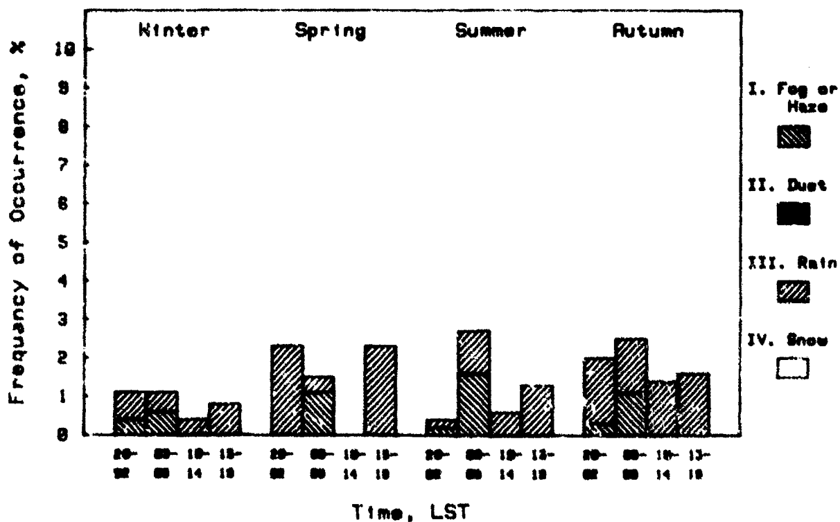
(B) Visibility At Least 1 km, But Less Than 3 km
