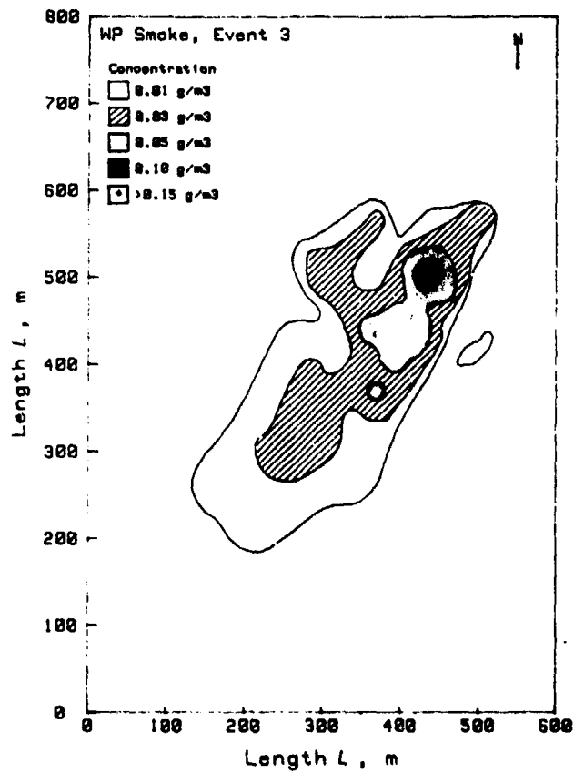
Figure 4-20. Concentration of Phosphorus Smoke from WP Munitions at a 2-m Altitude at Time H+4 Min (Ref. 15)
