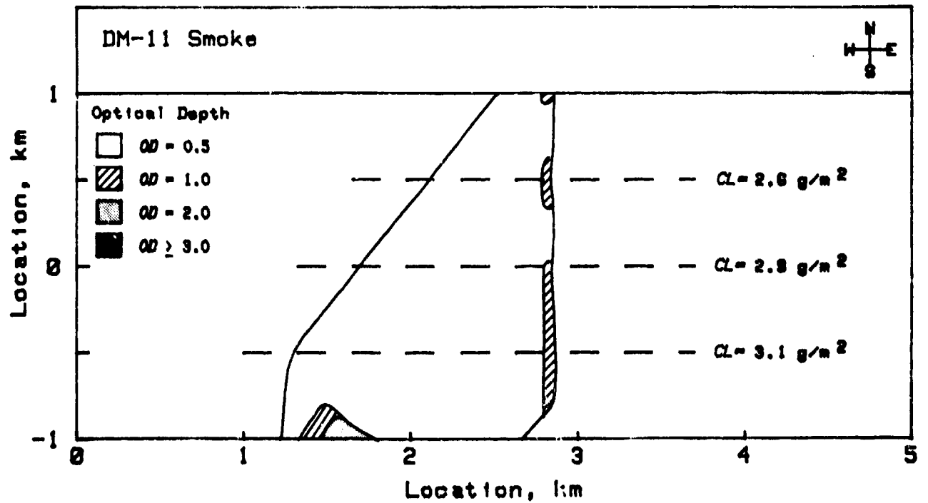
Figure 4-16. Downward-Looking Optical Depth of DM-11 Smoke at Time H-3 Min (Ref. 15)
