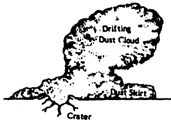
(C) Drift and Dissipation Phase
