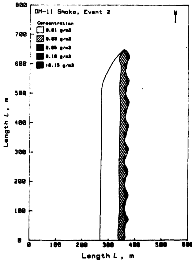
Figure 4-19. Concentration of DM-11 Smoke at a 2-m Altitude at Time H-3 Min (Ref. 15)
