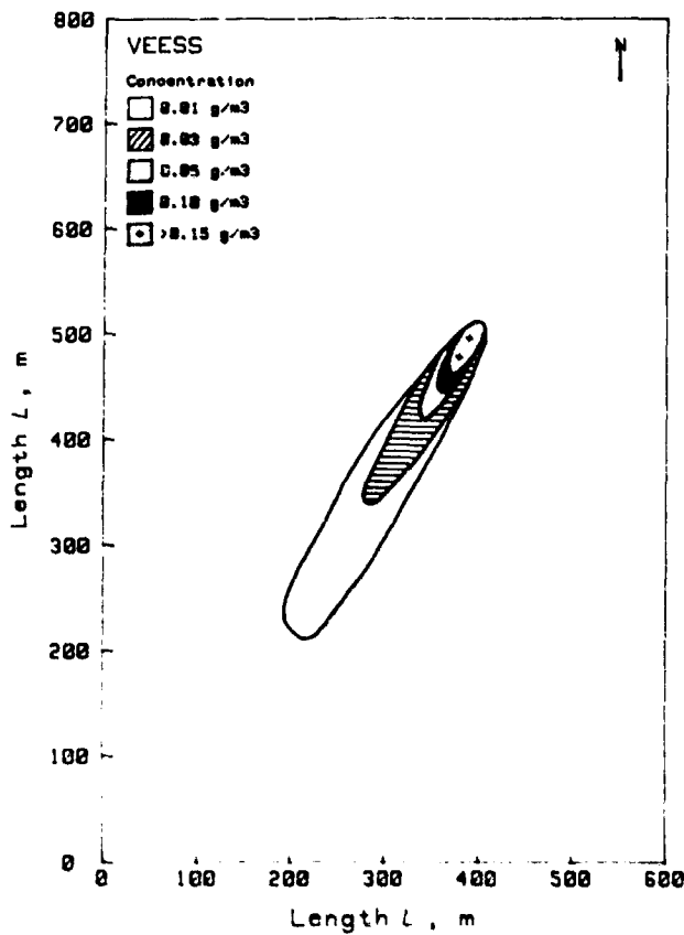
Figure 4-22. Concentration of Smoke from VEES at a 2-m Altitude
