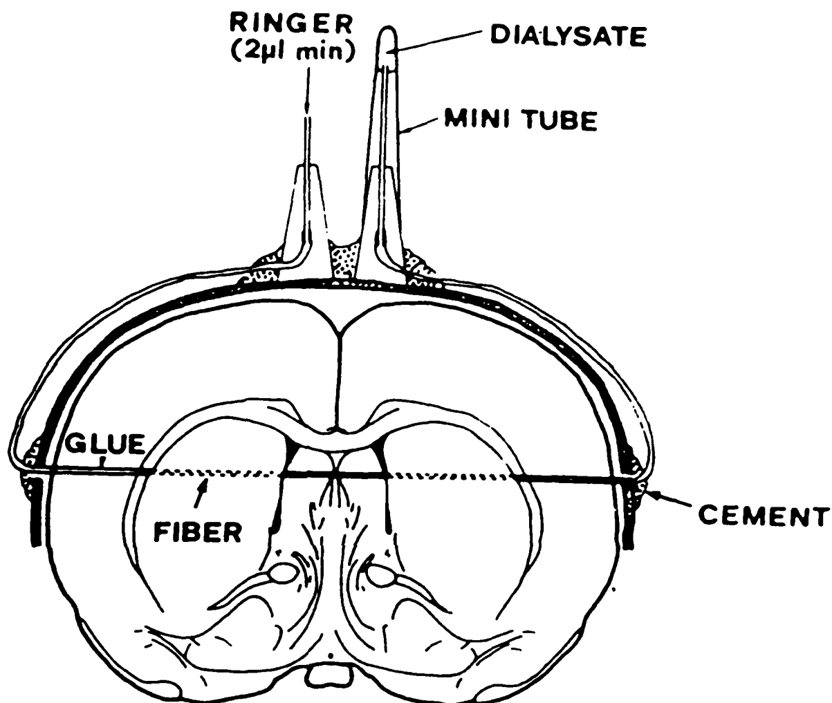
Schematic diagram of a trans-striatal dialysis preparation in an awake rat.
