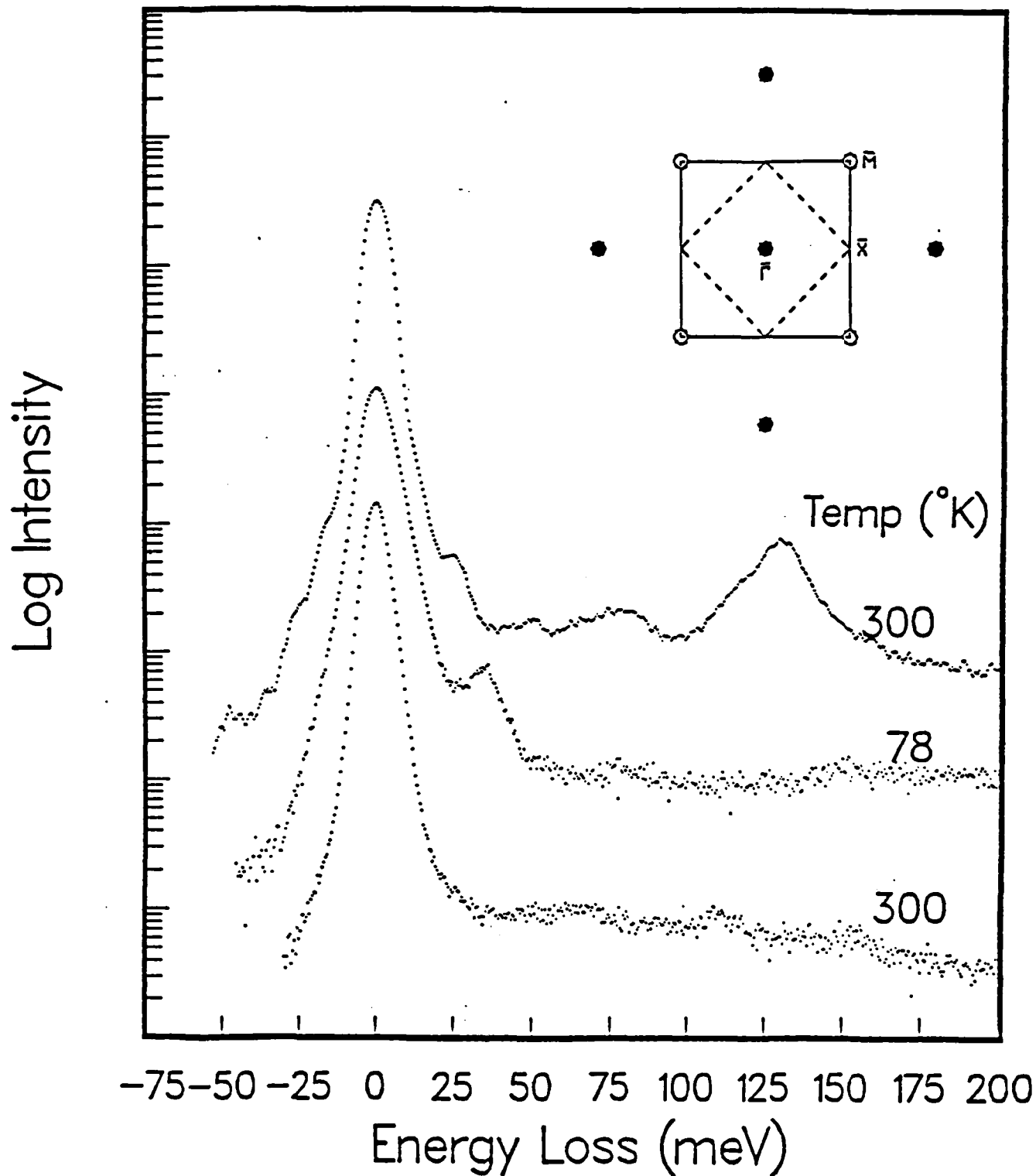
Fig. 1. Specular ( 60^\circ ) EEL spectra for hydrogen saturated surface
