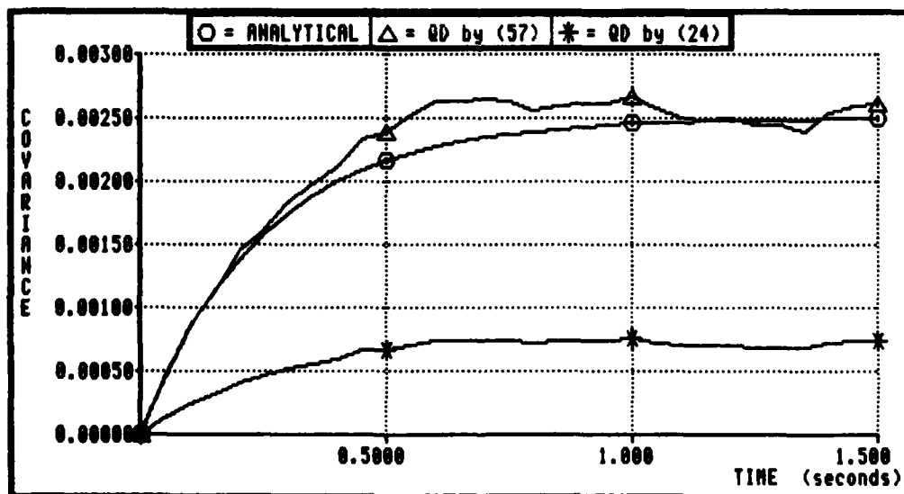
Figure 10. Runge-Kutta (5,6) Analysis
