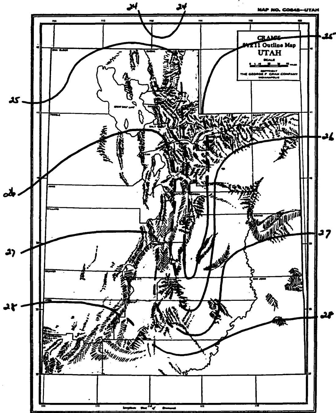
Figure 38. Monthly distribution of irradiance in Utah. Month of May. Units are: MJm^{-2} day^{-1}
