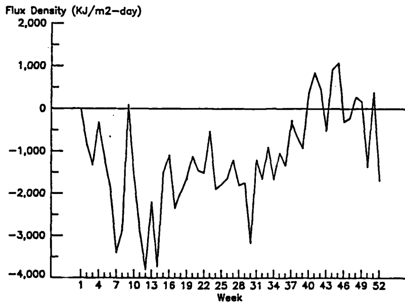
Figure 11. The difference between mean and median daily radiation for each week and month of the year.
