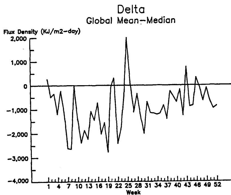
Figure 5. The difference between mean and median daily radiation for each week and month of the year.
