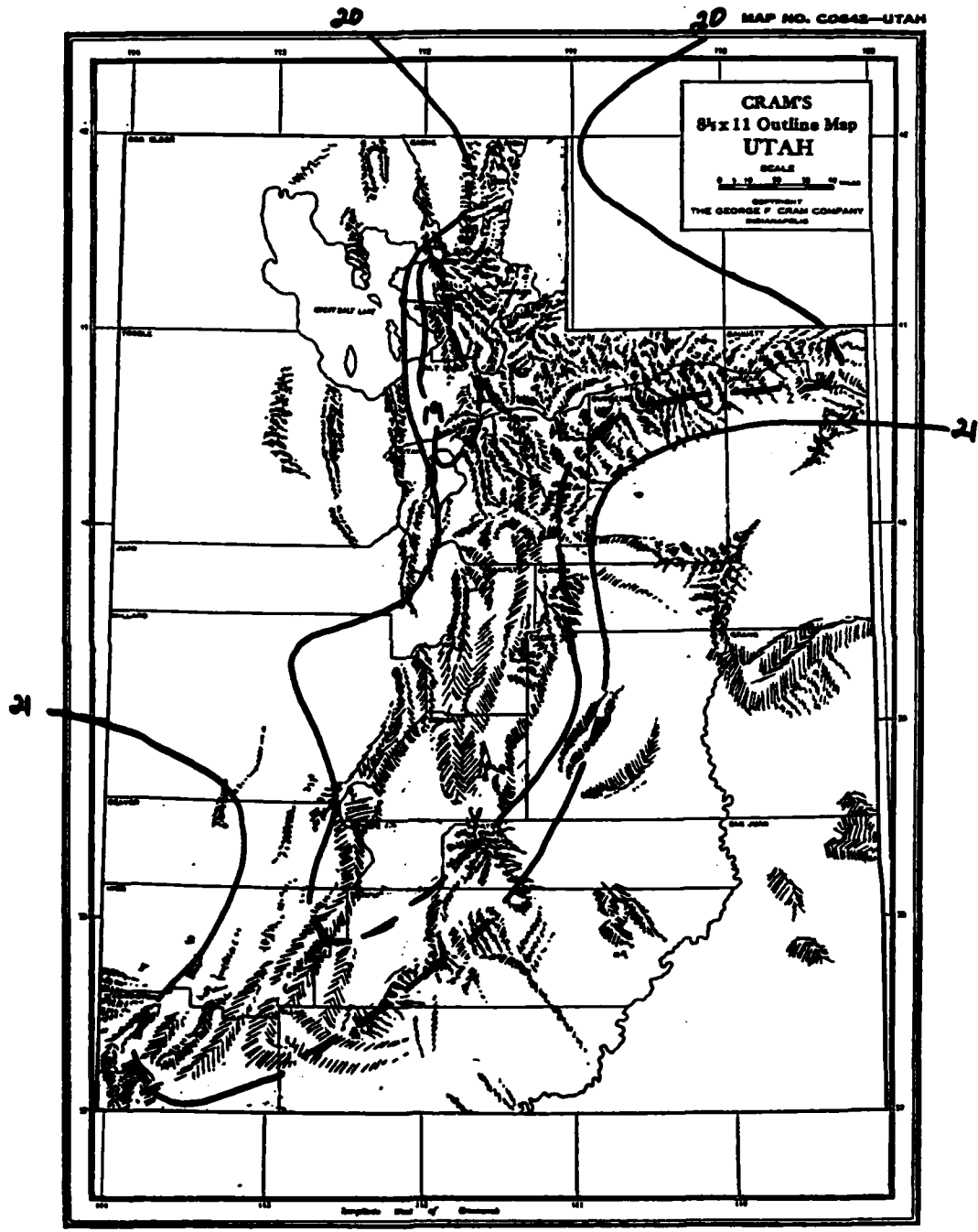
Figure 42. Monthly distribution of irradiance in Utah. Month of September. Units are: MJm^{-2} day^{-1}
