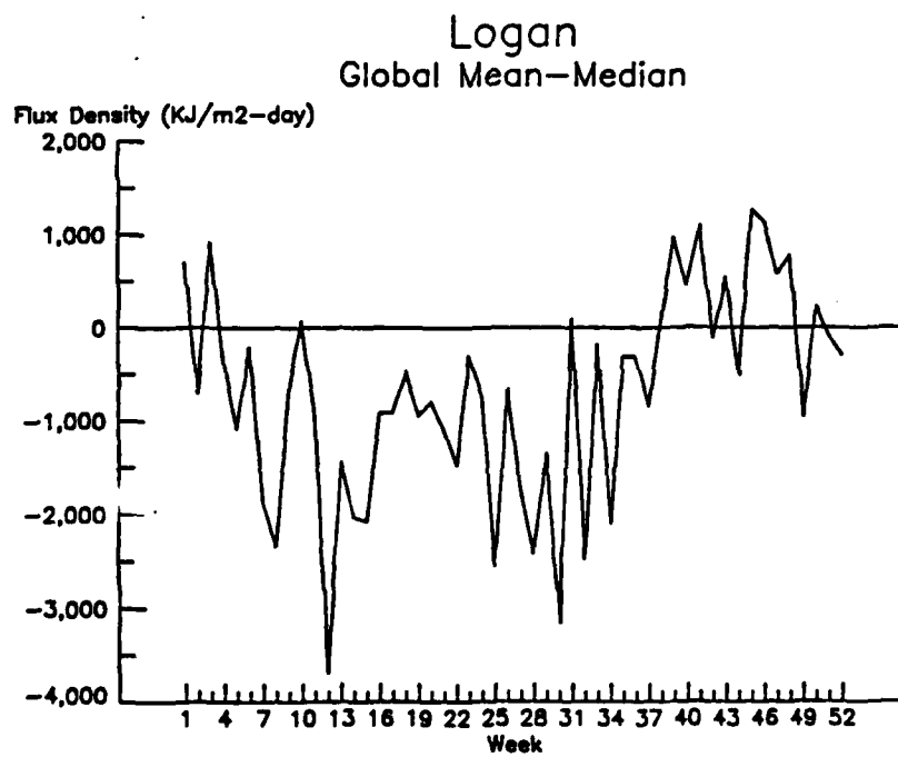
Figure 9. The difference between mean and median daily radiation for each week and month of the year.
