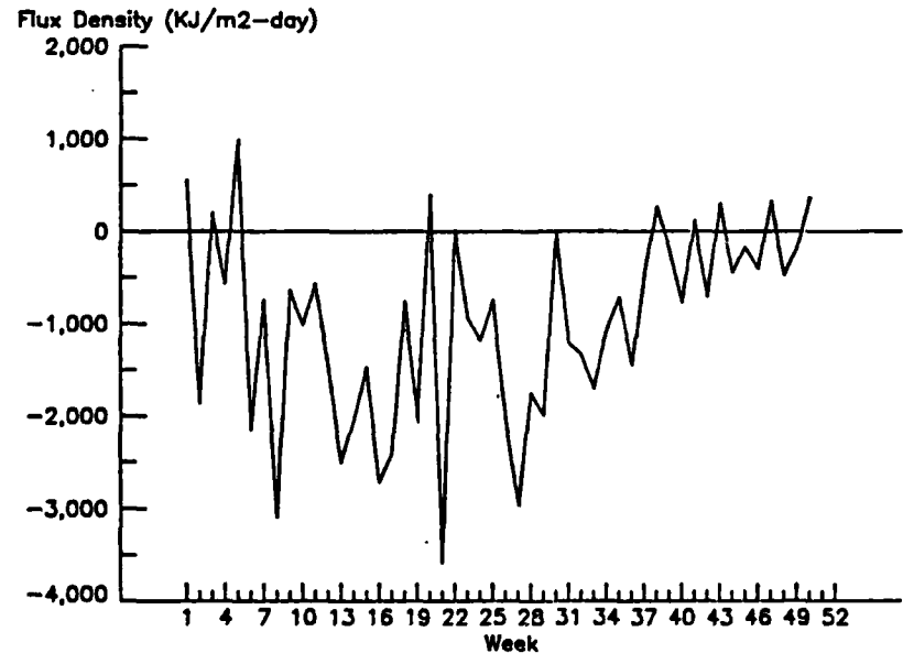
Figure 8. The difference between mean and median daily radiation for each week and month of the year.
