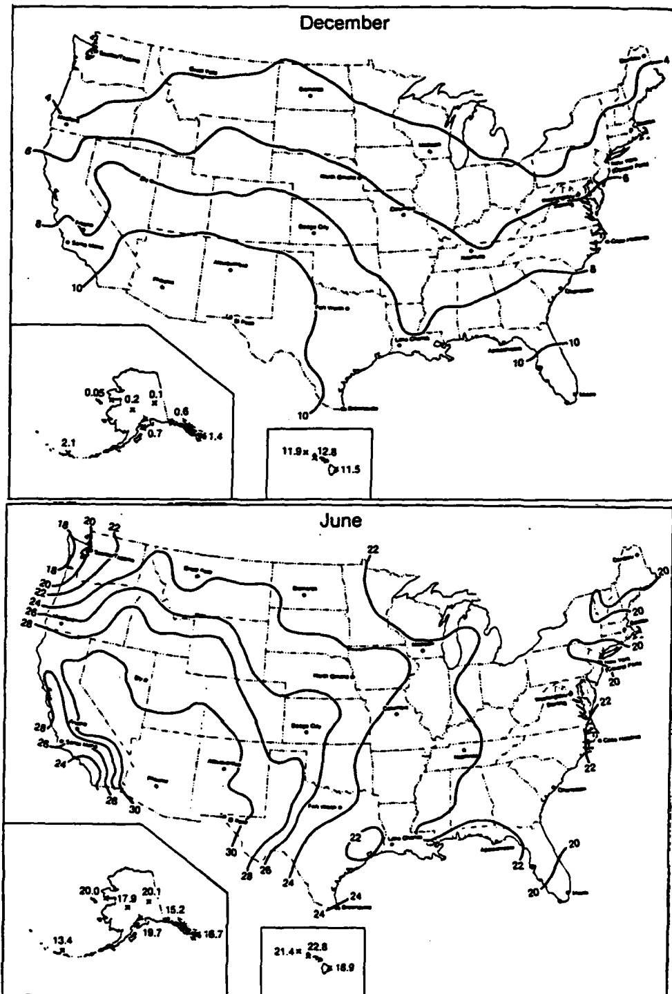
Figure 2. The distribution of global solar irradiance in the United States during December and June. (SERI, 1981) (units are MJ m -2 day -1 )
