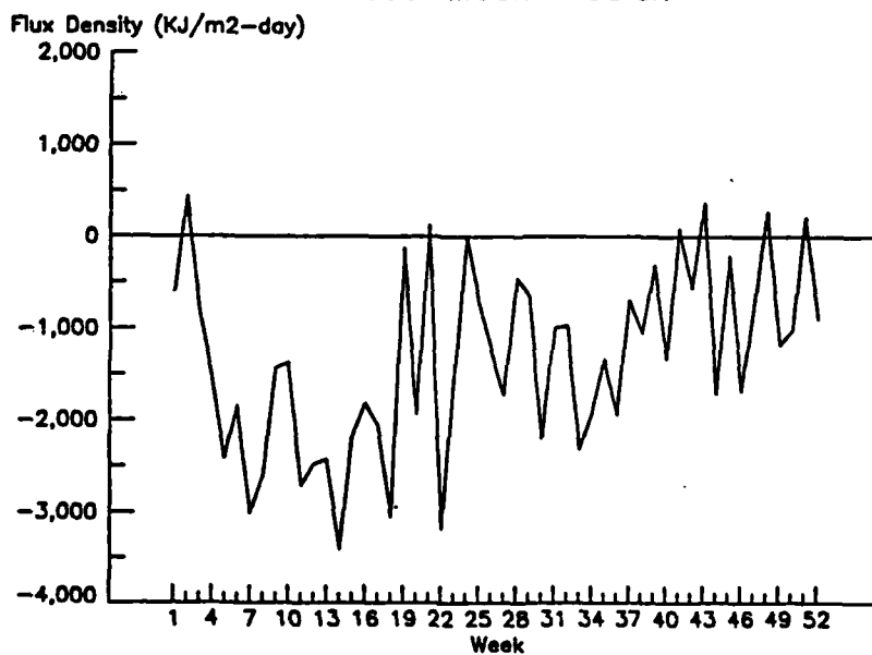
Figure 4. The difference between mean and median daily radiation for each week and month of the year.
