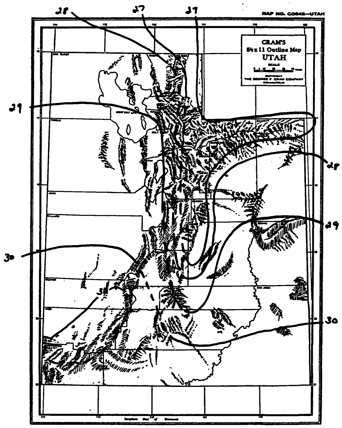
Figure 39. Monthly distribution of irradiance in Utah. Month of June. Units are: MJm^{-2} day^{-1}
