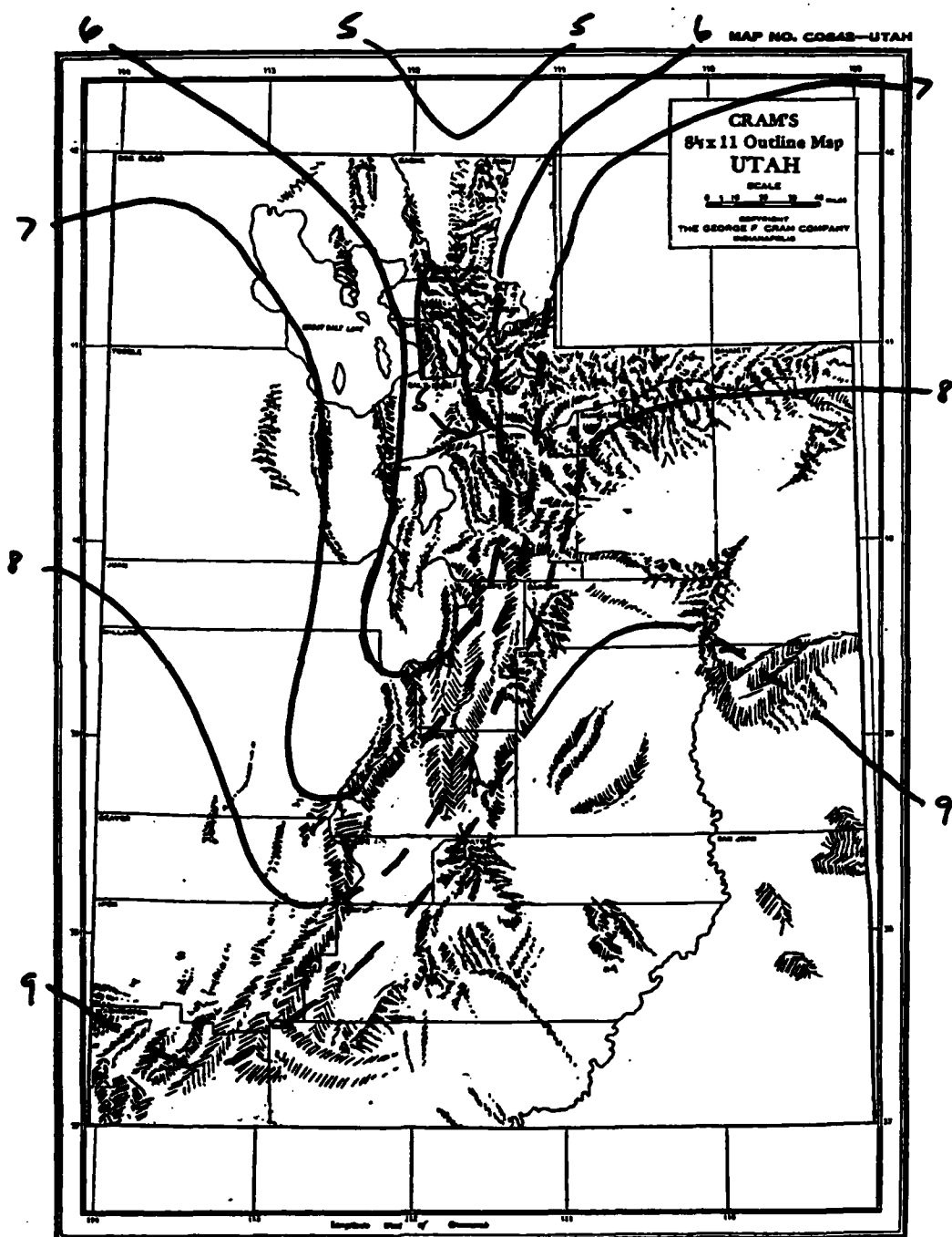
Figure 45. Monthly distribution of irradiance in Utah. Month of December. Units are: MJm -2 day -1
