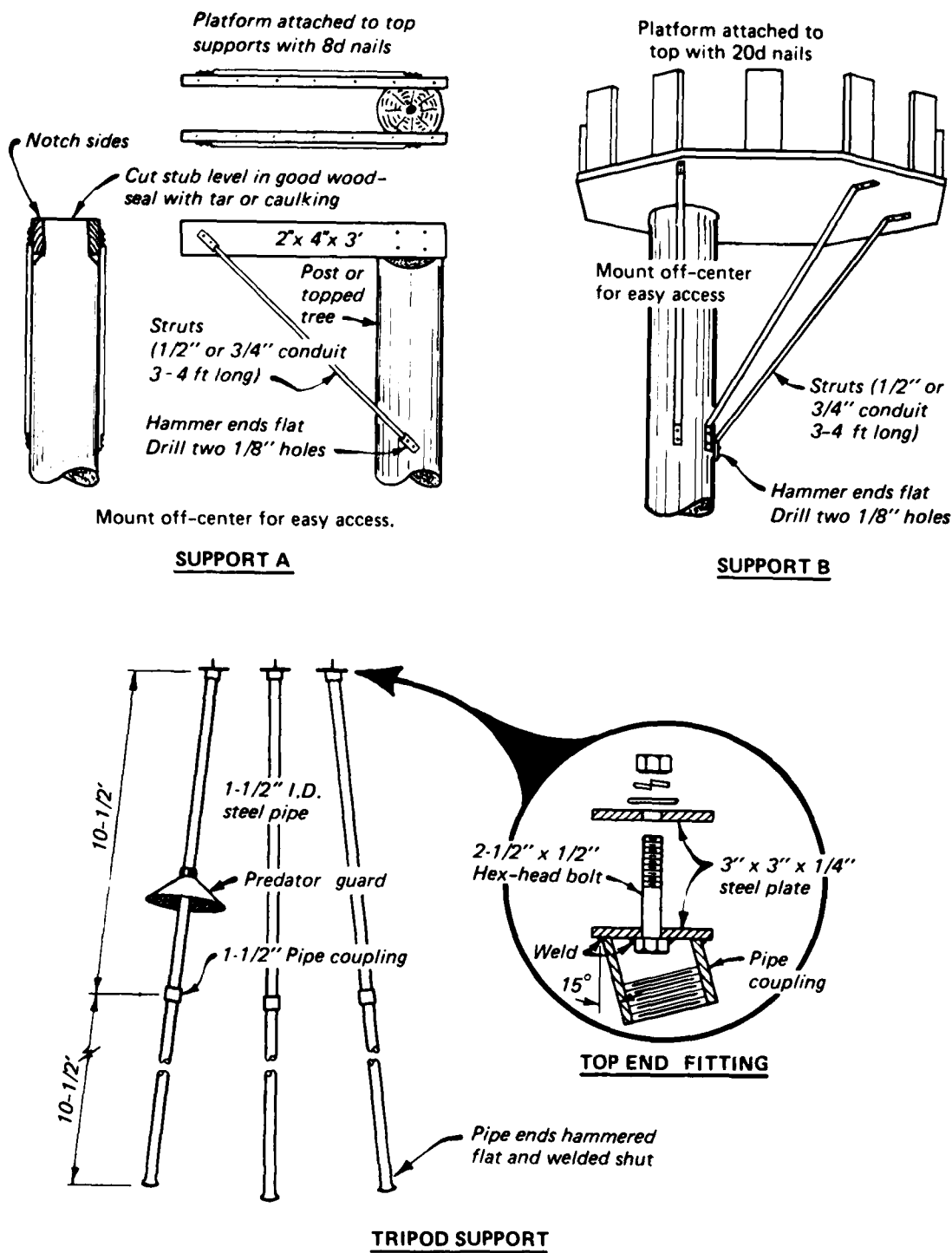
Figure 4. Design specifications for 3 types of supports used with a solid base osprey platform (after guidelines provided by Thomas U. Fraser, Sr., Conservation for Survival)
