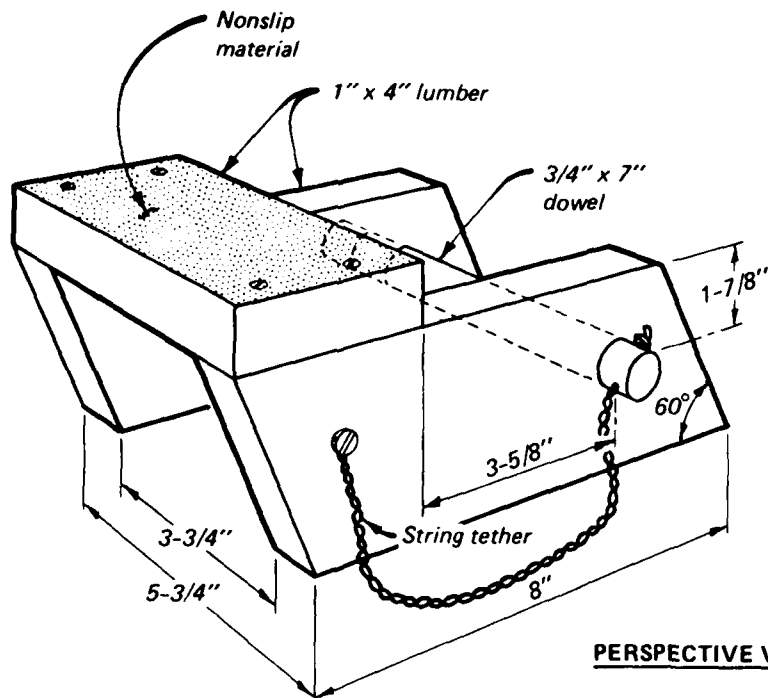
Figure 7. Construction details and materials for removable steps attached to one leg of a Sanibel Tripod (after Webb and Lloyd, in press)
