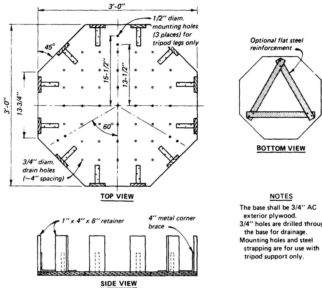
Figure 3. Design specifications for a solid base nesting platform for ospreys (after guidelines provided by Thomas U. Fraser, Sr., Conservation for Survival)
