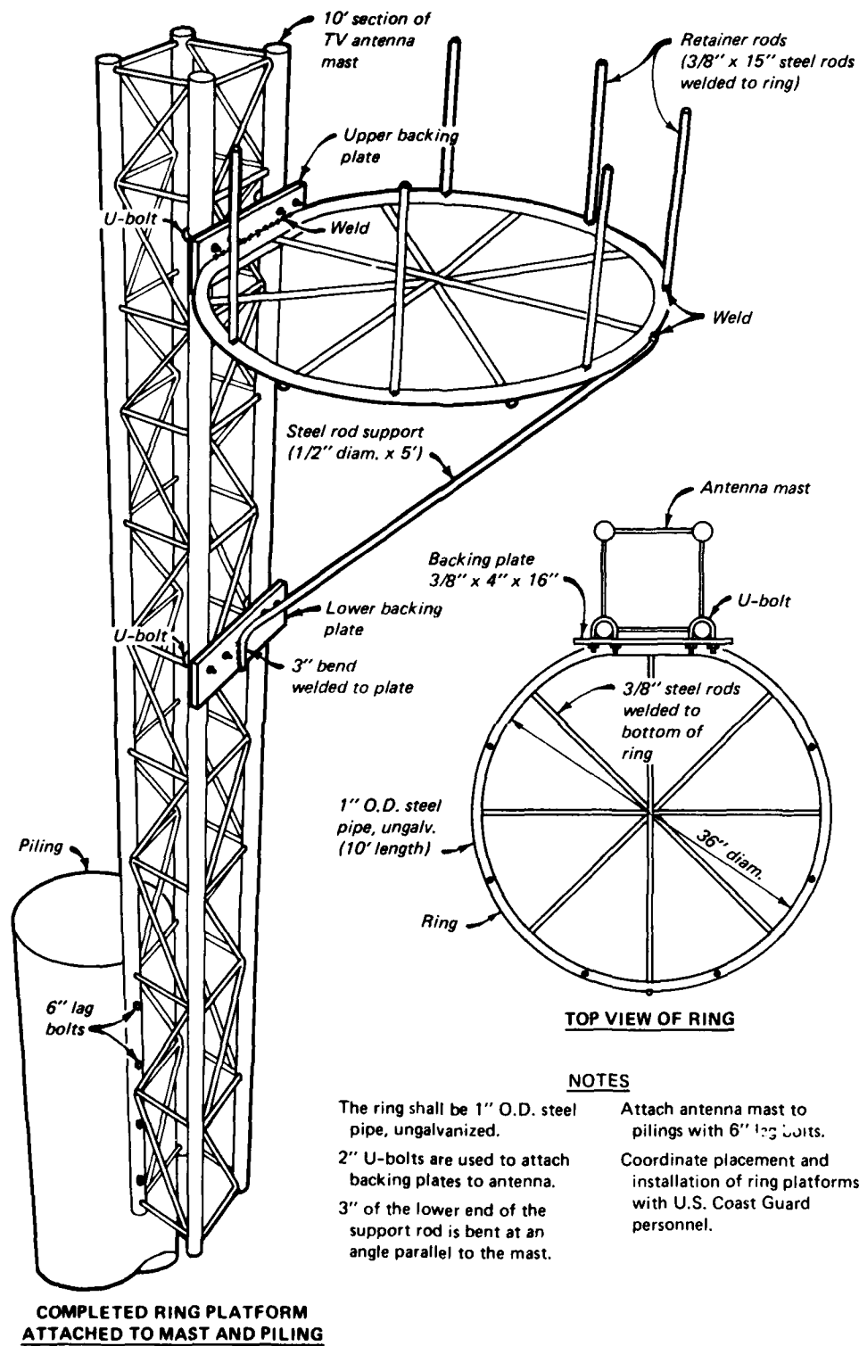
Figure 5. Design specifications for a ring nesting platform for ospreys that can be installed on marine navigation aids
