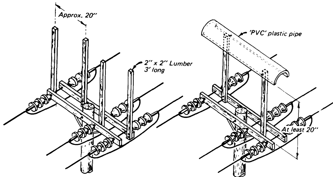
Figure 8. Osprey nesting discouragement devices for use on power poles (from Van Daele et al. 1980)
