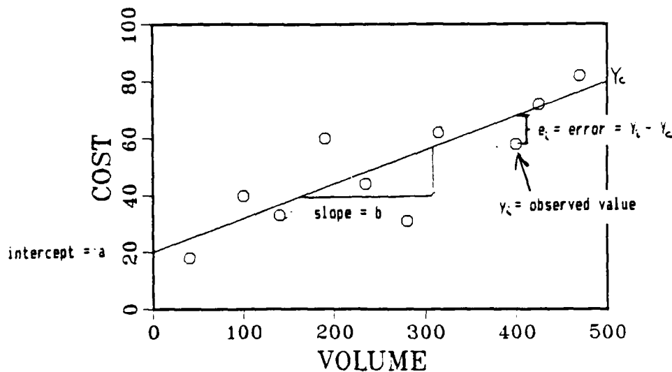
Figure 3.1 Linear Regression
