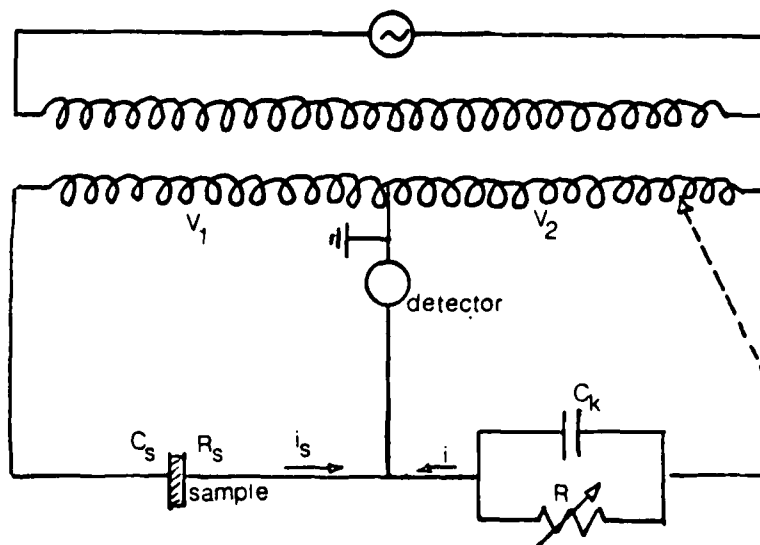
Figure 4.8 Schematic of a complex impedance bridge (G.C. Kolodziejczak in Radiation Induced Dielectric Relaxation In Rare Earth Doped Calcium Fluoride. Report to the Trident Scholar Committee. Annapolis, MD: U.S. Naval Academy, 1978)
