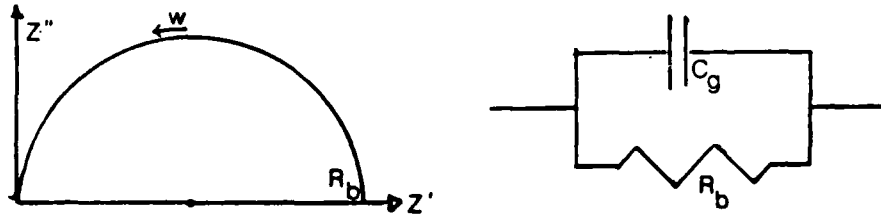
Figure 2.3 The bulk resistance is R_b .
