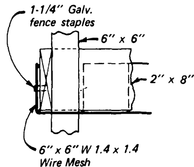
CONNECTION C
