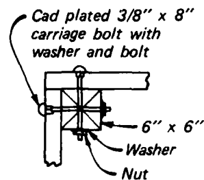
CONNECTION A
