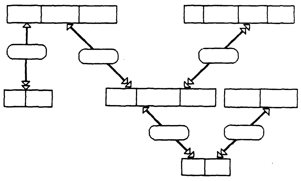
Figure 6. A Network data model
