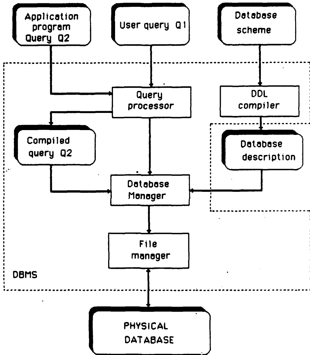
Figure 3. Schematic diagram of a database system.
