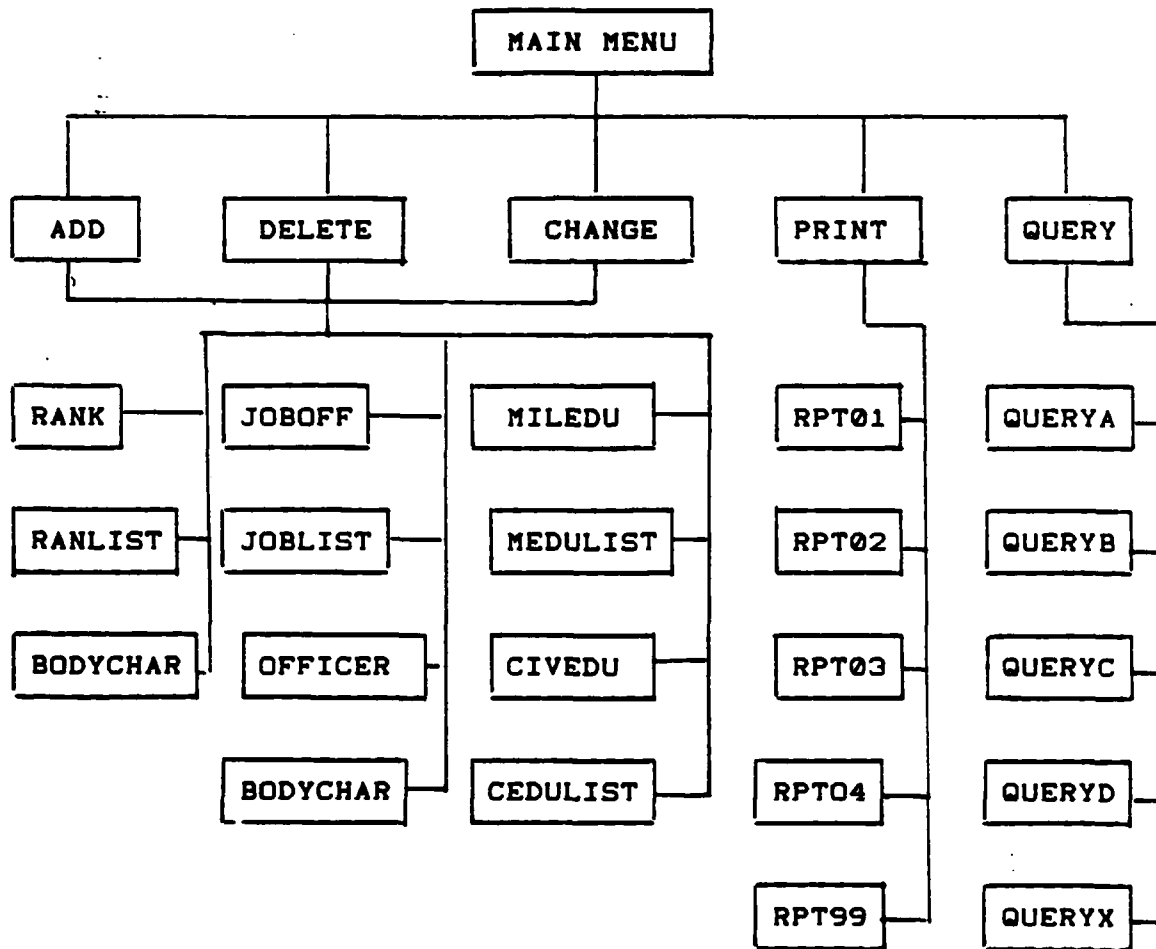
Figure 4.3 Hierarchy chart of the system.
