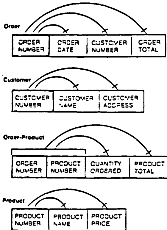
Figure 3.8 Third Normal Form.
