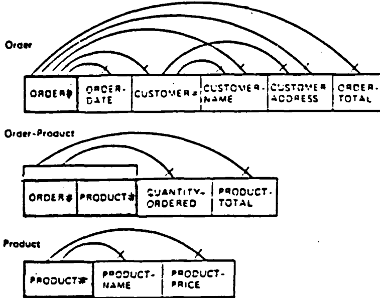
Figure 3.7 Second Normal Form.
