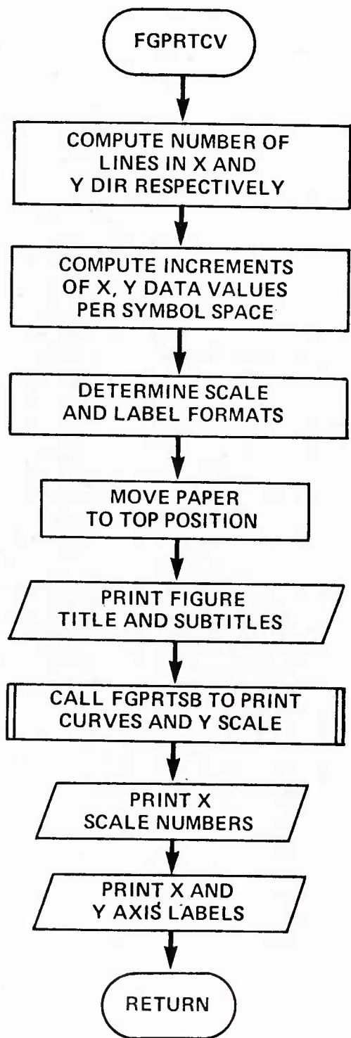
Flowchart of Subroutine FGPRTCV
