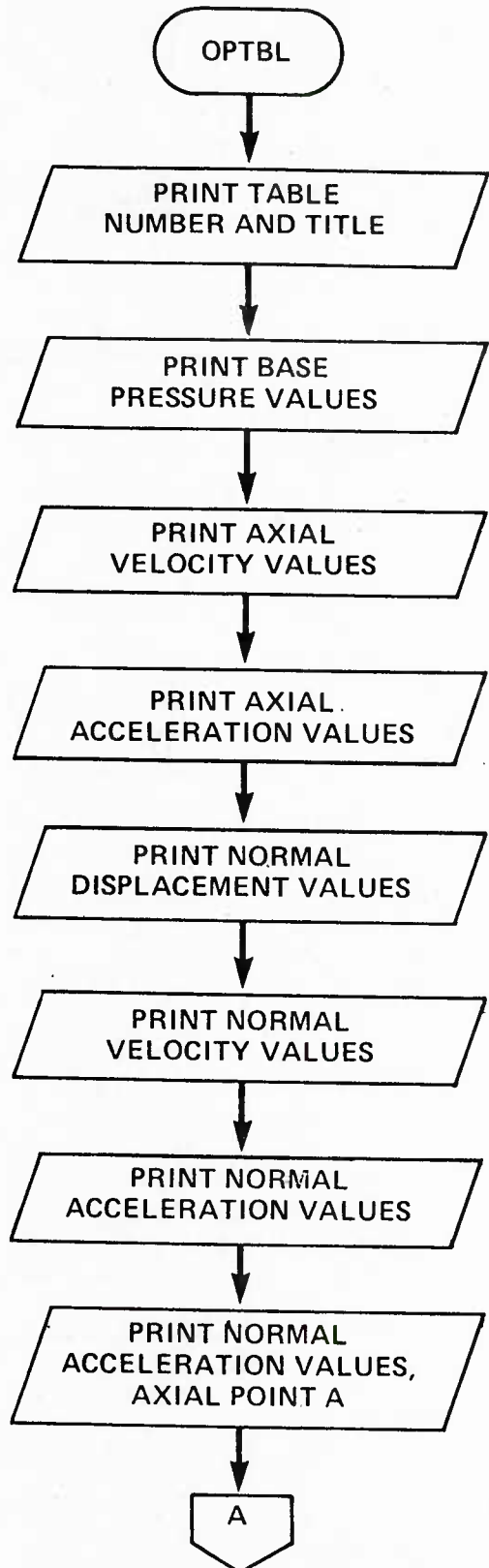
Flowchart of Subroutine OPTBL
