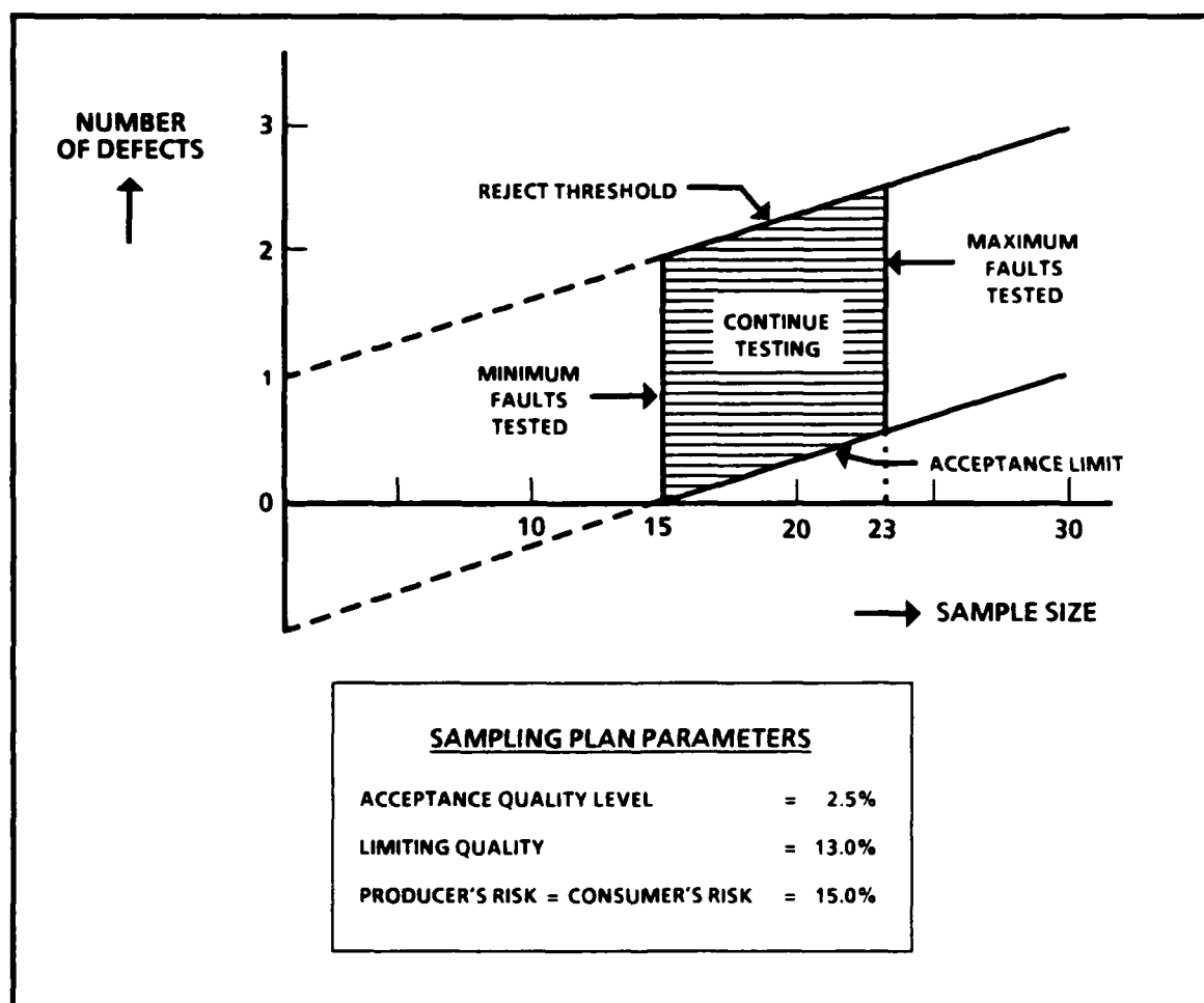
FIGURE 4-4. SEQUENTIAL SAMPLING CHART FOR TPS ACCEPTANCE TEST
