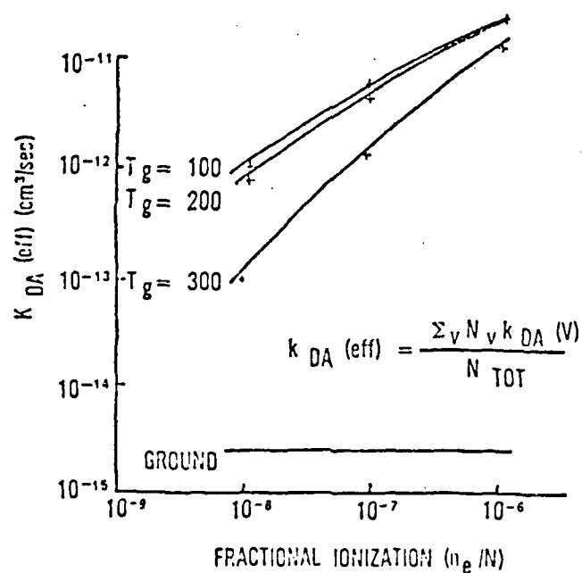
Figure 5. Effective rate constant of H - production including all vibrational levels as a function of fractional ionization and gas temperature. Discharge conditions of 40 Td are assumed. (after [5]).
