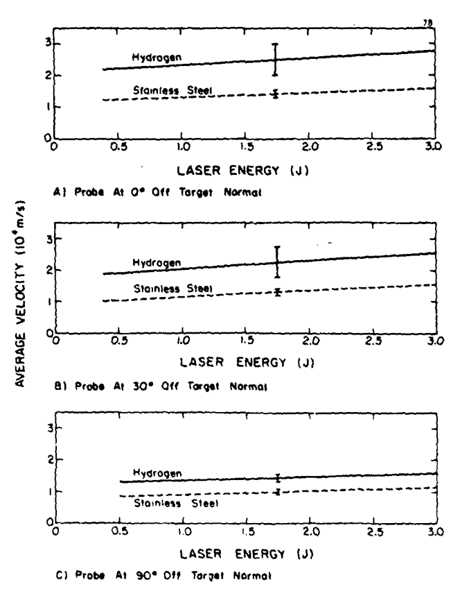
FIG. 8. Average ion velocity as a function of laser energy for a 0.025-cm hydrogen slab and bare stainless steel. Maximum velocity is approximately 1.5 times the average velocity.
