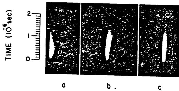
FIG. 3. Typical streak photographs for the laser beam incident on (a) the stainless-steel substrate, (b) a 0.060-cm-thick hydrogen slab against the substrate, and (c) a 0.025-cm-thick hydrogen slab against the substrate.
