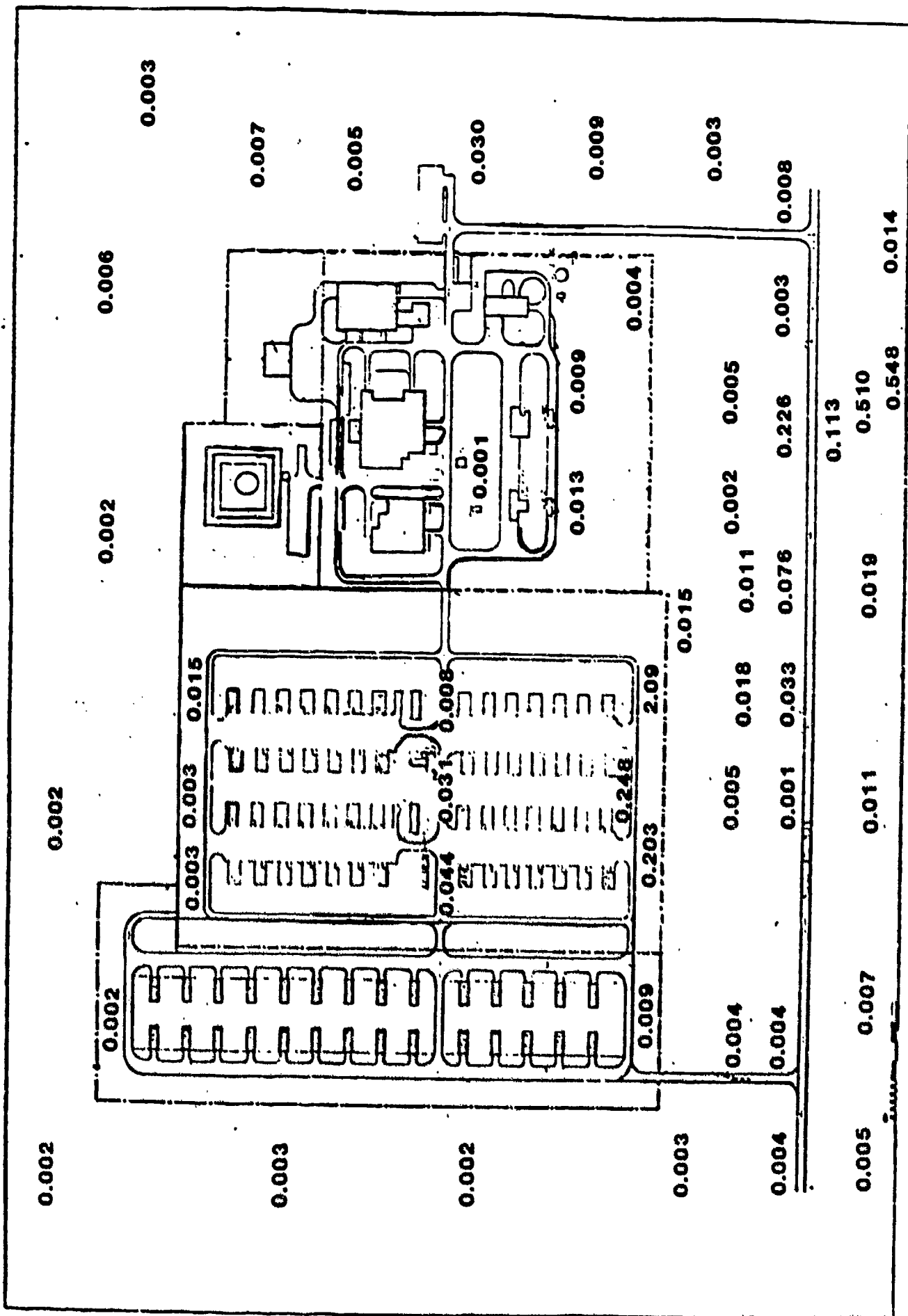
Figure 5. 1985 Pu ^{239,240} Soil Concentrations ( \mu\text{Ci}/\text{m}^2 )
