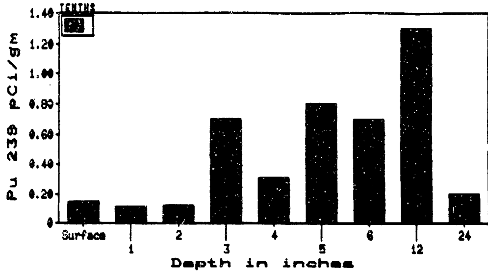
Figure 11: Vertical Pu-239 Soil Distribution, Site K0671
