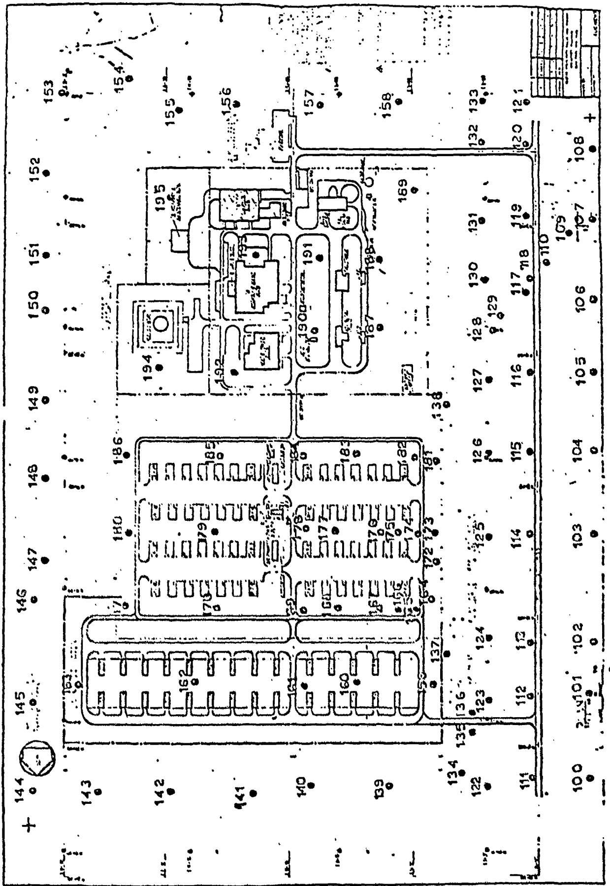
FIGURE 3 Soil Sampling Sites, BOMARC Site
