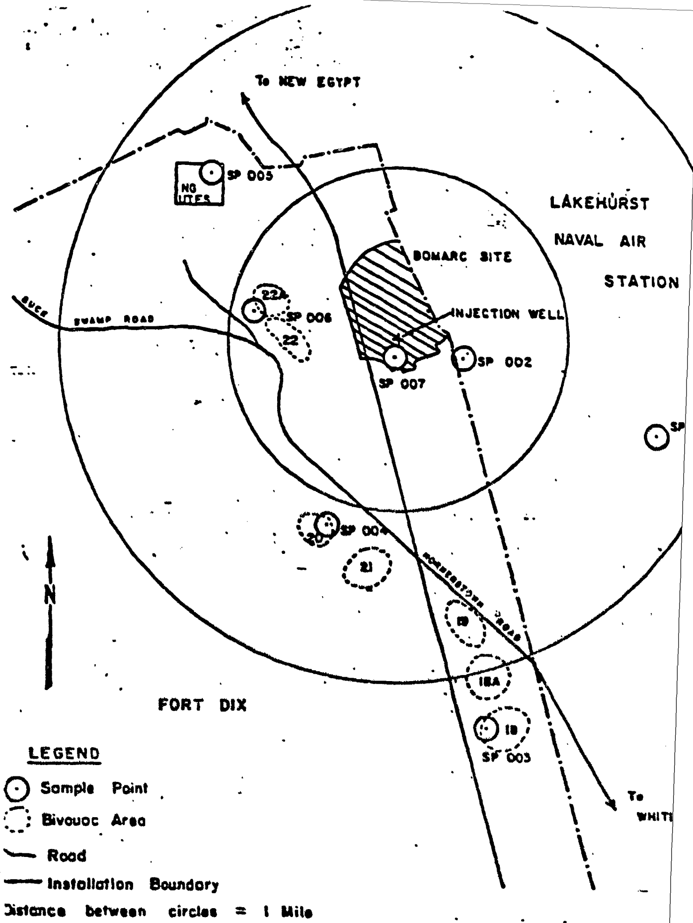
FIGURE 8 1985 Government Well Sampling Sites
