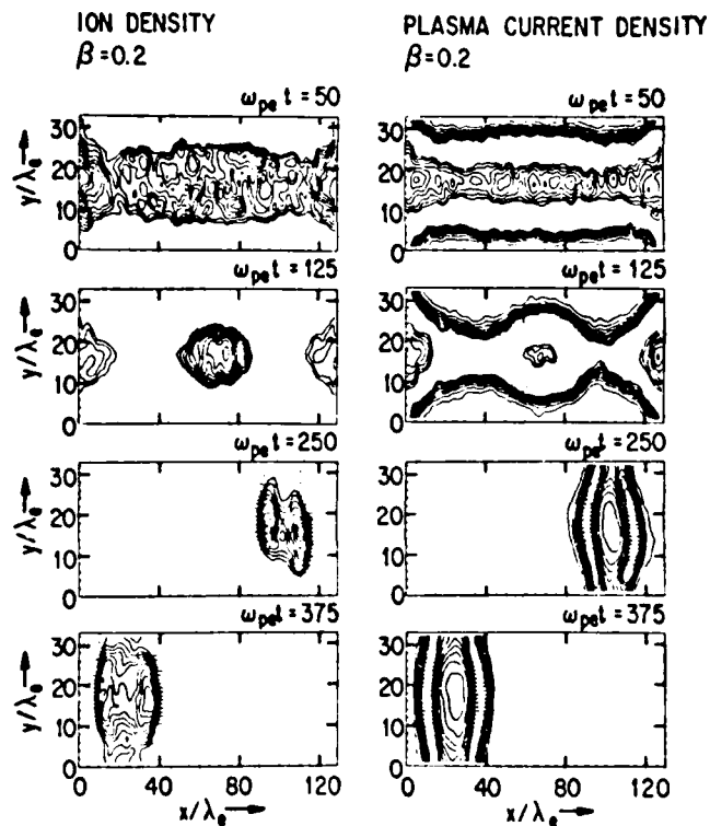
Fig. 14. 127x32 island coalescence run. The ion density is displayed on the left at, from top to bottom, \omega_{pe} t = 50, 125, 250, and 375. The dotted contours represent levels below the average density at a particular time, full contours levels above. The plasma current density in the z direction is shown on the right at equivalent times. Dotted contours indicate regions of highest return current (Leboeuf et al. 1982).
