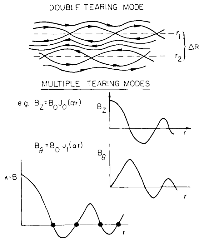
Fig. 9. Top: The simplest example of multiple tearing modes, the double tearing mode, in which k \cdot B = 0 occurs at two different radii from the center of the loop. Bottom: The Lunquist field in which multiple tearing modes can occur (Kahler et al. 1980).
