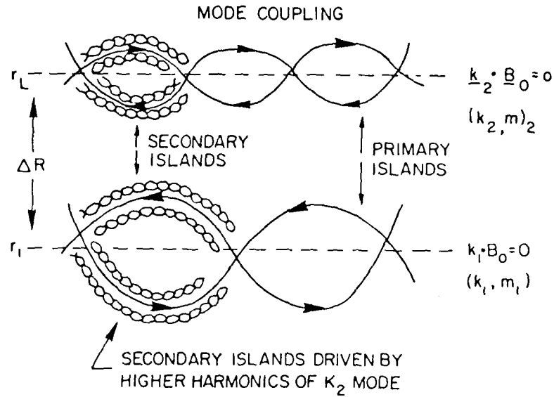
Fig. 10. The phenomenon of mode coupling. Primary islands are generated when k \cdot B_0 = 0 for different wave number vectors k . The coupling between these primary islands results in the generation of secondary islands of shorter wavelength k^{-1} (Kahler et al. 1980).
