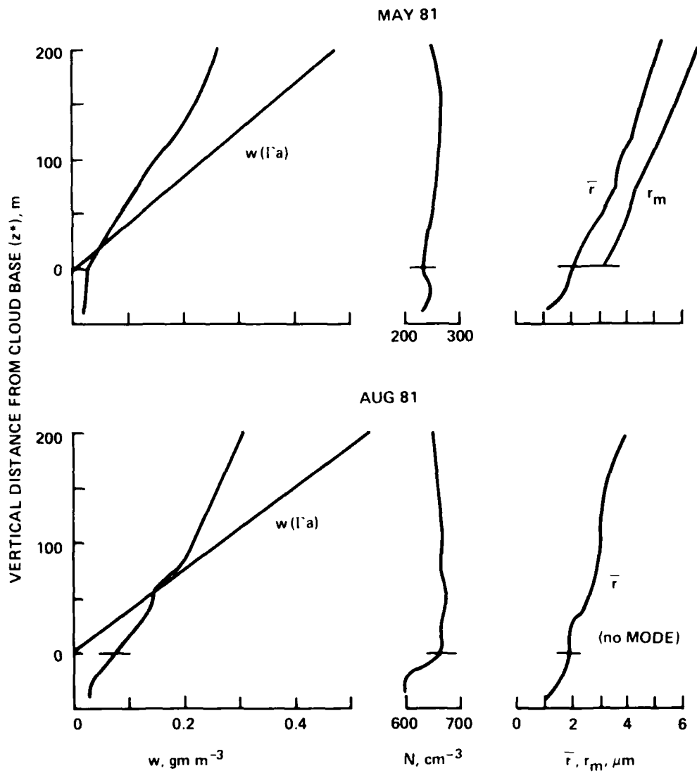
Figure 7. Vertical profile of aerosol spectral parameters in the cloud region averaged for the May and August days. w(\Gamma'a) is for moist adiabatic changes.
