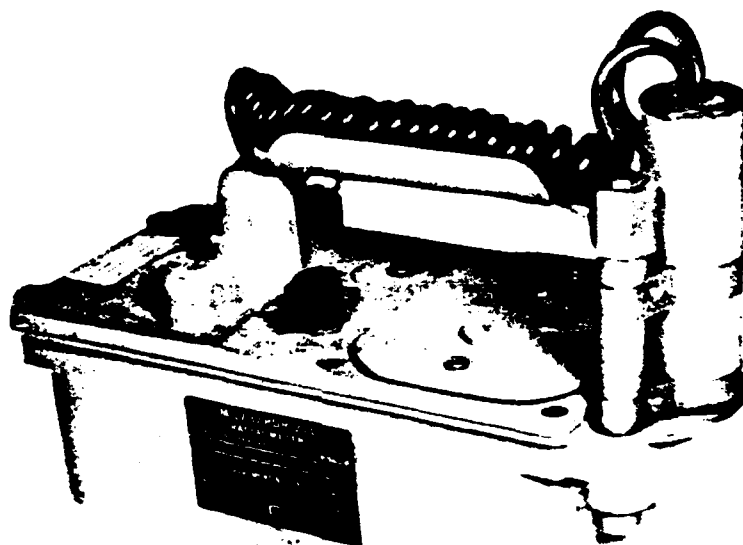
G-M TYPE RADIAC METER OF AN/PDR-27() RADIAC SET
