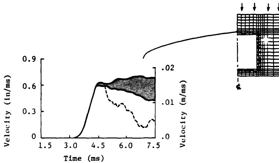
(a) Midspan slab velocity
