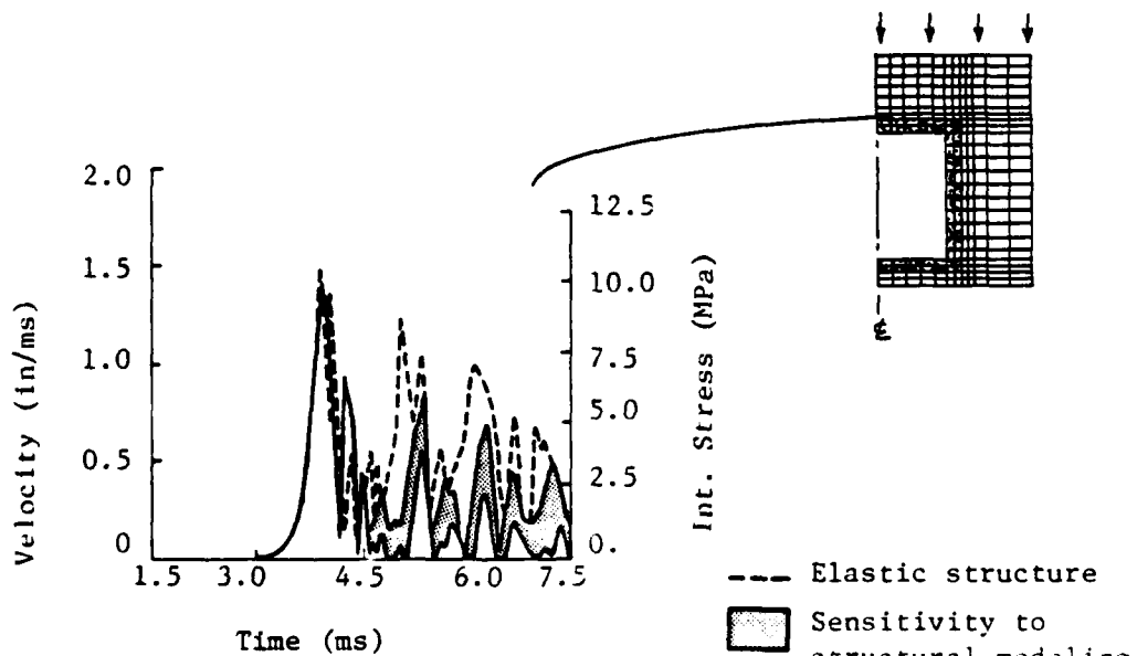
(b) Midspan interaction loading on roof
