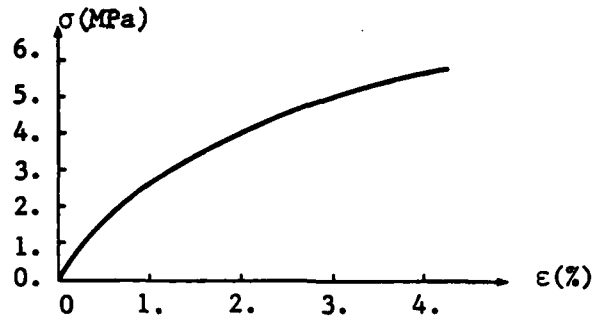
(a) Crisp stress-strain law
