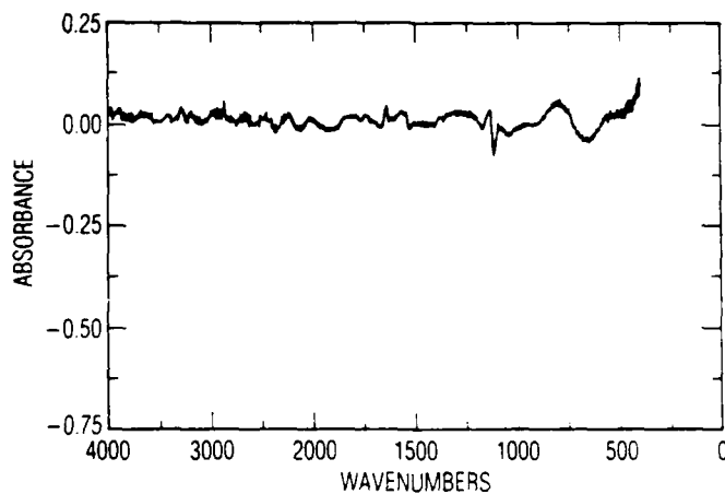
Fig. 2. Validation of Measurement Technique on PRC 1535 Samples Having Peak Absorbance Values Similar to Those of Uralane 5753. (FCR = 1.84 for the difference spectrum in the bottom graph.)
