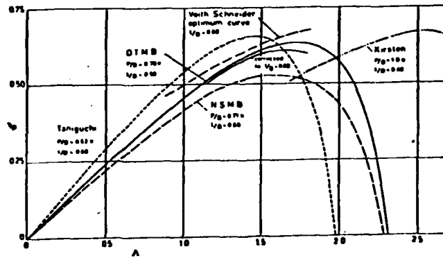
Figure 8. Propeller efficiency of compared vertical axis propellers.
