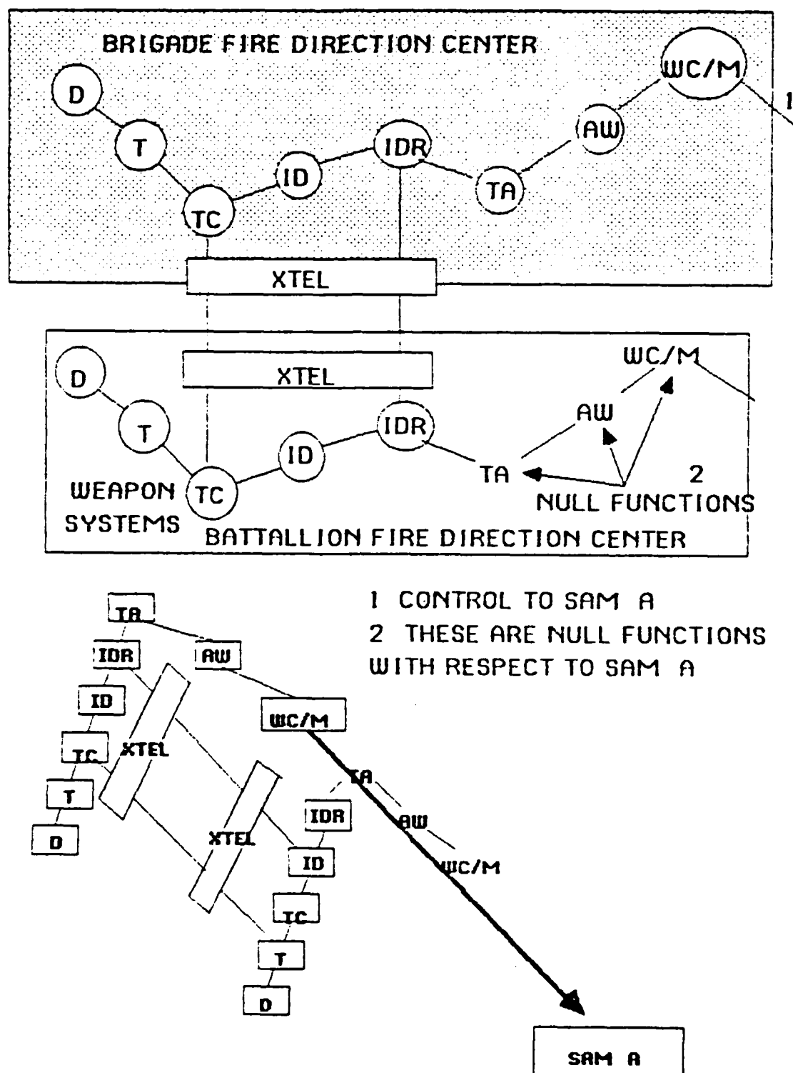
Figure 5.4 Null Process with Vertical C2 Nodes
