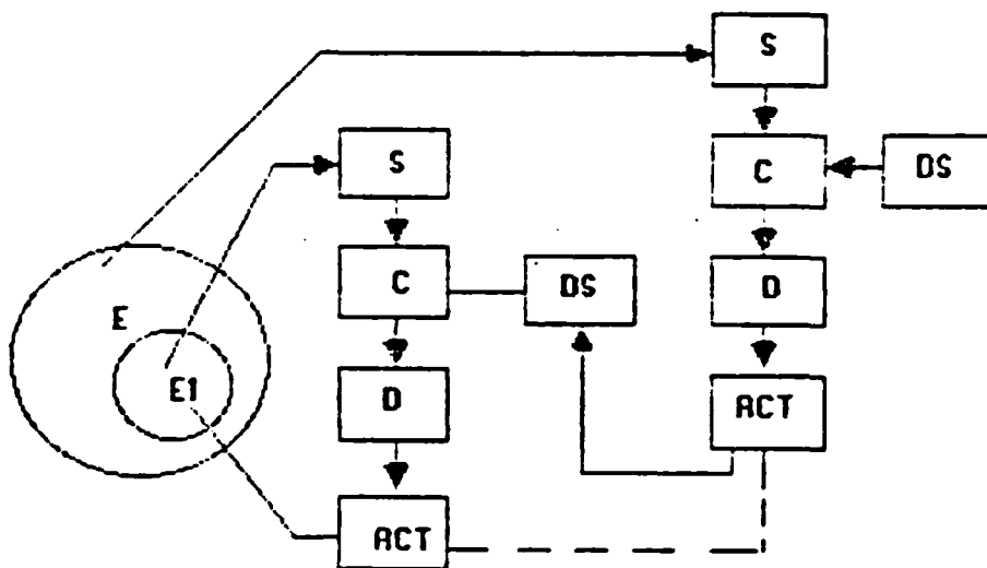
LAWSON NESTED C2 PROCESS
