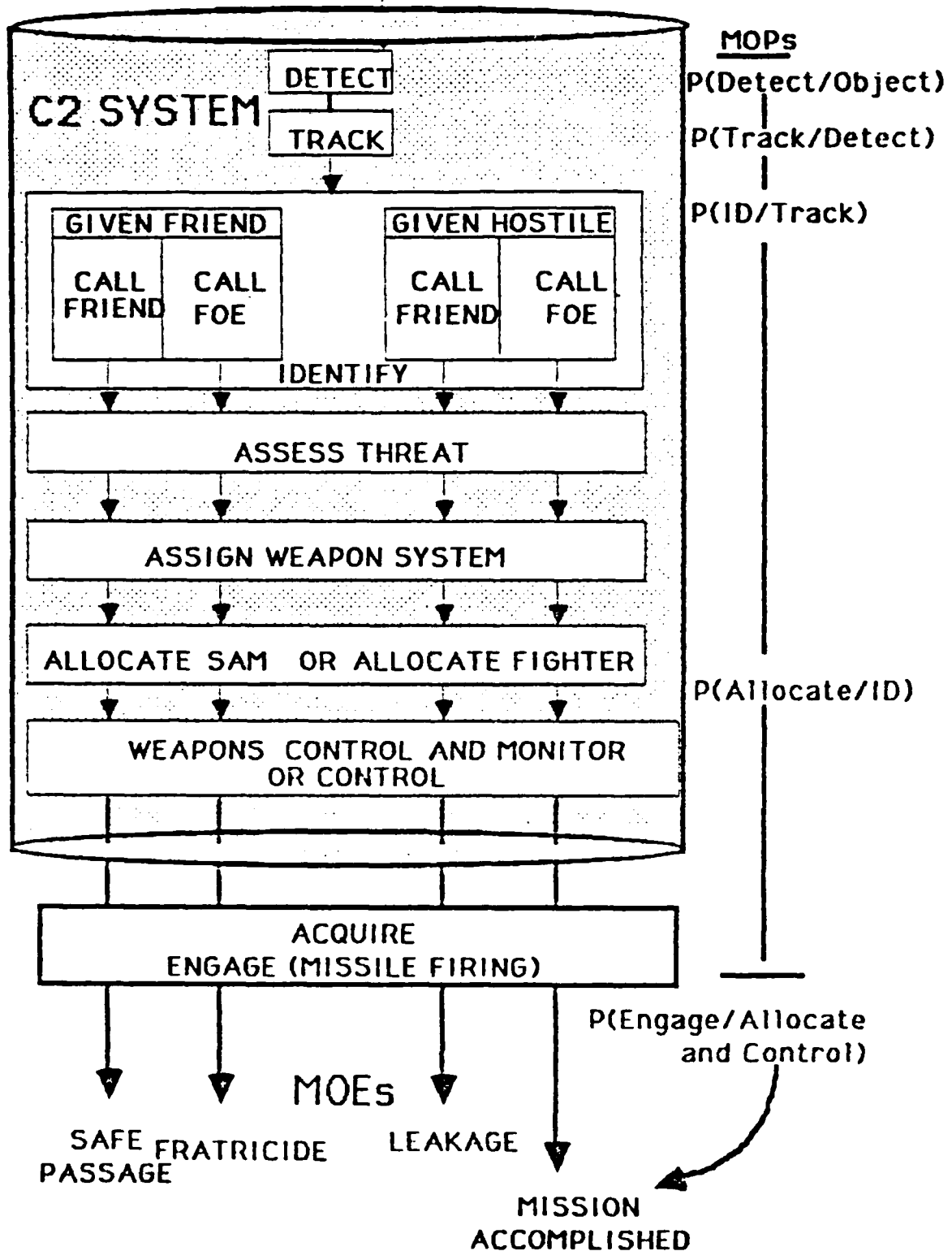
Figure 6.2 Relationship between MOPs and MOEs
