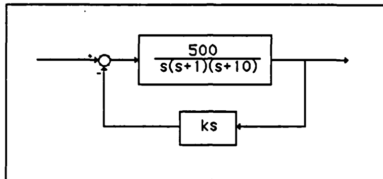
Figure 3.4 Single Loop System
