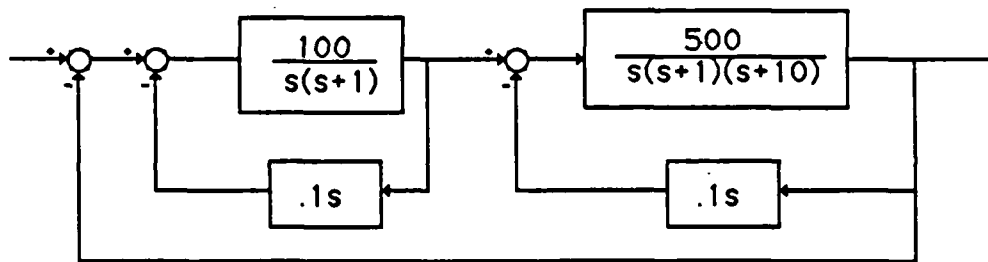
Figure 3.17 Nested and Cascaded Loops
