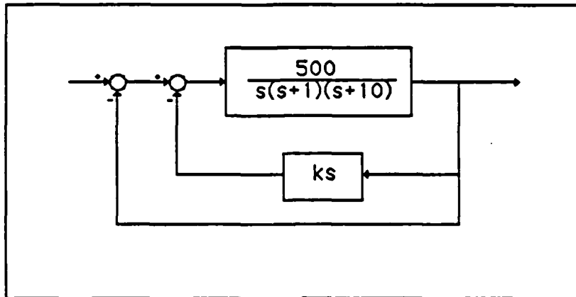
Figure 3.9 Nested Loops
