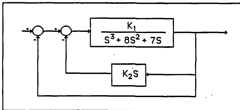
Figure 2.23 Velocity Feedback
