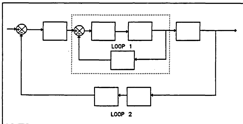
Figure 3.12 Sample Multiloop System
