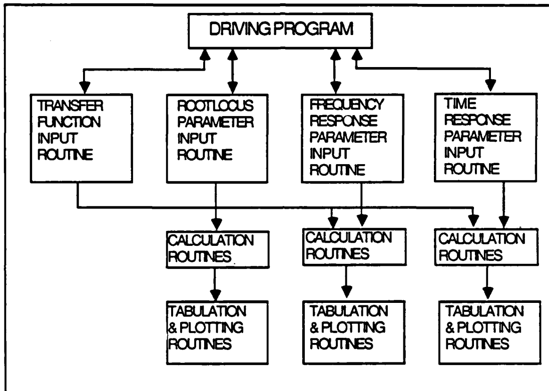
Figure 2.1 Program Organization
