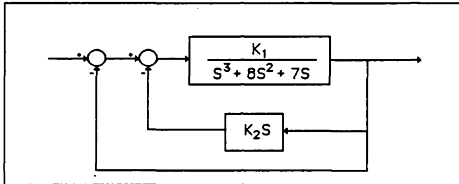
Figure 2.23 Velocity Feedback
