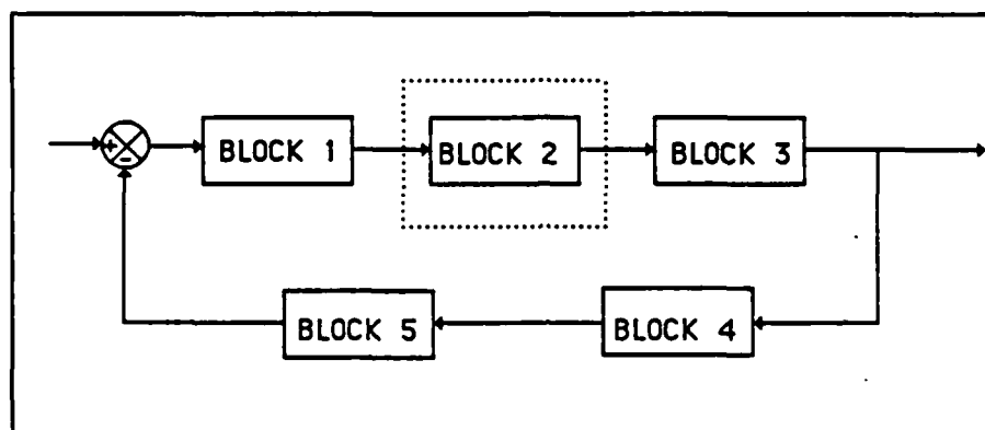
Figure 3.13 Reduced Multiloop System
