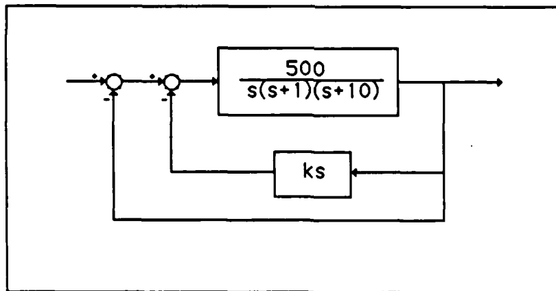
Figure 3.9 Nested Loops
