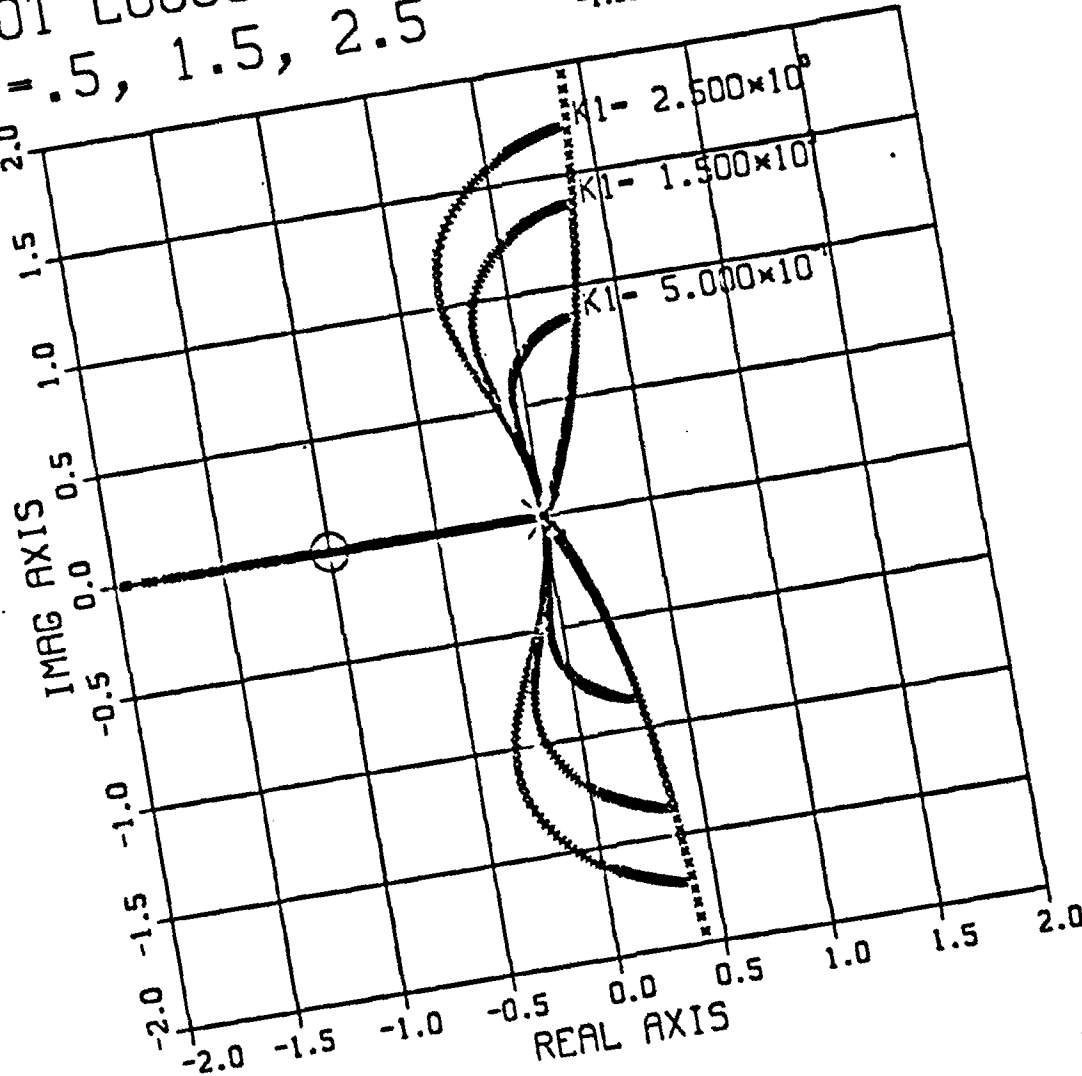
Figure E.6 Root Locus Family Example
