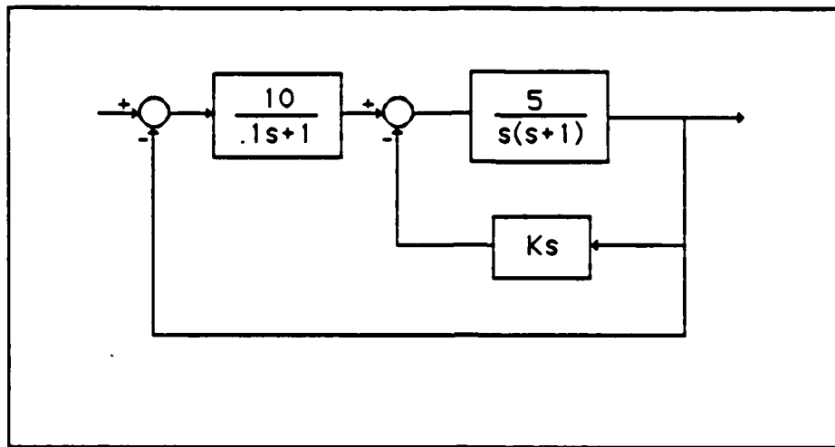
Figure E.5 Multiloop System
