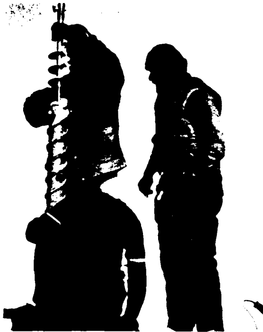
Figure 18. Rand drill with section of flight auger for stirring cuttings above the core barrel.
