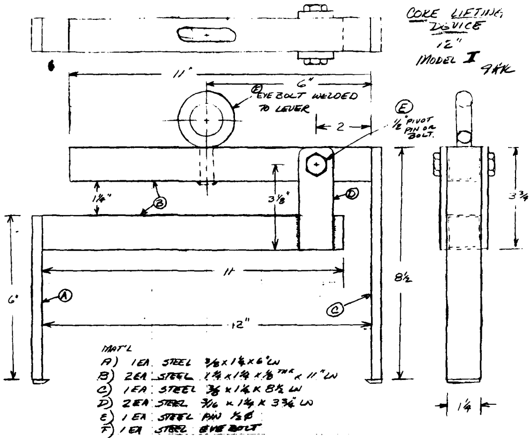
Figure 27. Two-prong gripper for lifting 12-inch ice cores.
