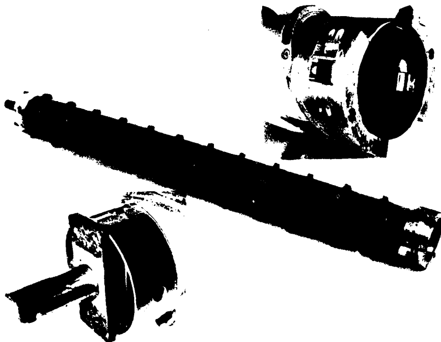
Figure 11. First version of the 4 1/4-inch Rand auger.
