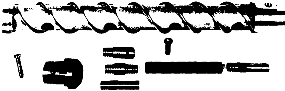
Figure 7. 3-inch CRREL auger with heavy-duty driving head and connectors.
