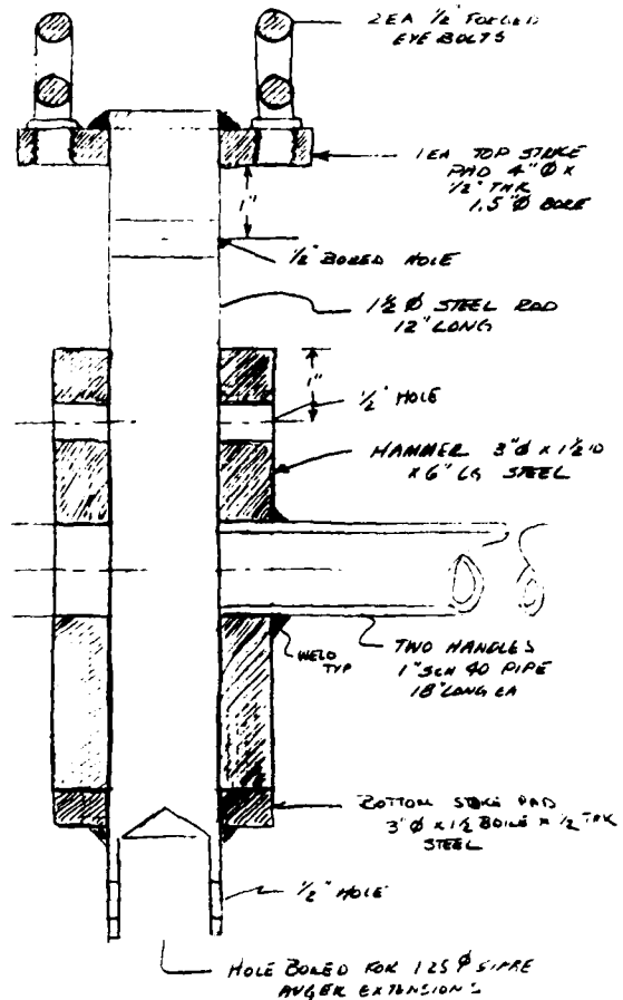
Figure 17. Reverse impact hammer for seating core dogs and breaking core.
