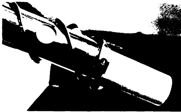
Figure 5. Core being removed from the upper end of the core barrel of the 3-inch auger (driving head removed).
