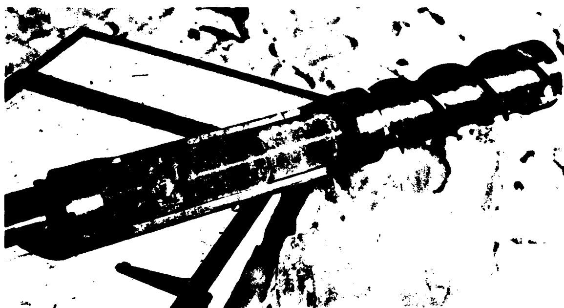
Figure 1. The original ACFEL ice coring auger, showing the core barrel and the attachment for removing cores.
