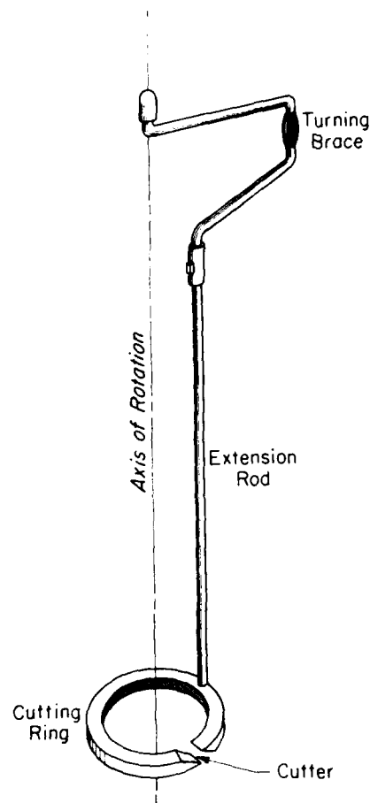
Figure 31. Ice-fisherman's auger (PI-8) used for shallow coring in the U.S.S.R.
