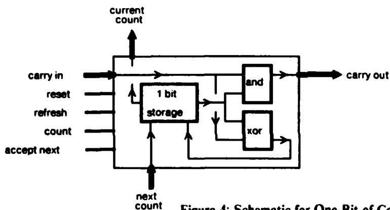
Figure 4: Schematic for One Bit of Counter
