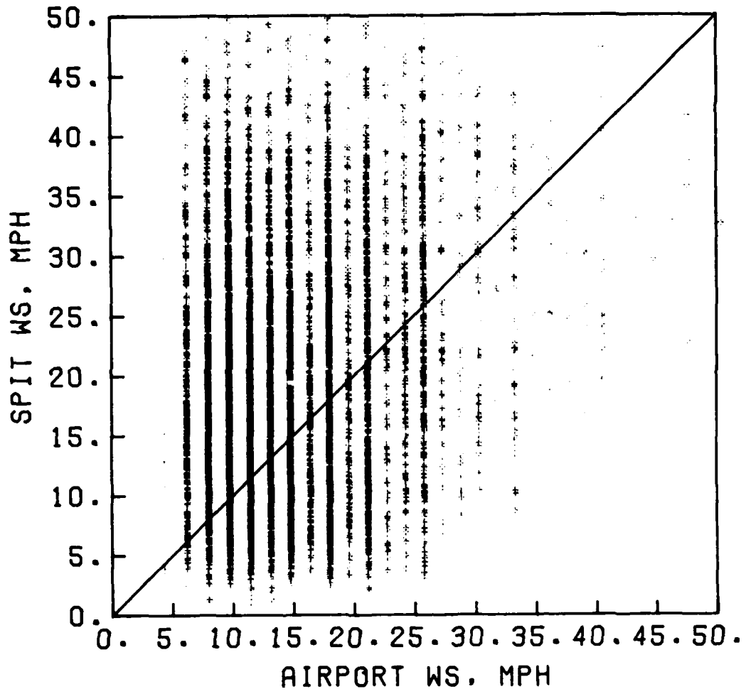
Figure A-8. Scatter plot of paired spit and airport observations
