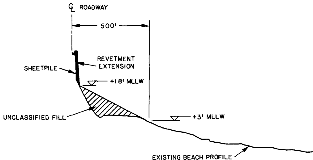
Figure 13 - Typical cross section for Alternative 3 uniform beach fill with revetment extension
