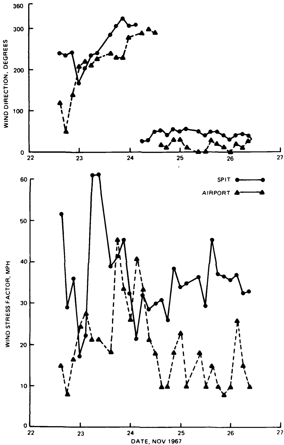
Figure A-10. Comparison of time-histories from the Spit and airport anemometers, Homer, Alaska
