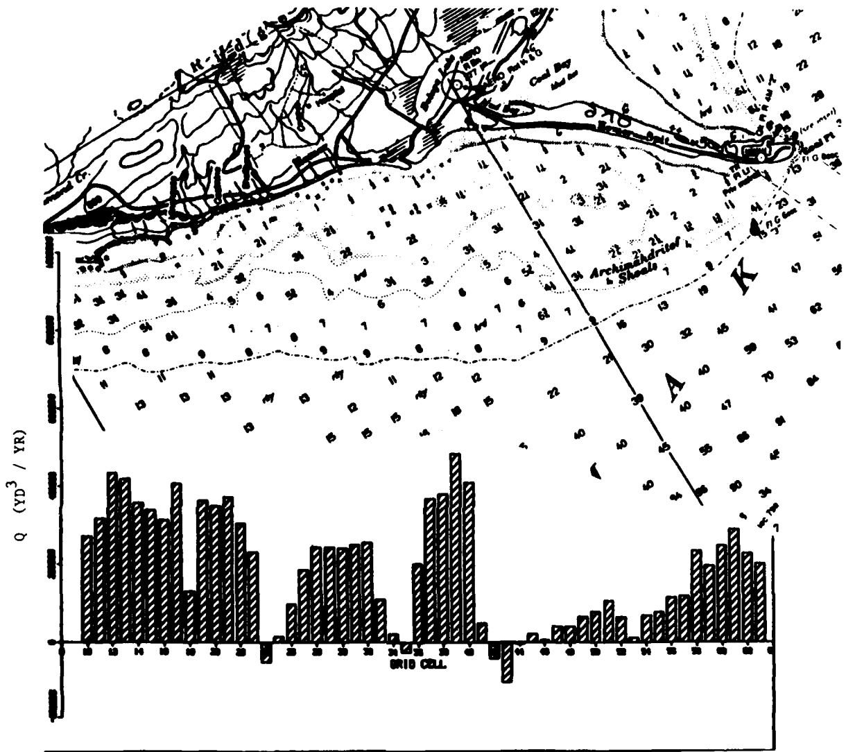
Figure B-5 - Expected annual sediment transport for each grid cell (airport wind distribution)
