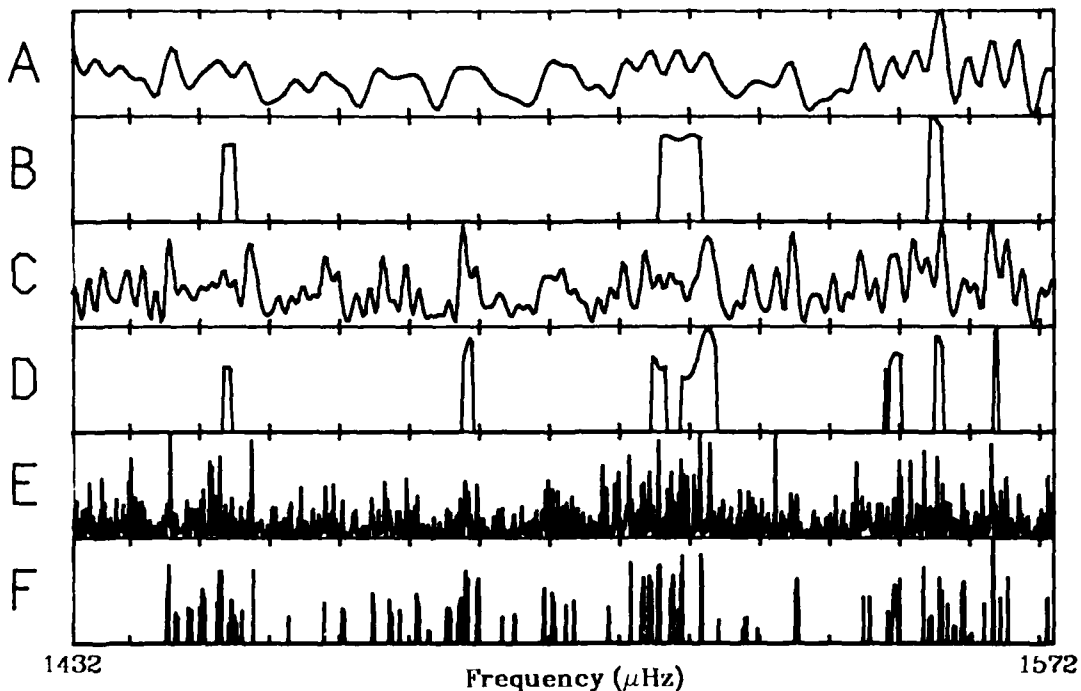
Figure 3 Plot of data in the frequency range from 1432 \mu\text{Hz} to 1572 \mu\text{Hz} : A) average power spectrum of 4 day chunks of data, B) peak search on A, C) average power spectrum of 8 day chunks of data, D) peak search on C, E) full resolution power spectrum, F) peak search on E.
