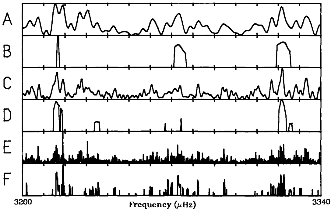
Figure 4 As figure 3, but for the range from 3200 \mu\text{Hz} to 3340 \mu\text{Hz} .
