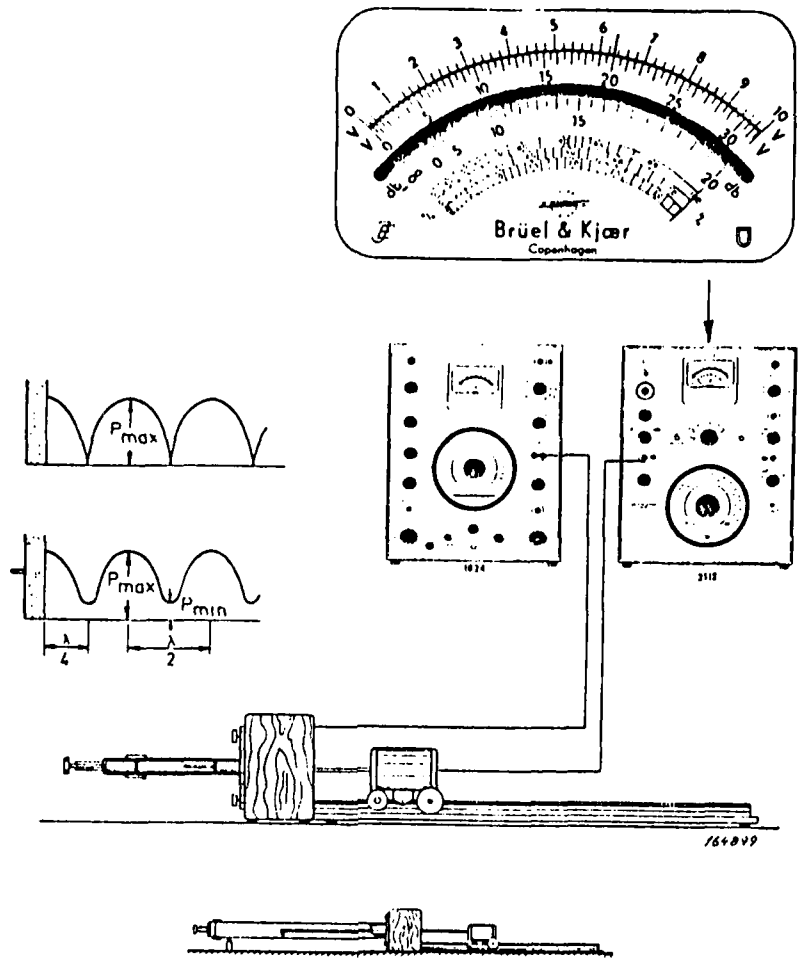
Figure A. The Standing Wave Apparatus Type 4002 mounted for low frequency 1/2 Octave Analyzer 2112.
