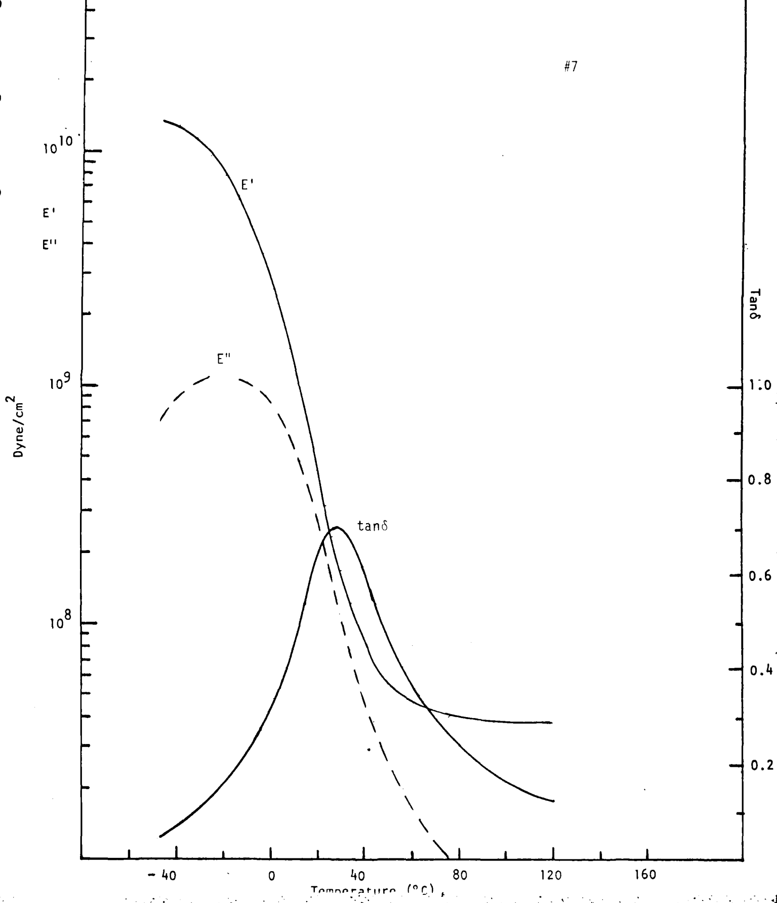
Figure 10. Dynamic mechanical spectroscopy of PU/Epoxy 60/40 with 20% #2 graphite, roll milled technique
