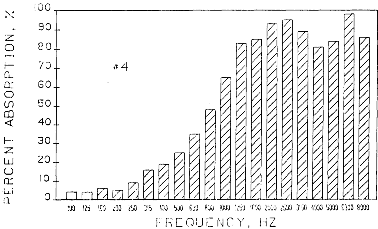
Figure 26. Sound absorption property of 50/50 PU/Epoxy IPN foam
