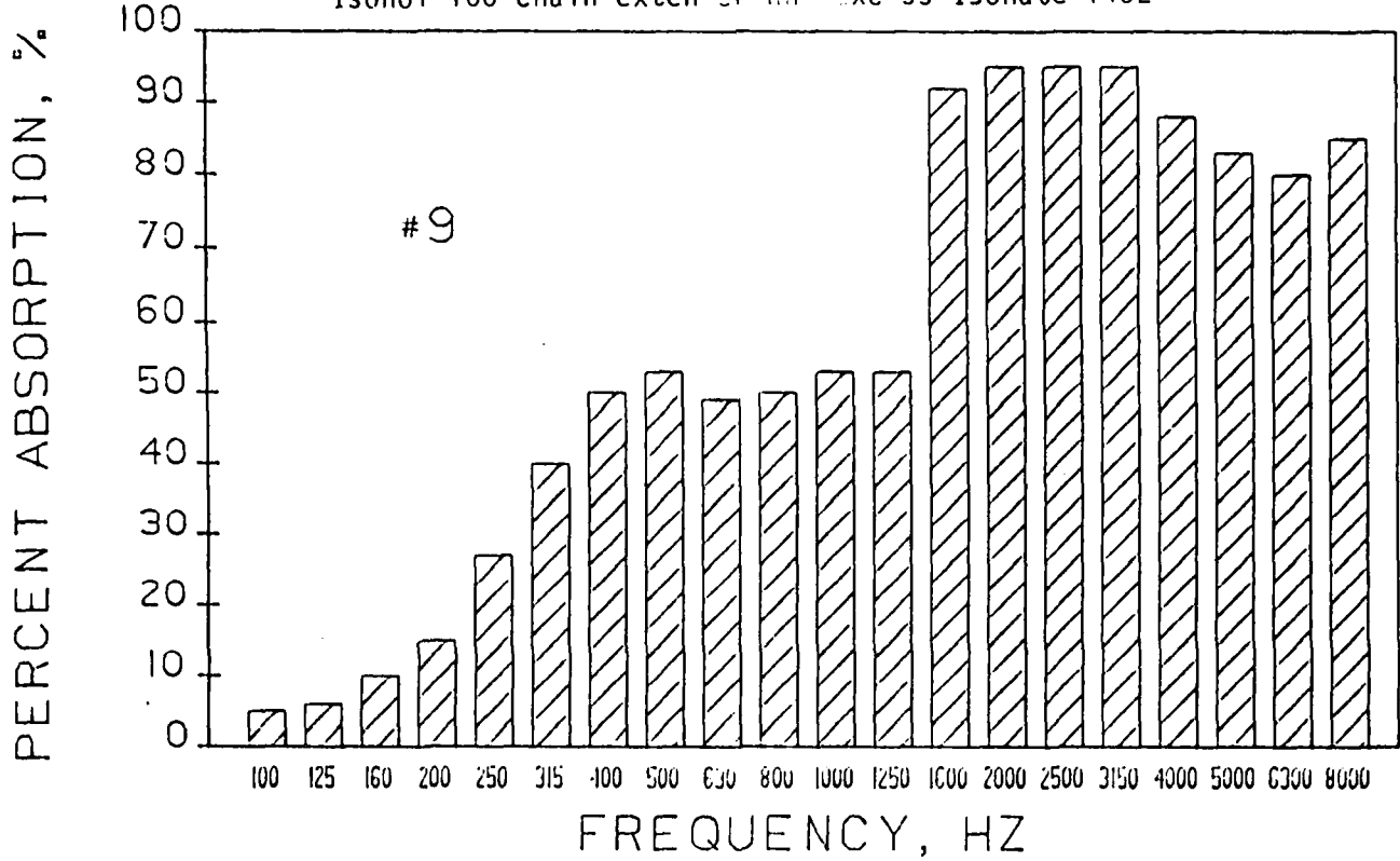
Figure 31. Sound absorption property of 50/50 PU/Epoxy IPN foam excluded Isonol 100 chain extender and excess Isonate 143L
