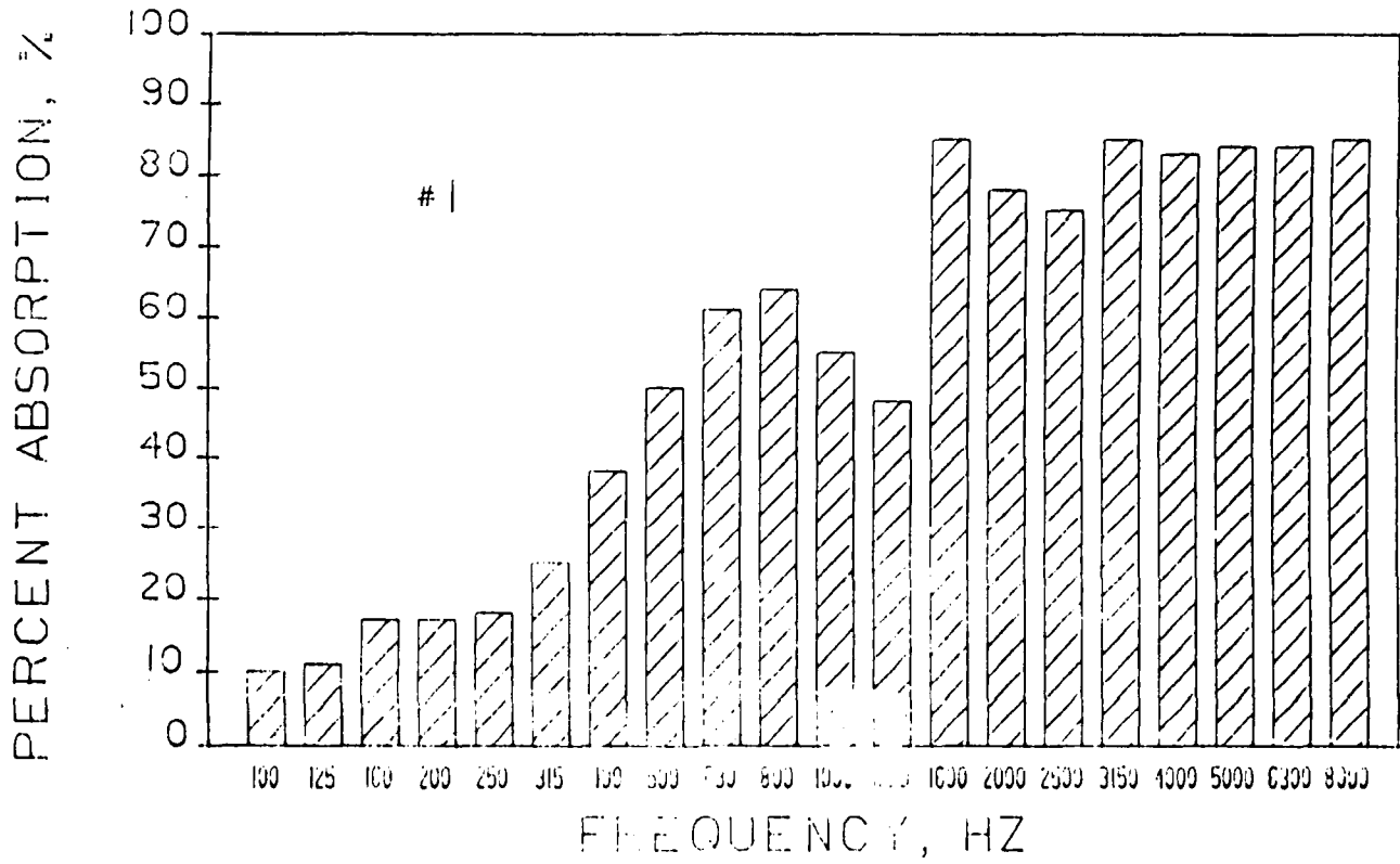
Figure 23. Top portion of 70/30 PU/Epoxy IPN foam
