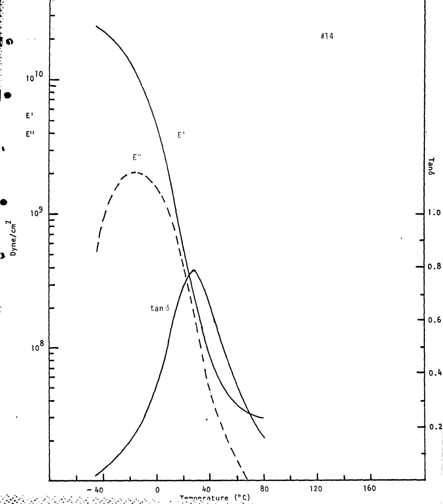
Figure 18. Dynamic mechanical spectroscopy of PU/Epoxy (60/40) IPN after 2 hrs. post curing at 100°C
