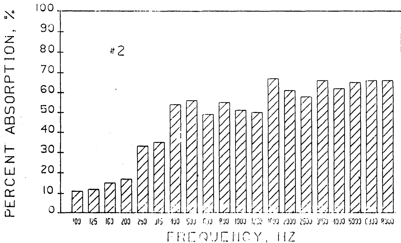
Figure 24. Bottom portion of 70/30 PU/Epoxy IPN foam
