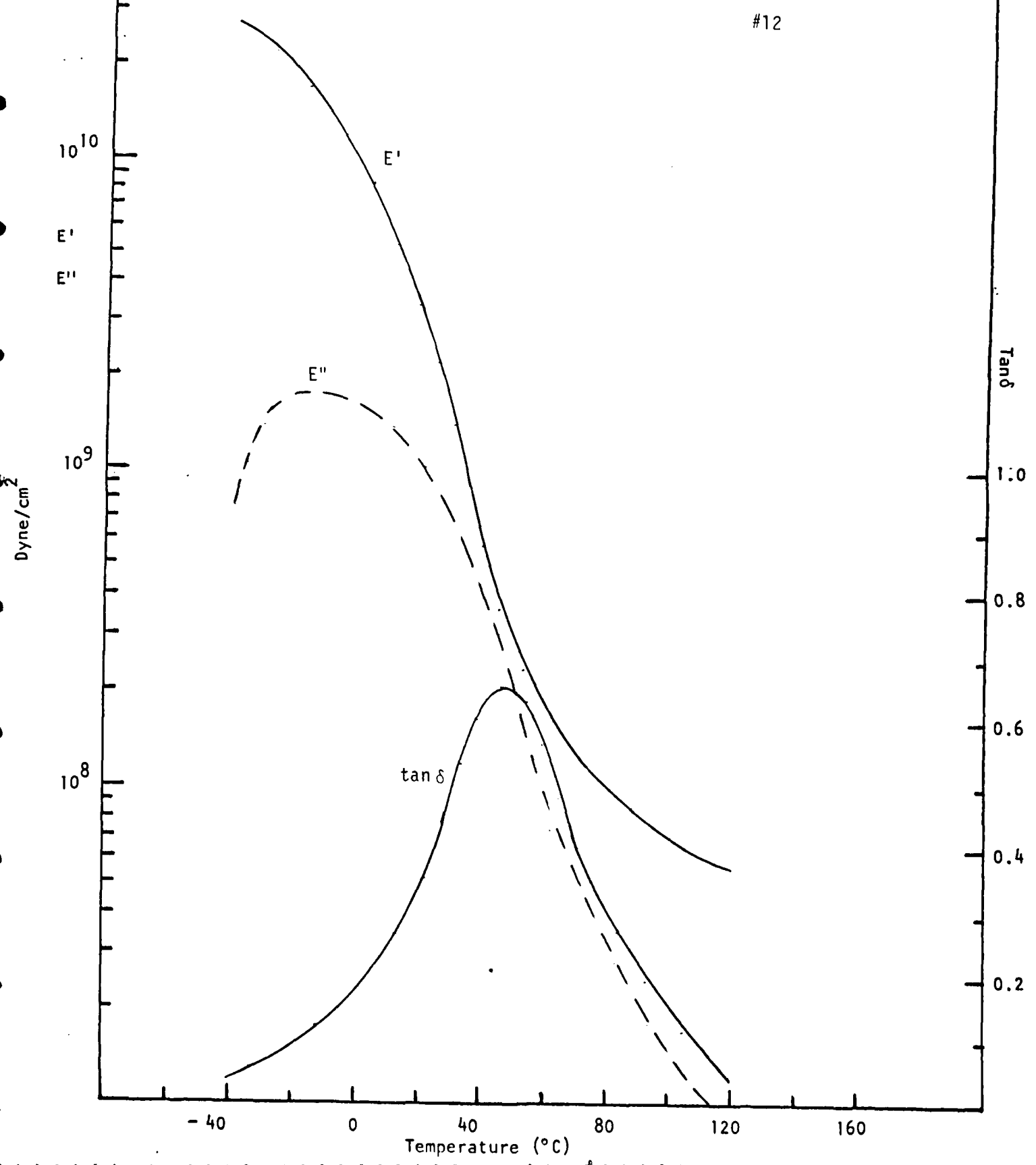
Figure 15. Dynamic mechanical spectroscopy of PU/Epoxy (60/40) IPN with 10% Dicaperl filler
