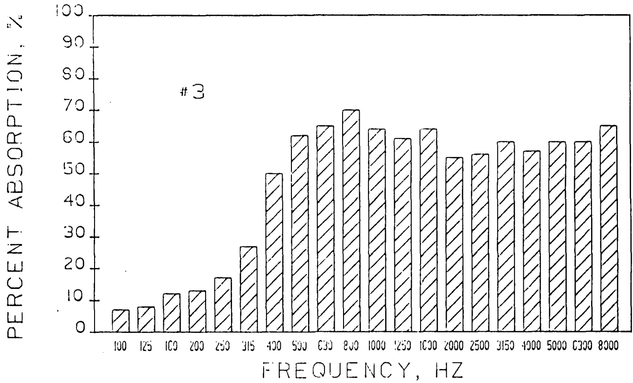
Figure 25. Sound absorption properties of 60/40 PU/Epoxy IPN foam
