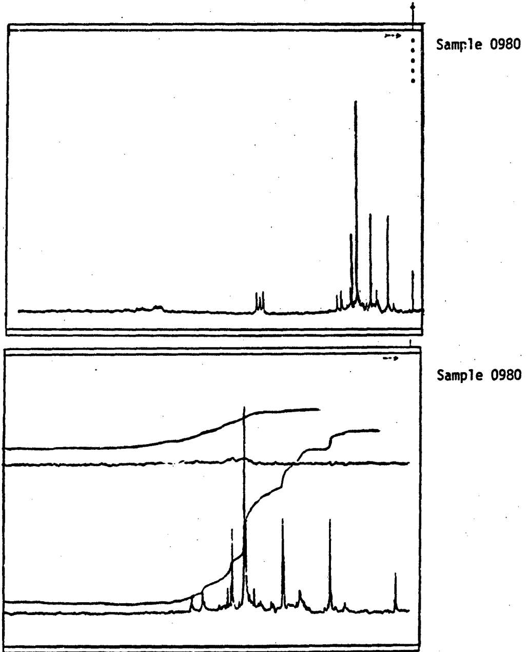
Figure 4. Fuel 83-POSF-0980 ^{13}\text{C} spectra.
