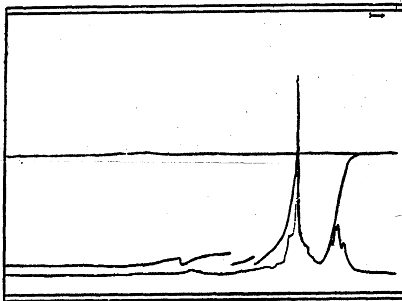
Figure 5. Fuel 83-POSF-0980 1 H spectra.
