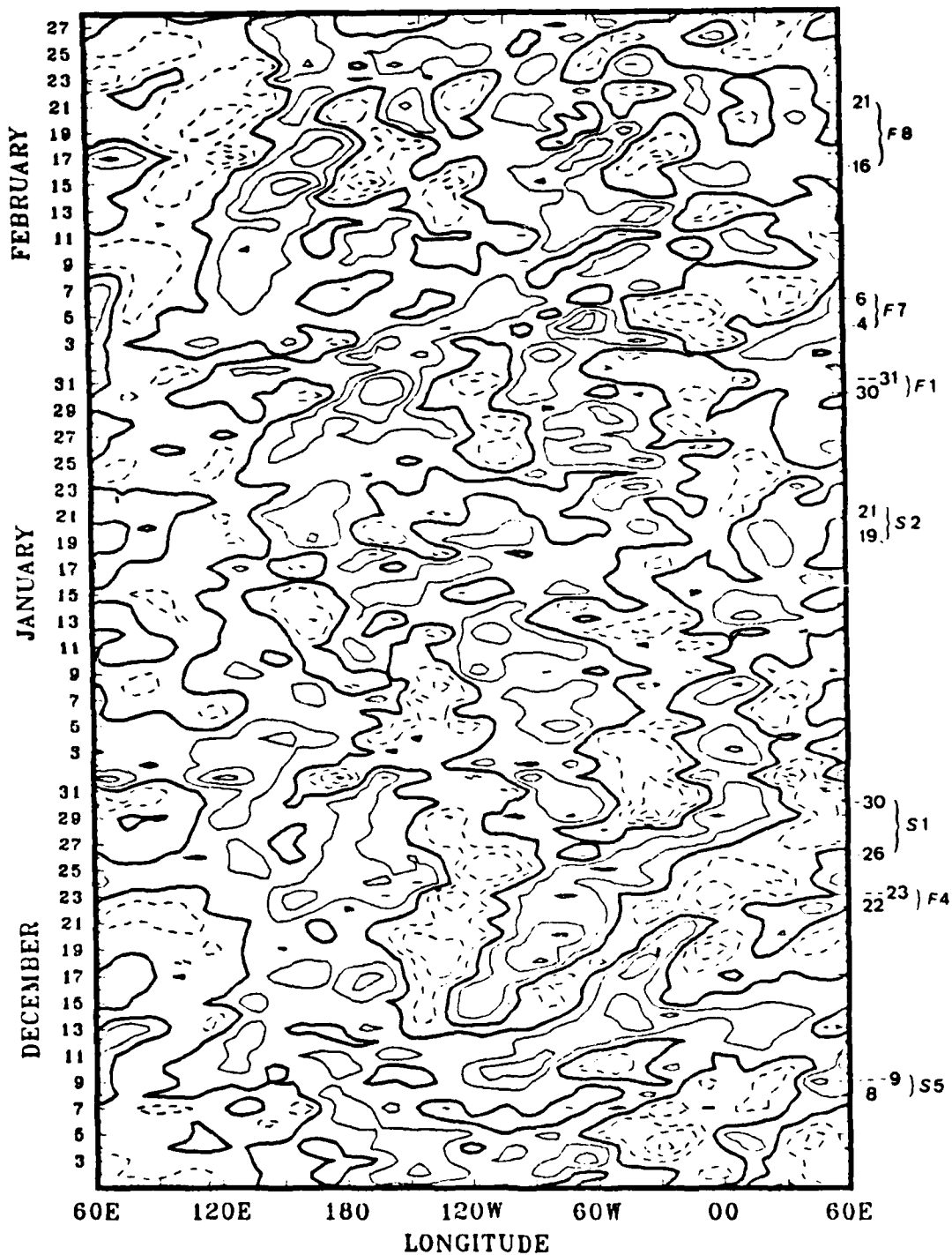
Fig. A.12 Winter 1983-84 day-five error patterns (average five-day forecast 500 mb heights minus average verifying day an heights).
