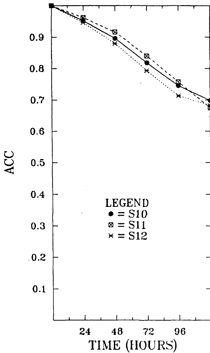
Fig. A.5 ACC versus forecast day for winter 1984-85 STARH periods. Each ACC value plotted represents an average value for the period.
