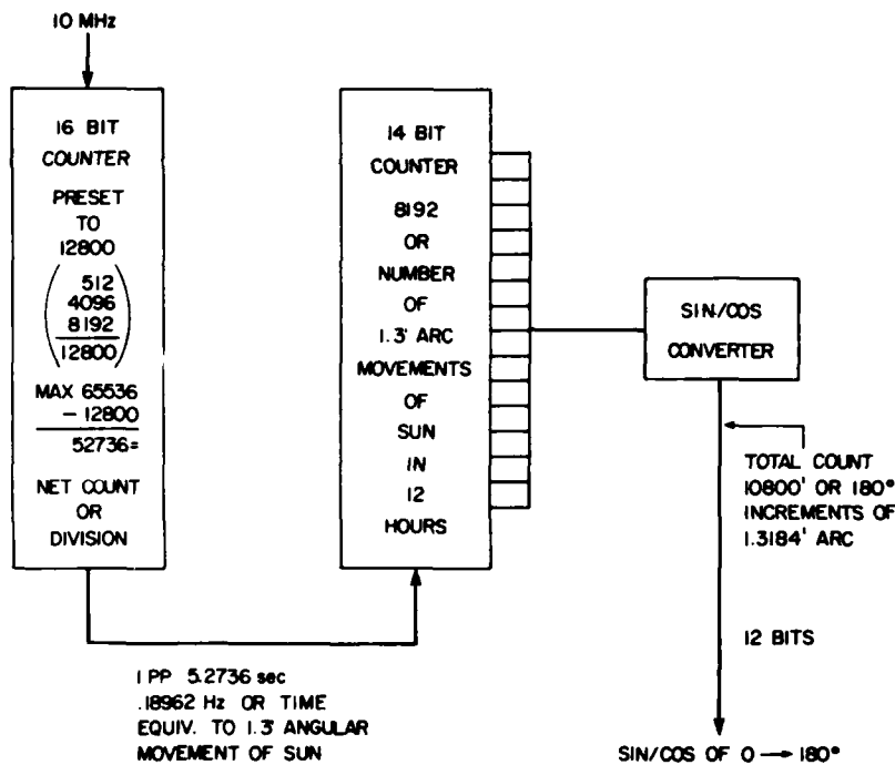
Figure 3. Time Base Generator, 10 MHz Divided by 52736 = 0.18962 Hz
