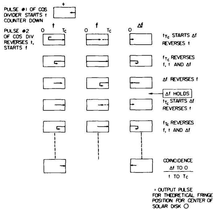
Figure 6. Logic of Fringe Position Detector
