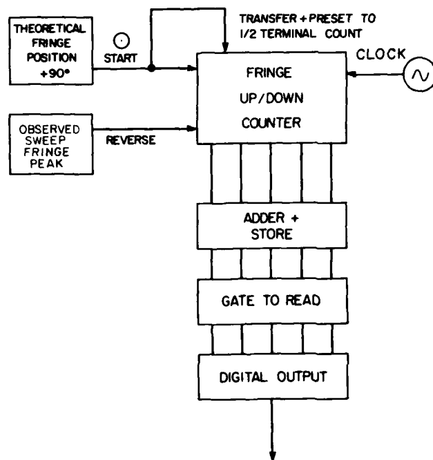
Figure 7. Fringe Read Out
