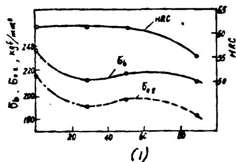
Fig. 2 The percentage of bainite vs strength and toughness. (treated by carbide refining techniques II a , II b , II c , and II d ) (1: percentage of bainite)
