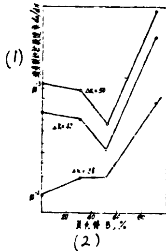
Fig.5 The percentage of bainite vs the growth rate of fatigue cracks (da/dN) at various \Delta K . ( 1: growth rate of fatigue cracks; 2: percentage of bainite)
