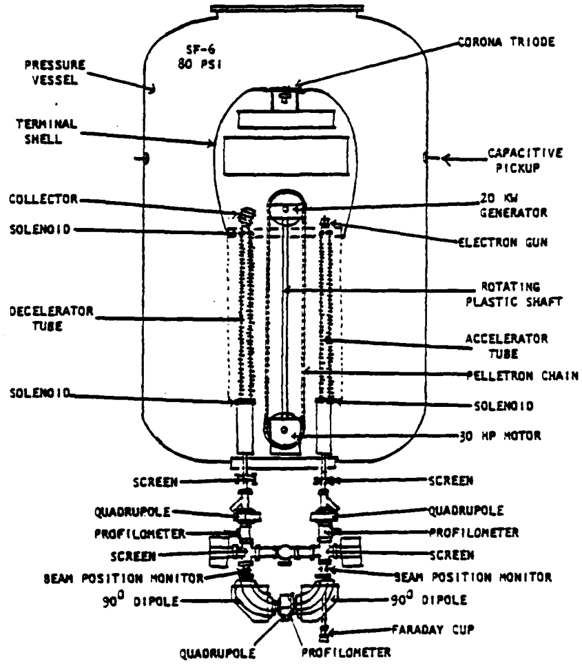
Figure 1. Experimental Set-up.
