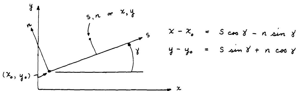
Figure 4. Coordinate Relations
