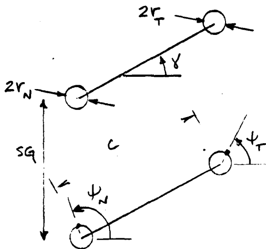
FIGURE 5 NOTATION FOR FLAT-PLATE CASCADE
