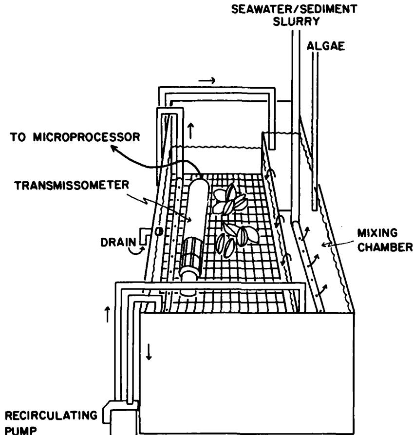
Figure 6. Blue mussel ( Mytilus edulis ) contaminant uptake system
