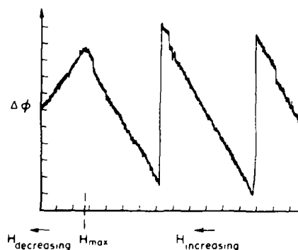
FIG. 2. Strip-chart record of changing flux (on the vertical scale) as a function of external field (on the horizontal scale) showing three Barkhausen jumps near the peak field on run no. 13. The jumps are equivalent to magnetic-moment changes of \sim 10^{-7} emu in the iron pill sample. The field was ramped at 0.897 mOe/sec. The two full-scale vertical lines are due to manual resets. The peak field, seen near the left end of the figure, was 299 mOe.
