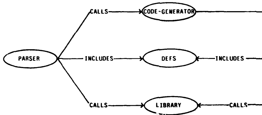
Figure 1-1: TINYCOMP Inter-Module Reference Graph
