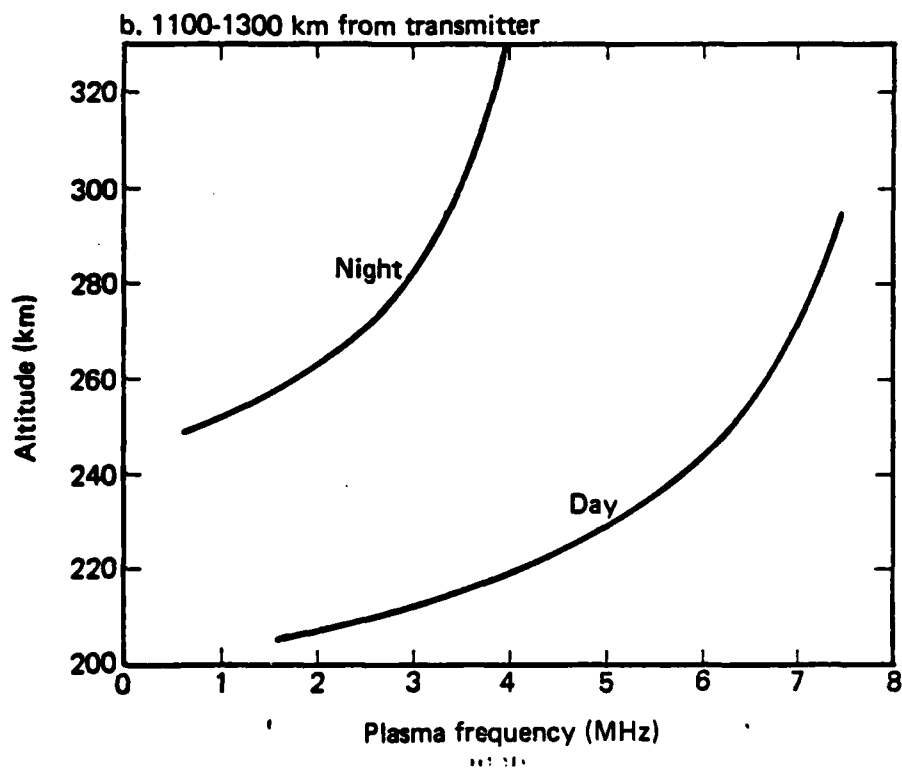
Figure 2. Ionosphere profiles for calculation of electric fields.
