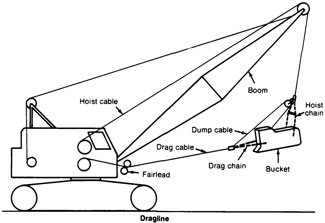
Figure A-1. Equipment schematic of a typical clamshell and dragline.
