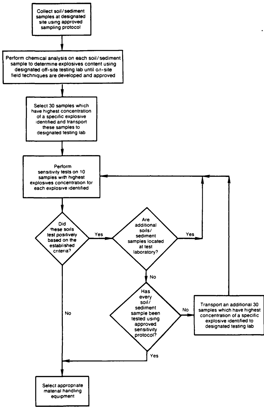
Figure 4. Sensitivity testing protocol.
