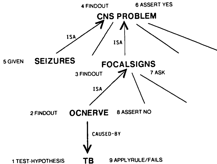
Figure 6-1: Backward deduction in NEOMYCIN to confirm a solution
